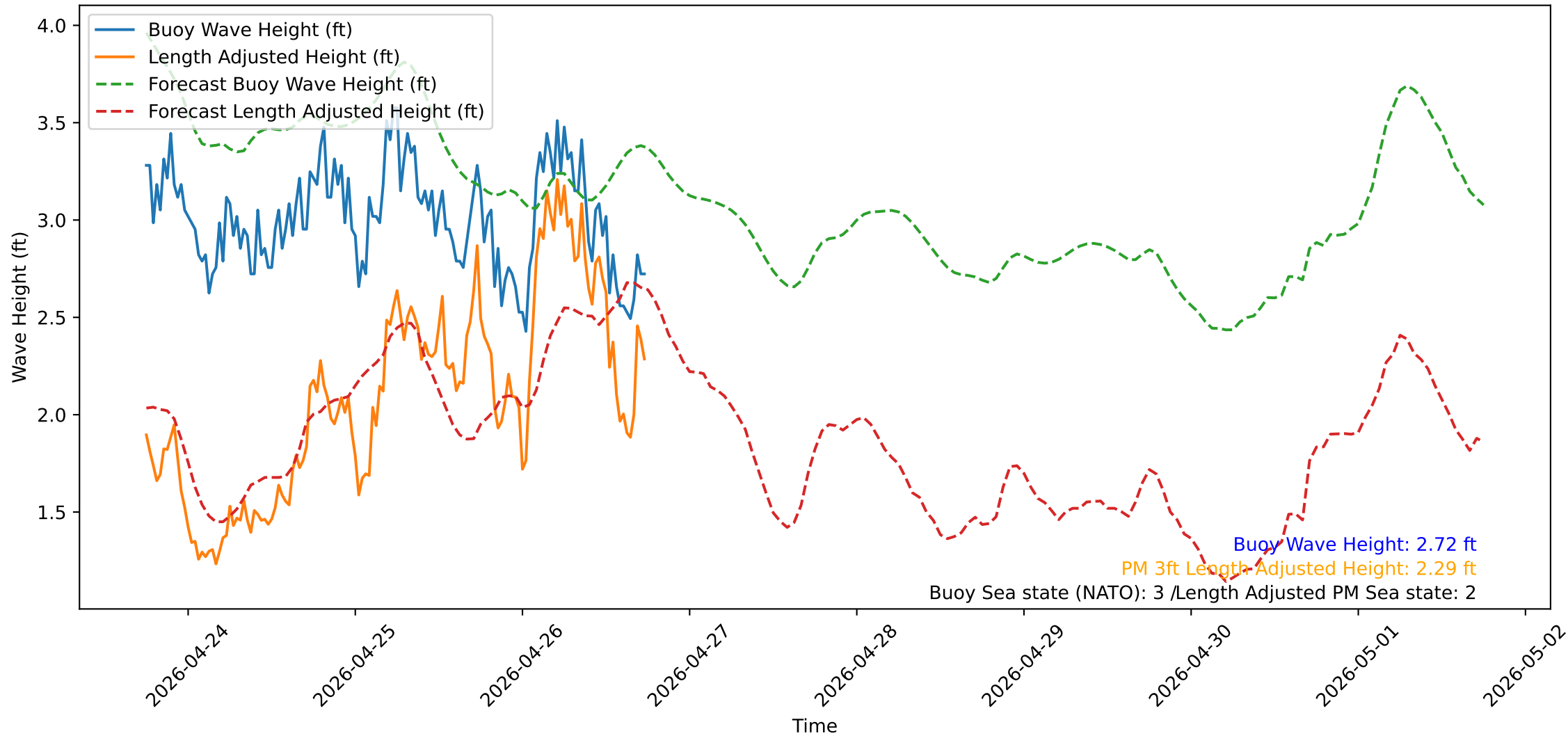
Wave Heights over Time for Green Beach at 2026-04-26 18:11:13
