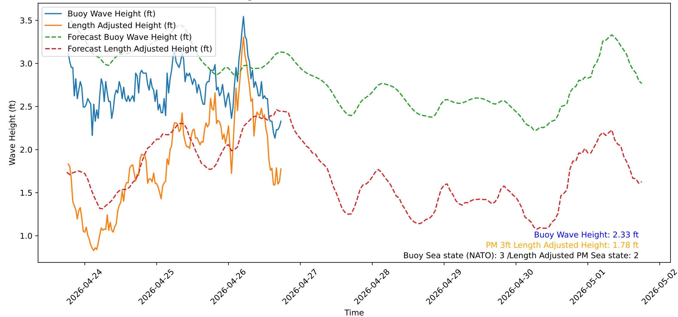
Wave Heights over Time for Red Beach at 2026-04-26 18:10:50
