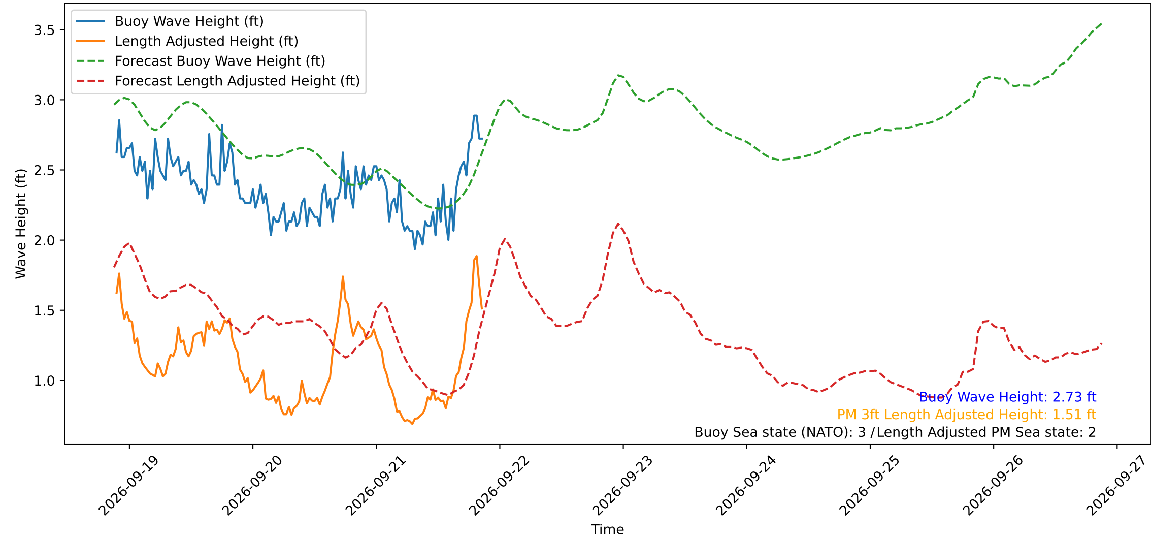
Wave Heights over Time for Red Beach at 2026-09-21 21:20:50
