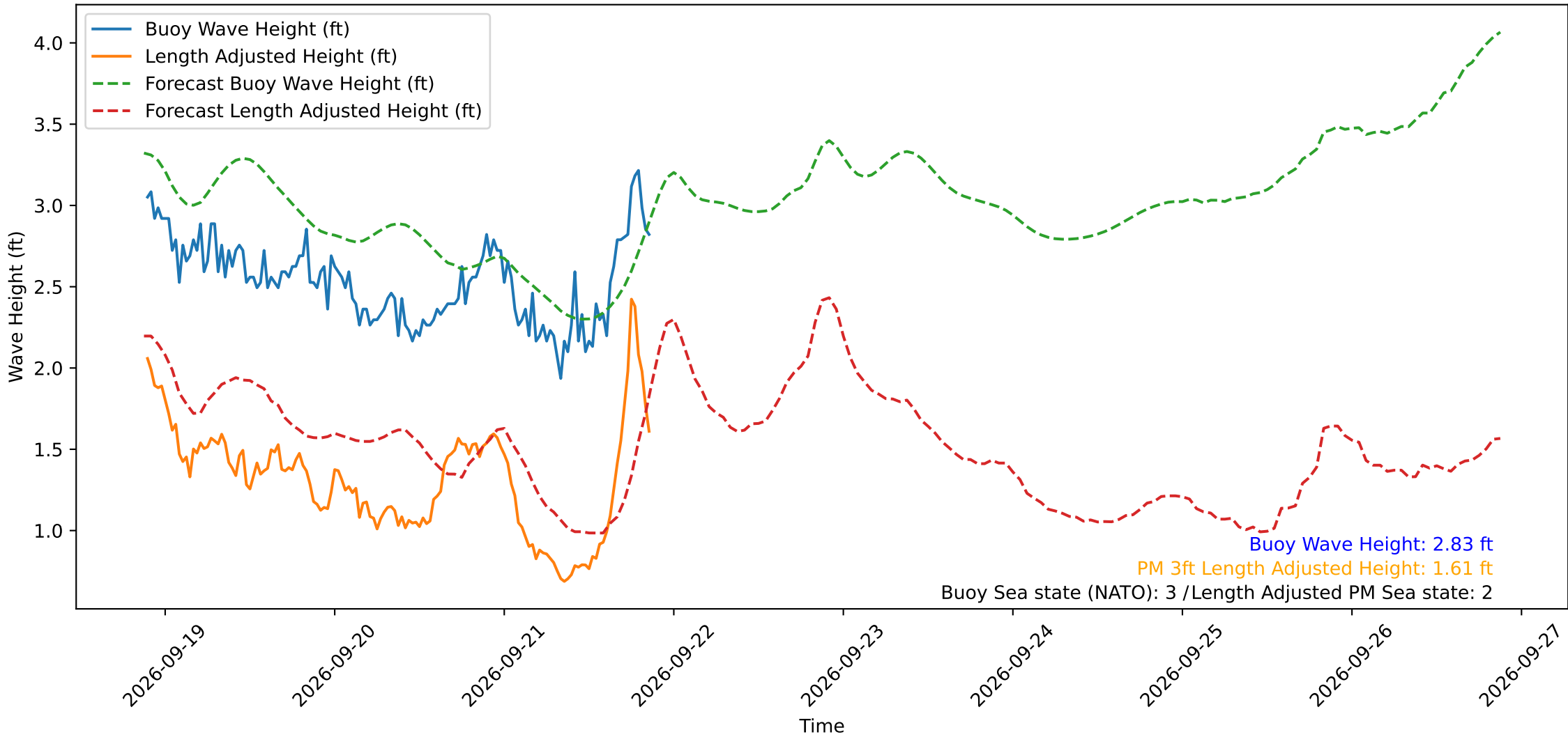
Wave Heights over Time for Green Beach at 2026-09-21 21:21:13
