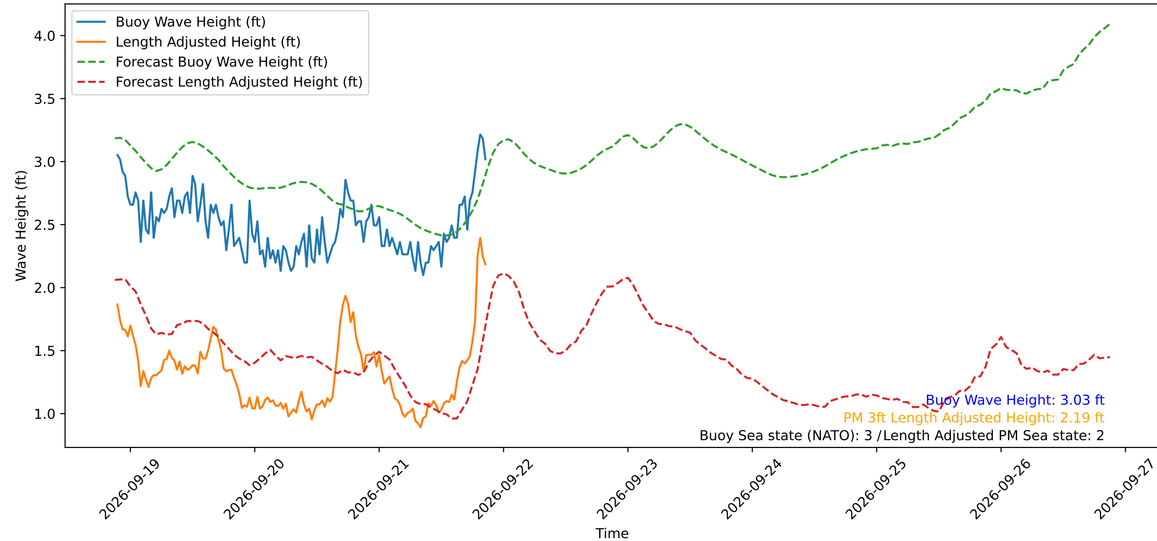
Wave Heights over Time for Oceanside Harbor at 2026-09-21 21:20:29
