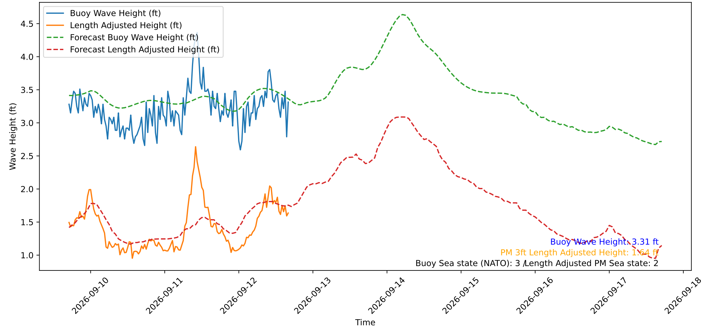
Wave Heights over Time for Oceanside Harbor at 2026-09-12 16:50:29
