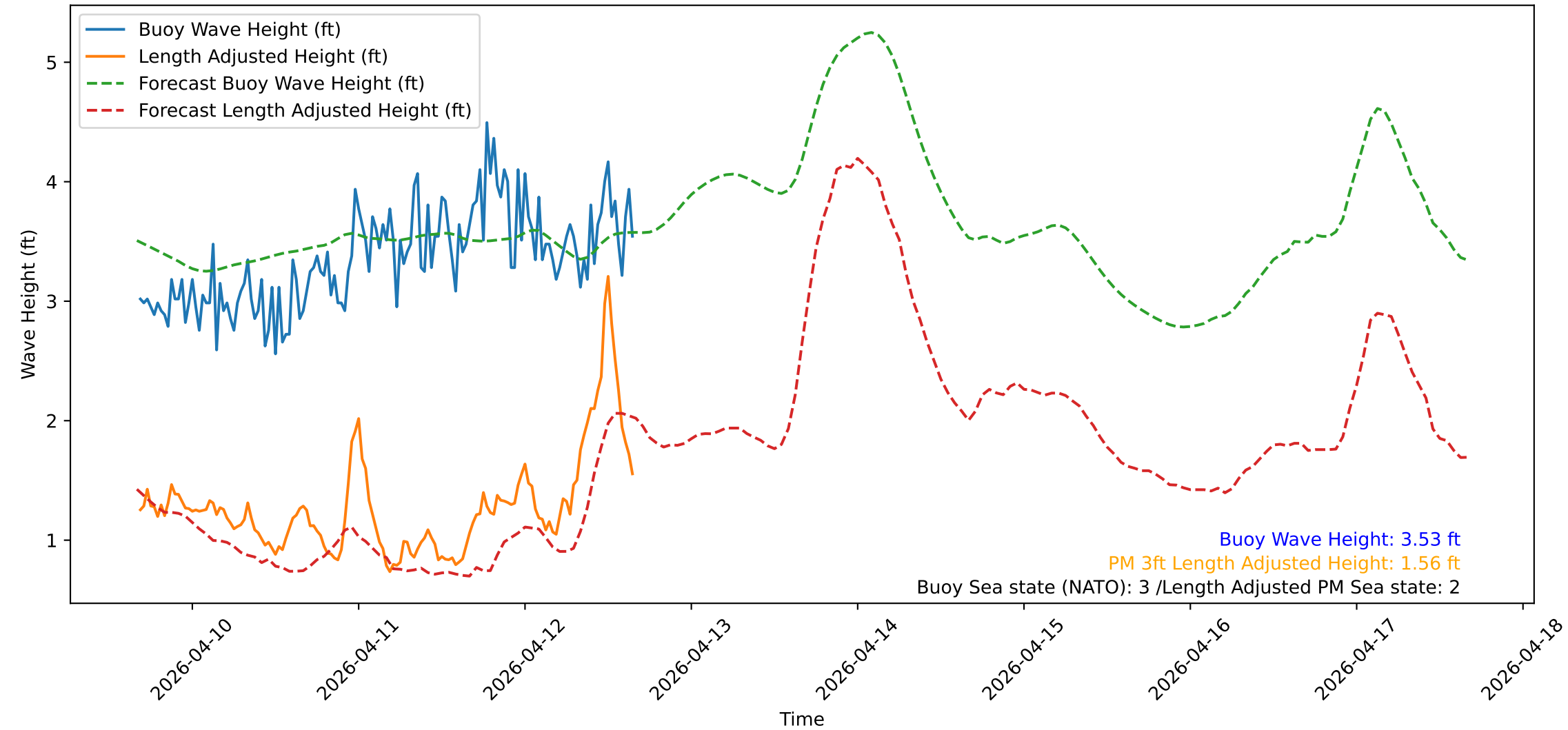
Wave Heights over Time for Green Beach at 2026-04-12 16:21:14
