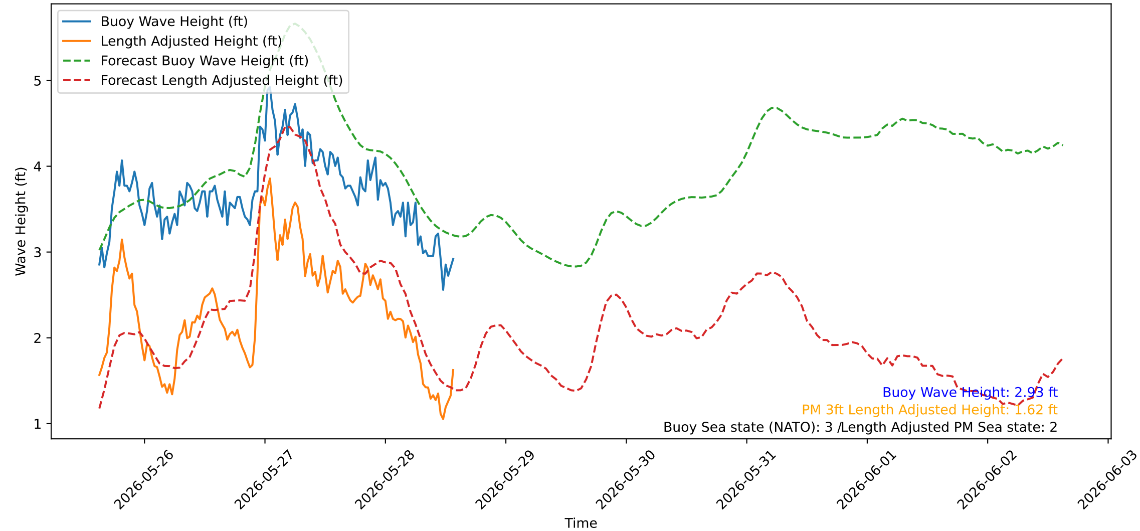
Wave Heights over Time for Green Beach at 2026-05-28 15:01:00
