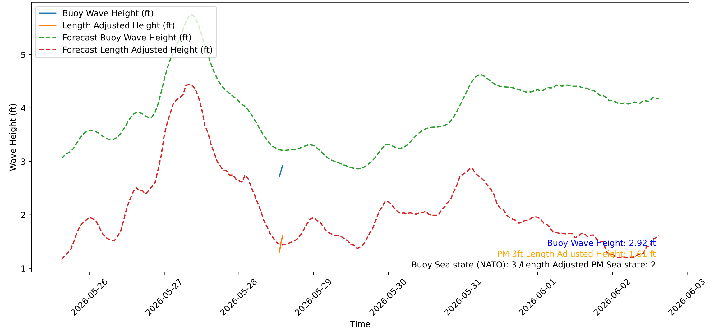
Wave Heights over Time for Oceanside Harbor at 2026-05-28 15:00:19
