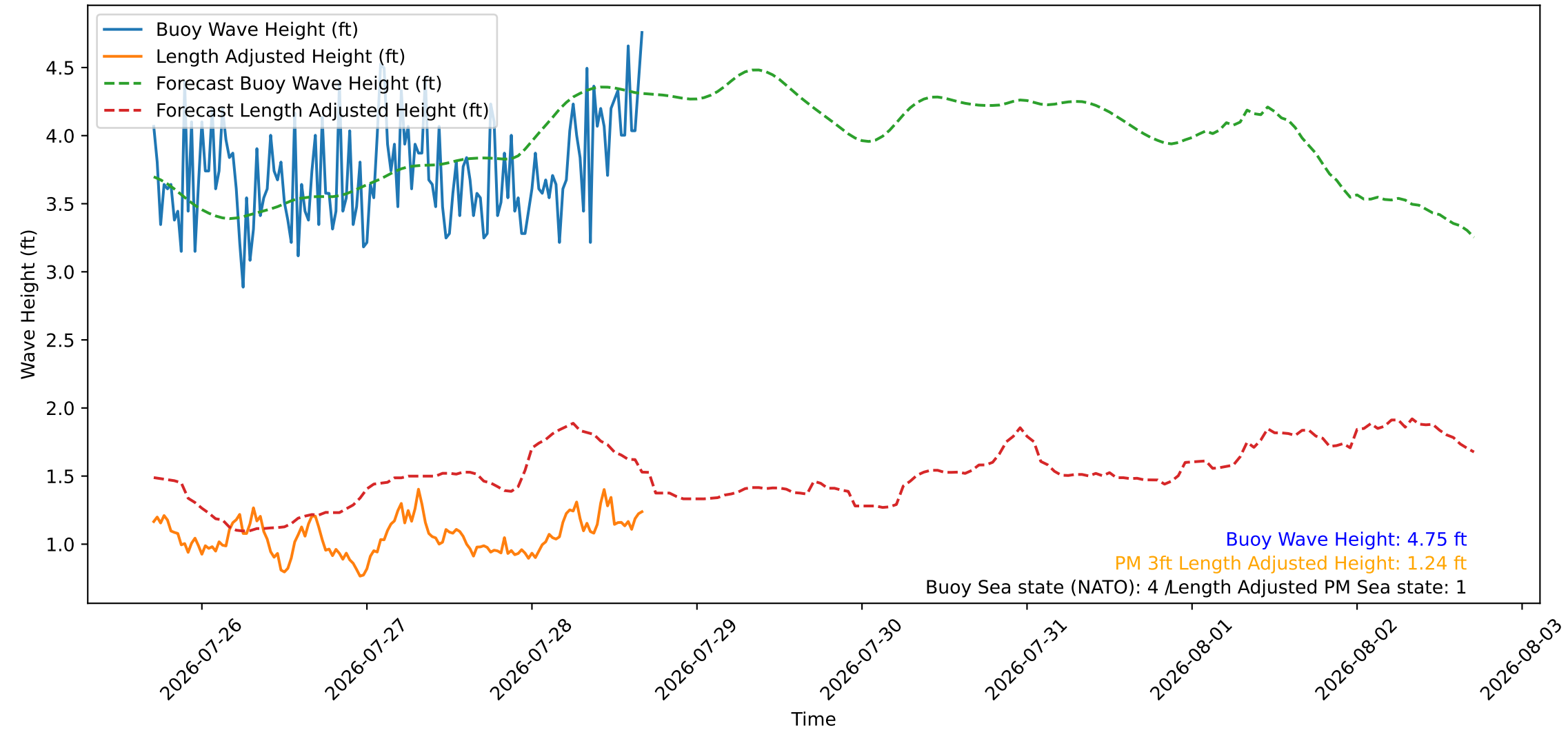
Wave Heights over Time for Red Beach at 2026-07-28 16:40:46
