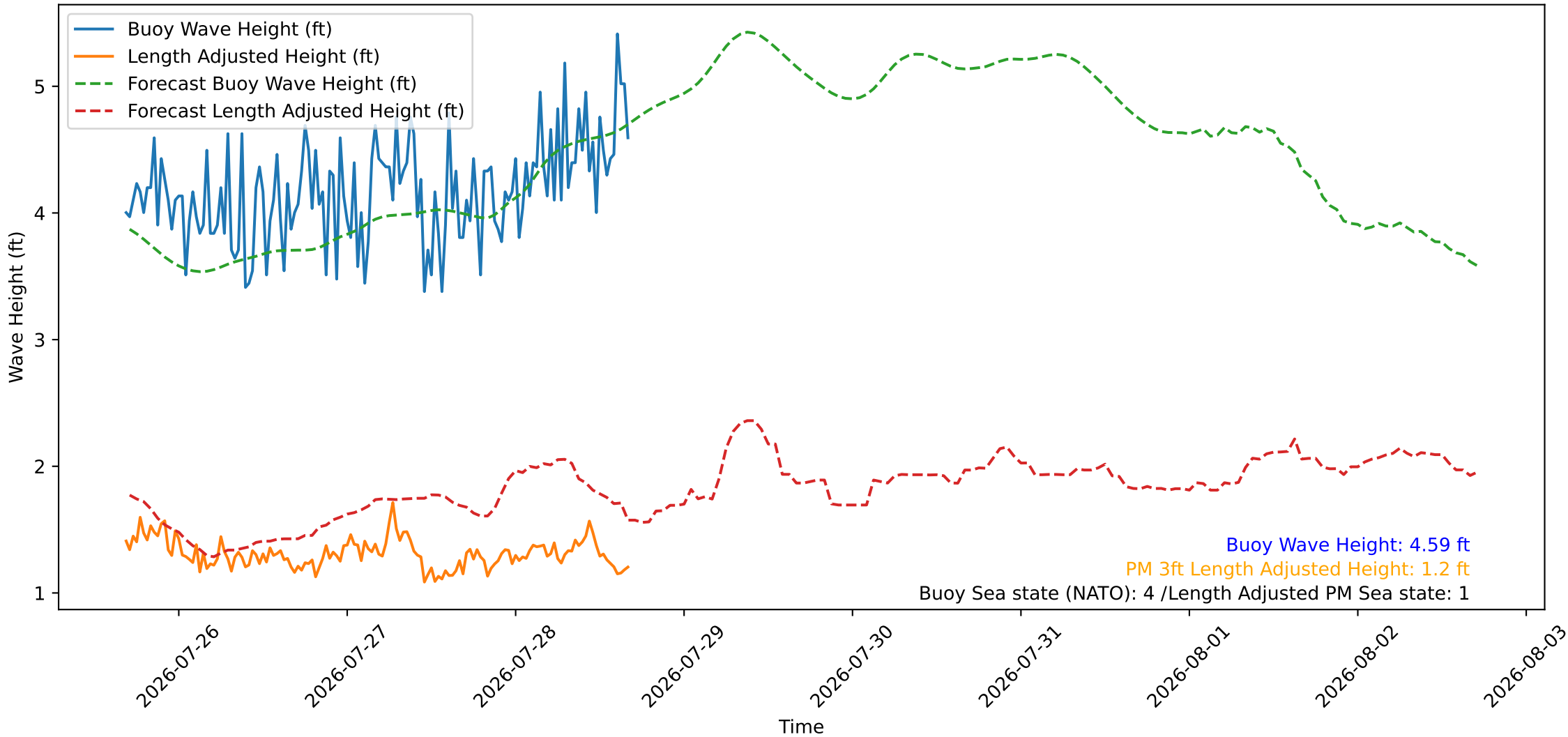
Wave Heights over Time for Green Beach at 2026-07-28 16:41:09
