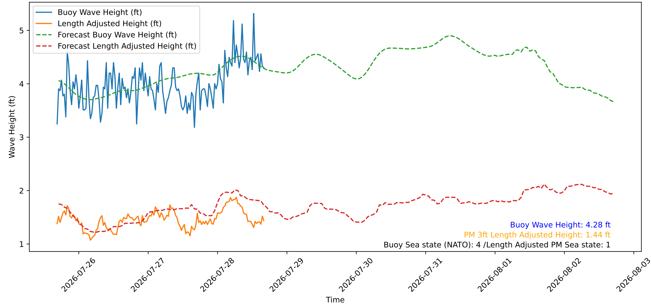
Wave Heights over Time for Oceanside Harbor at 2026-07-28 16:40:27
