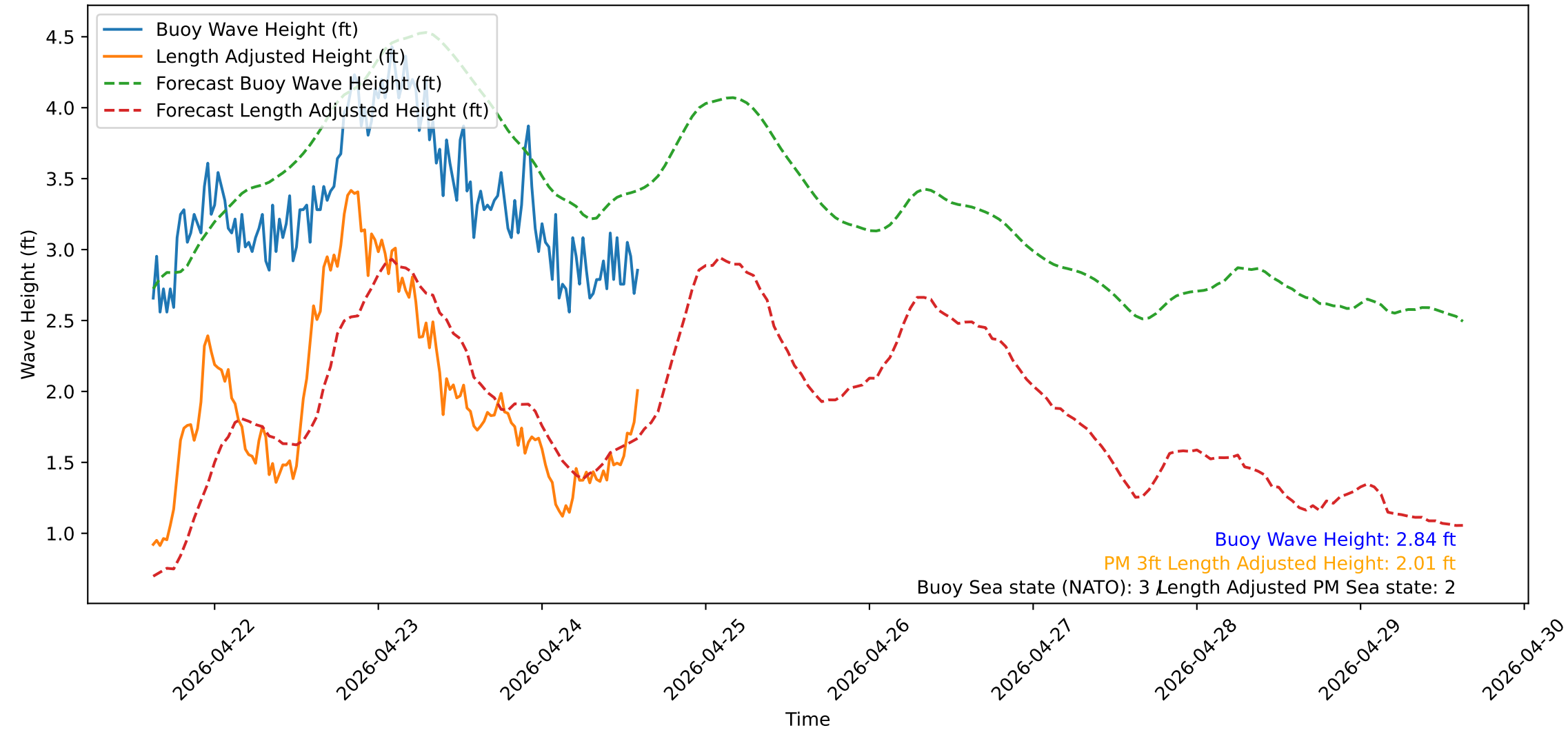
Wave Heights over Time for Oceanside Harbor at 2026-04-24 15:00:32
