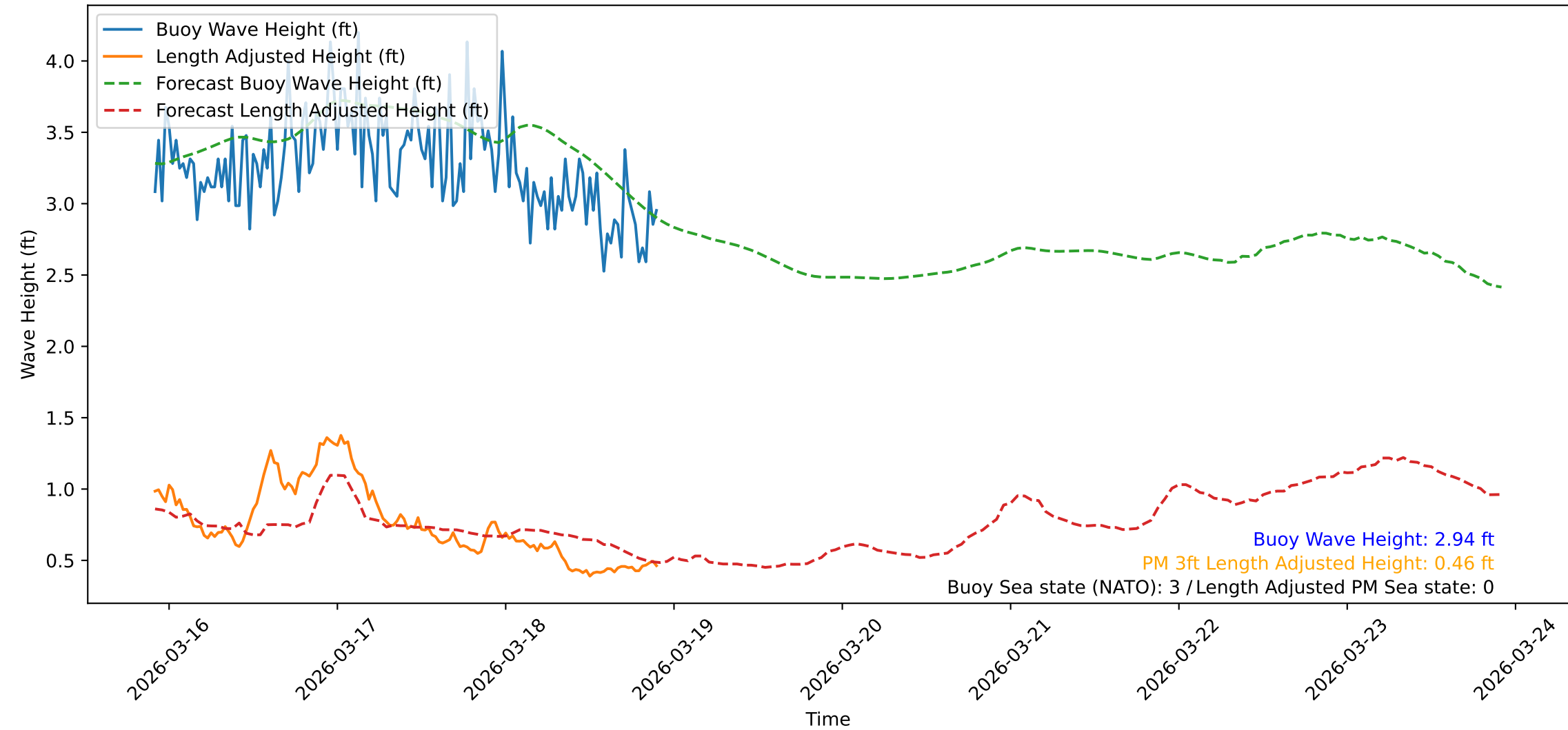
Wave Heights over Time for Green Beach at 2026-03-18 22:11:10
