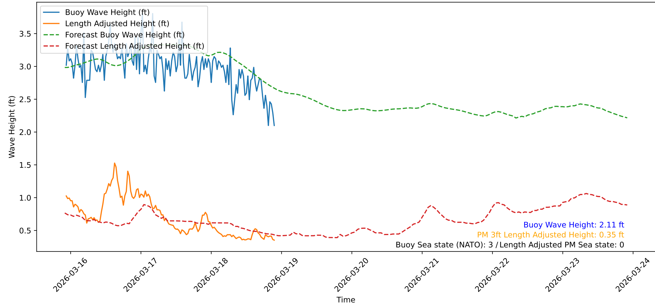
Wave Heights over Time for Red Beach at 2026-03-18 22:10:47
