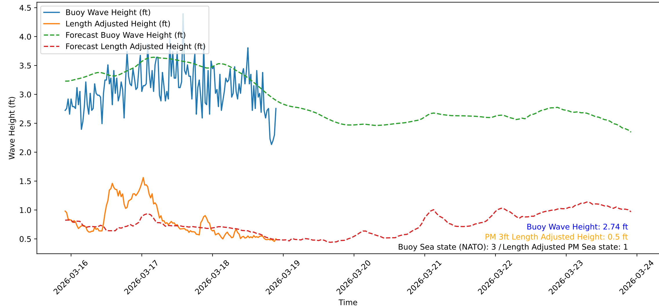
Wave Heights over Time for Oceanside Harbor at 2026-03-18 22:10:31
