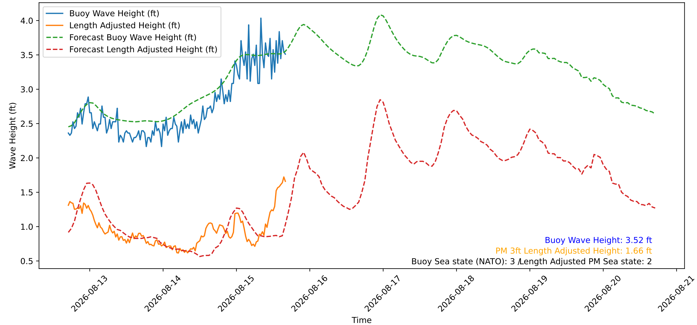
Wave Heights over Time for Red Beach at 2026-08-15 16:40:46
