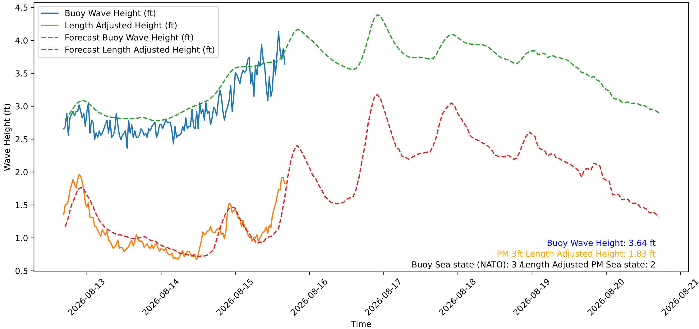
Wave Heights over Time for Green Beach at 2026-08-15 16:41:08
