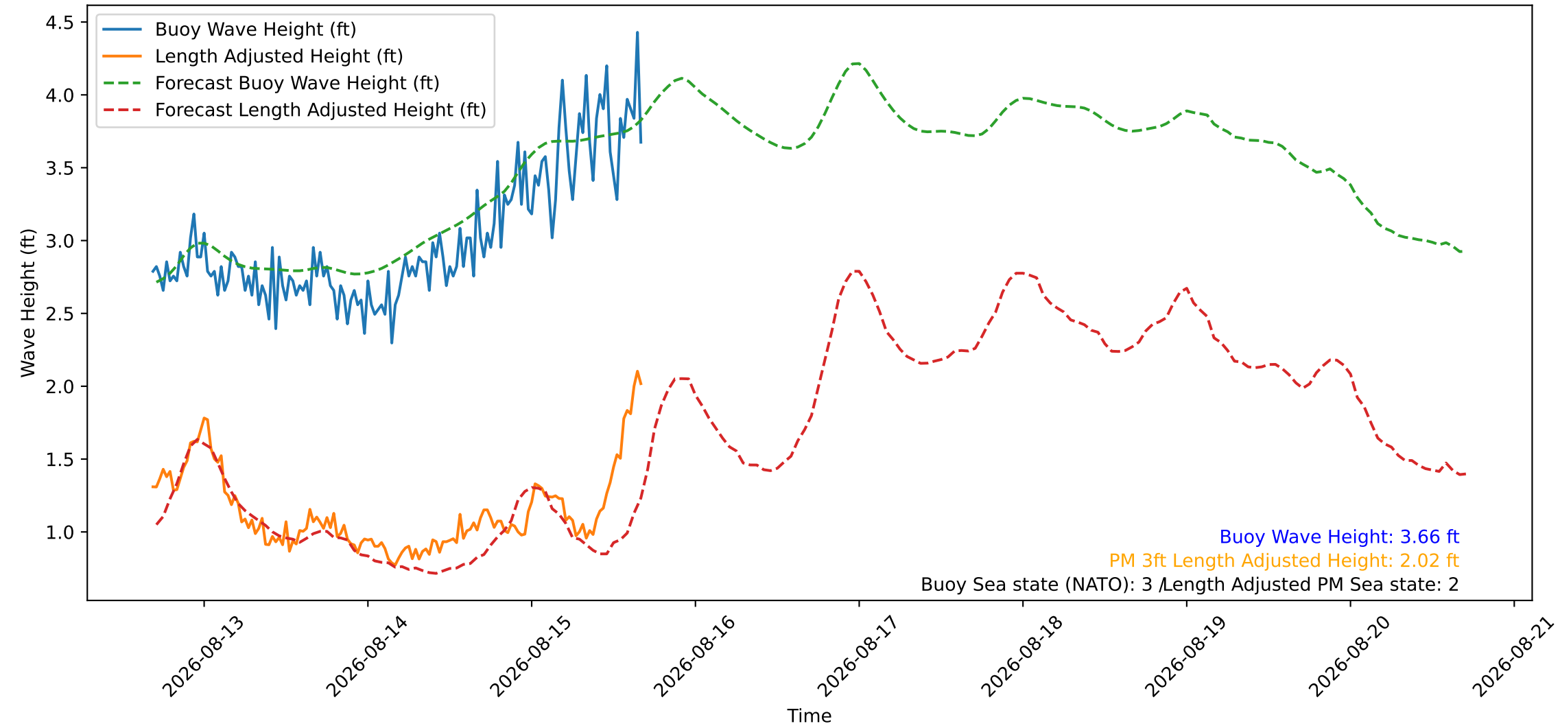
Wave Heights over Time for Oceanside Harbor at 2026-08-15 16:40:26
