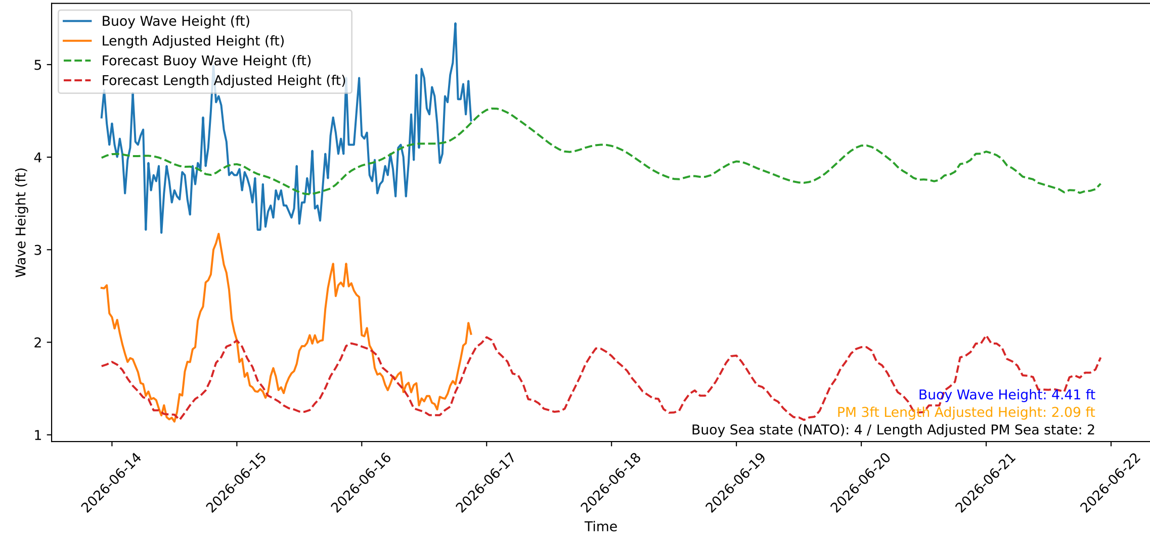
Wave Heights over Time for Oceanside Harbor at 2026-06-16 22:00:26
