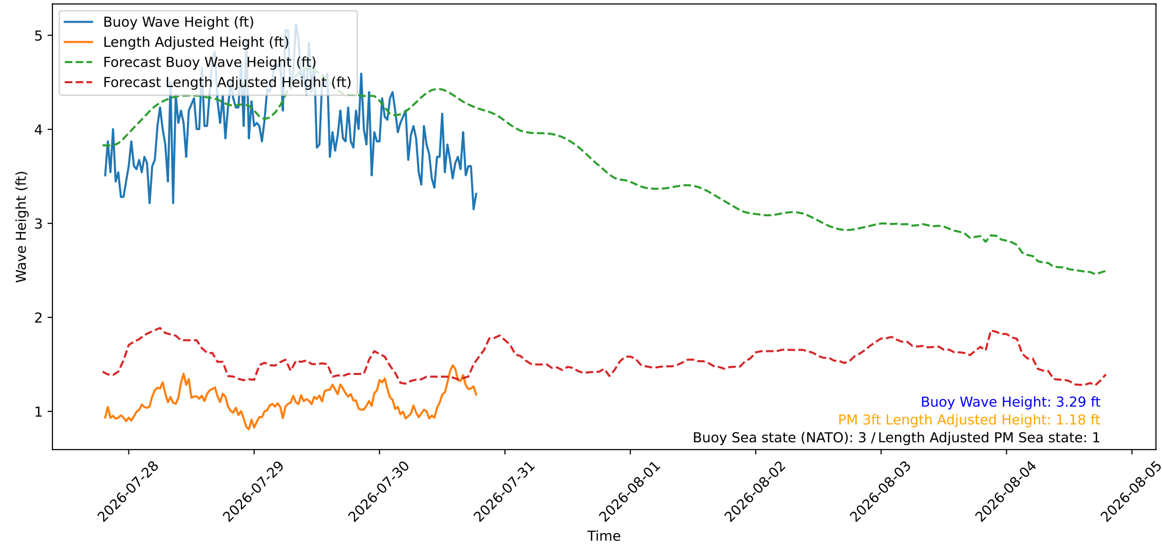
Wave Heights over Time for Red Beach at 2026-07-30 19:20:47
