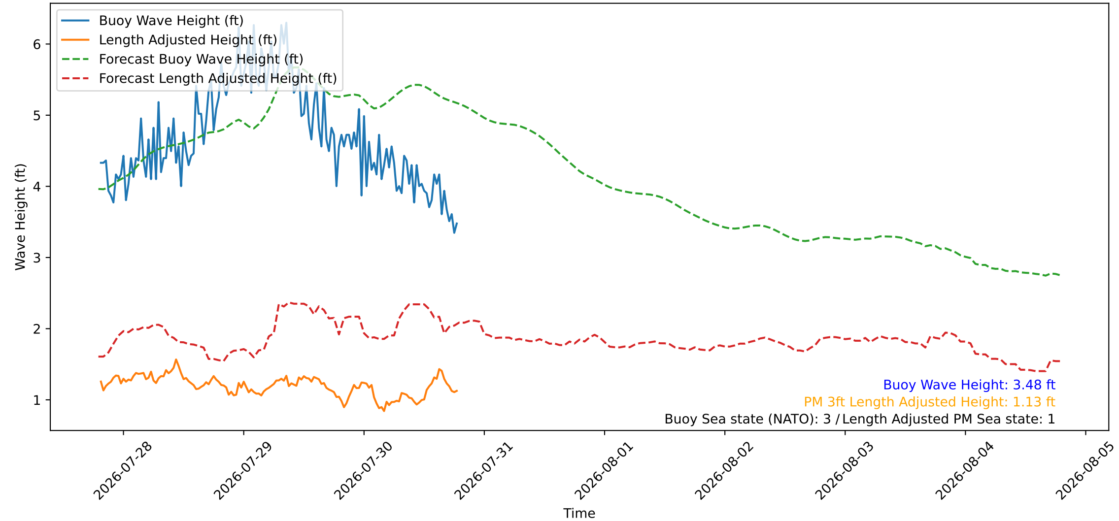
Wave Heights over Time for Green Beach at 2026-07-30 19:21:10
