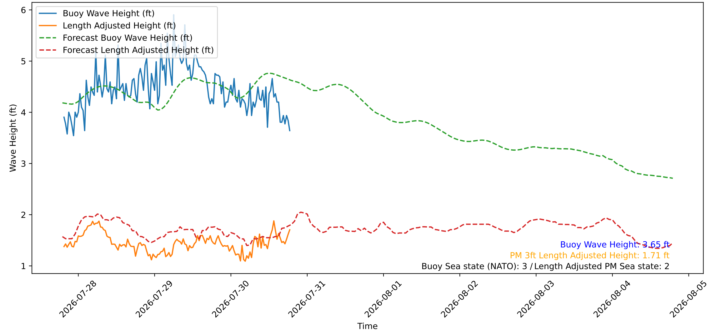
Wave Heights over Time for Oceanside Harbor at 2026-07-30 19:20:26
