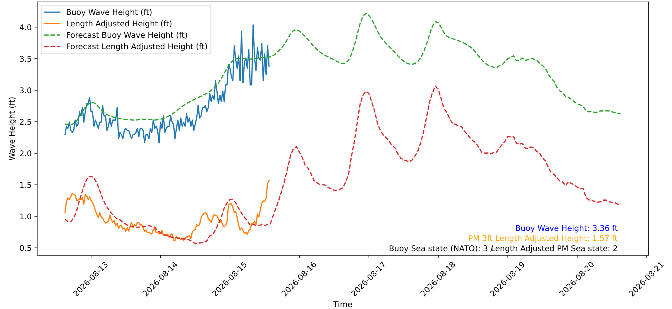
Wave Heights over Time for Red Beach at 2026-08-15 14:30:46
