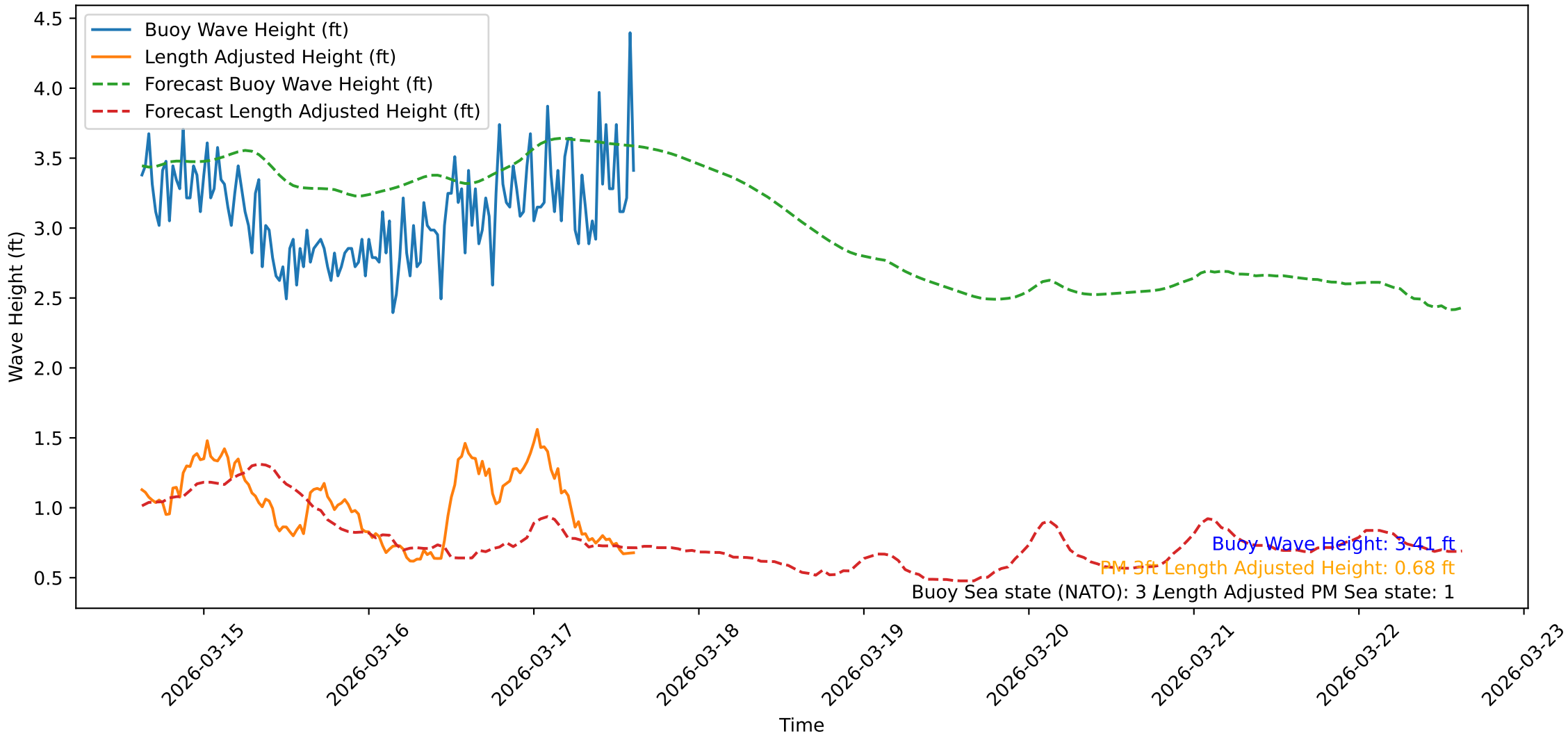
Wave Heights over Time for Oceanside Harbor at 2026-03-17 15:11:02
