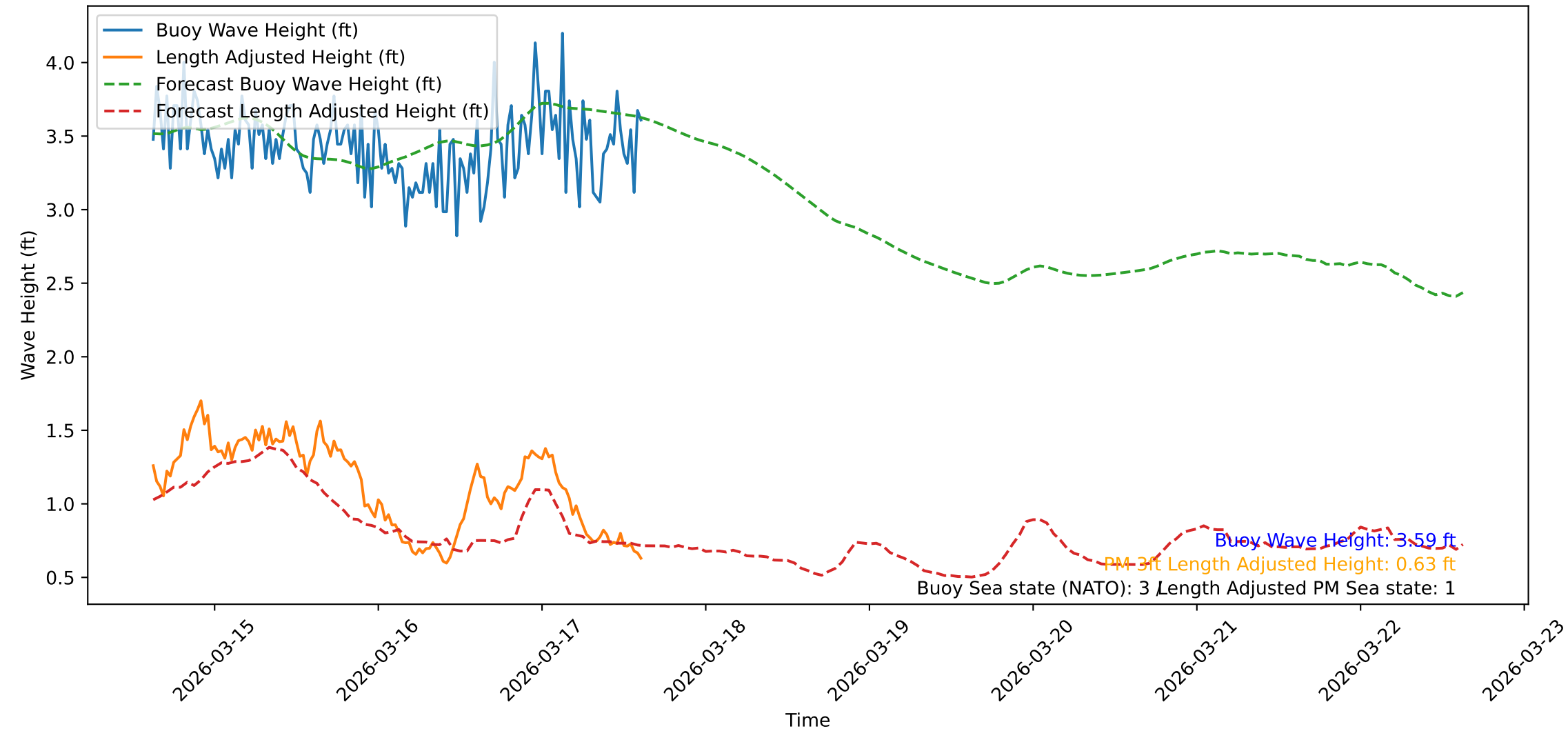
Wave Heights over Time for Green Beach at 2026-03-17 15:12:08
