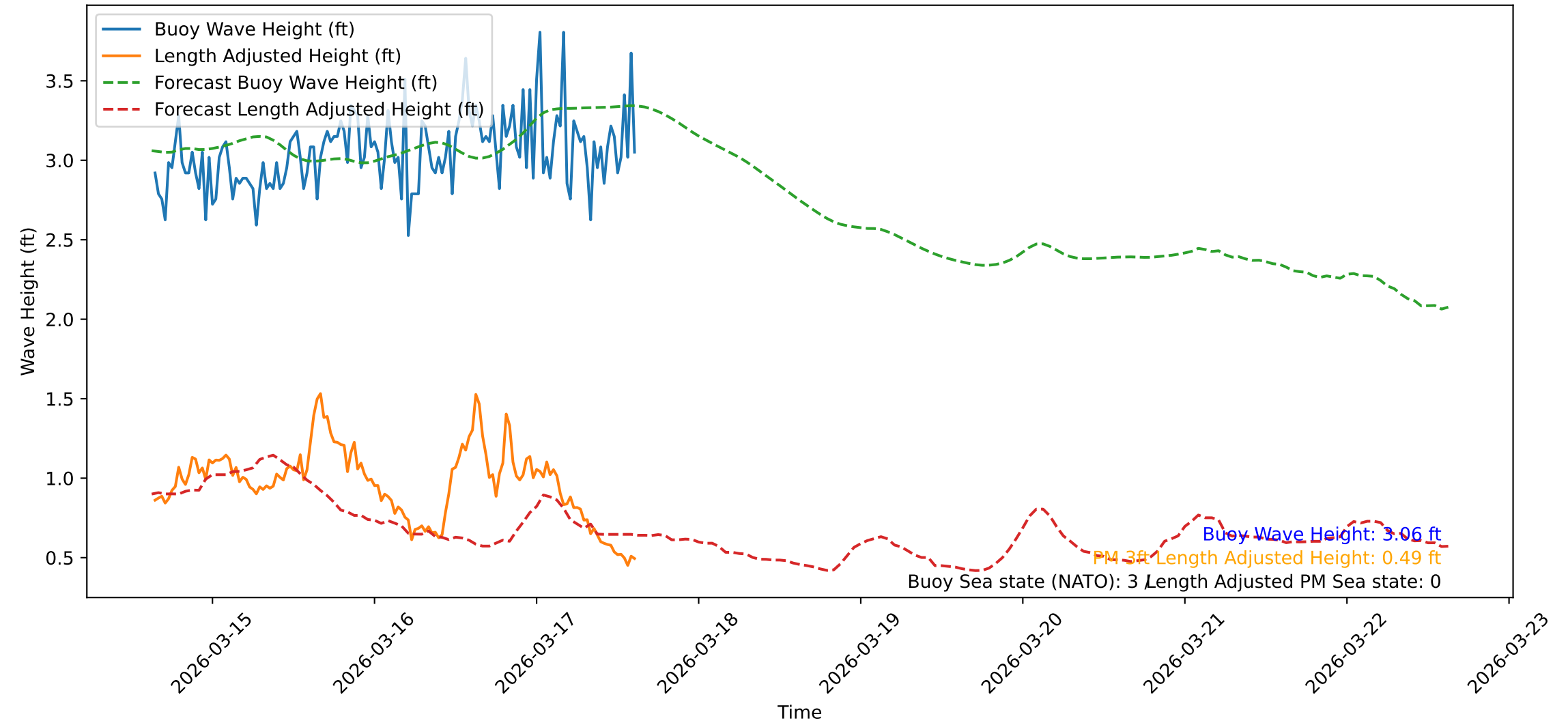
Wave Heights over Time for Red Beach at 2026-03-17 15:11:24
