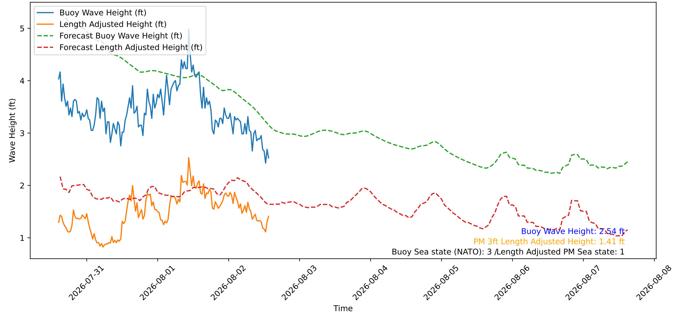
Wave Heights over Time for Green Beach at 2026-08-02 14:31:08
