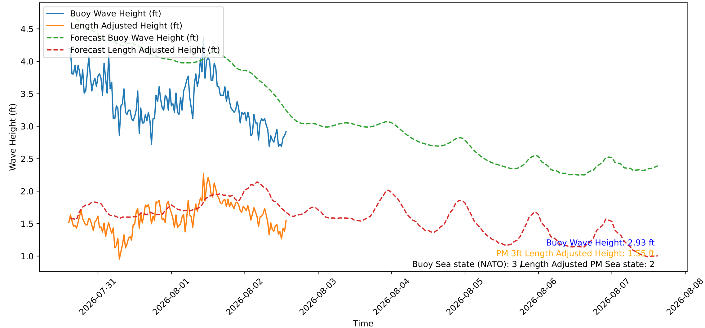
Wave Heights over Time for Oceanside Harbor at 2026-08-02 14:30:27
