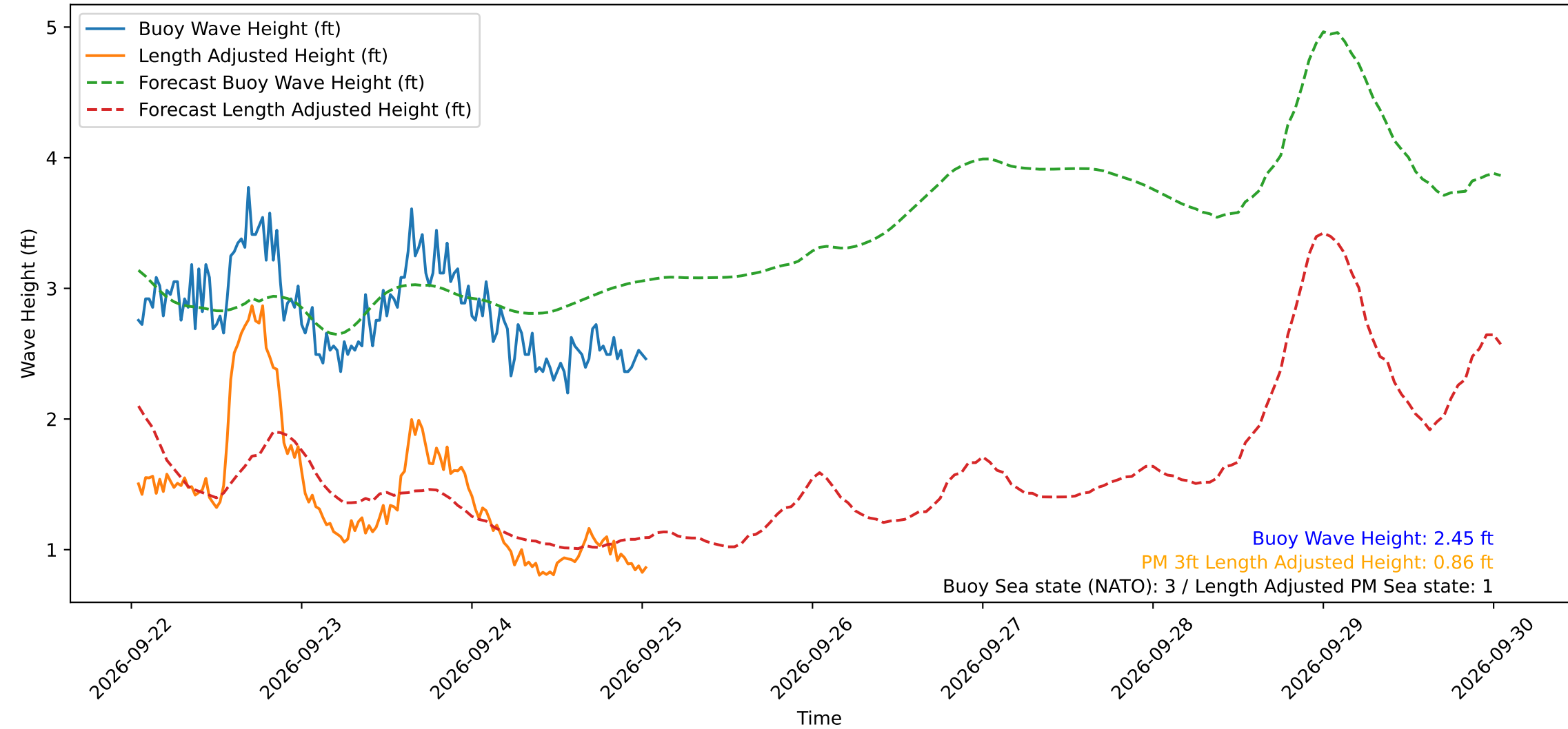
Wave Heights over Time for Oceanside Harbor at 2026-09-25 01:10:30
