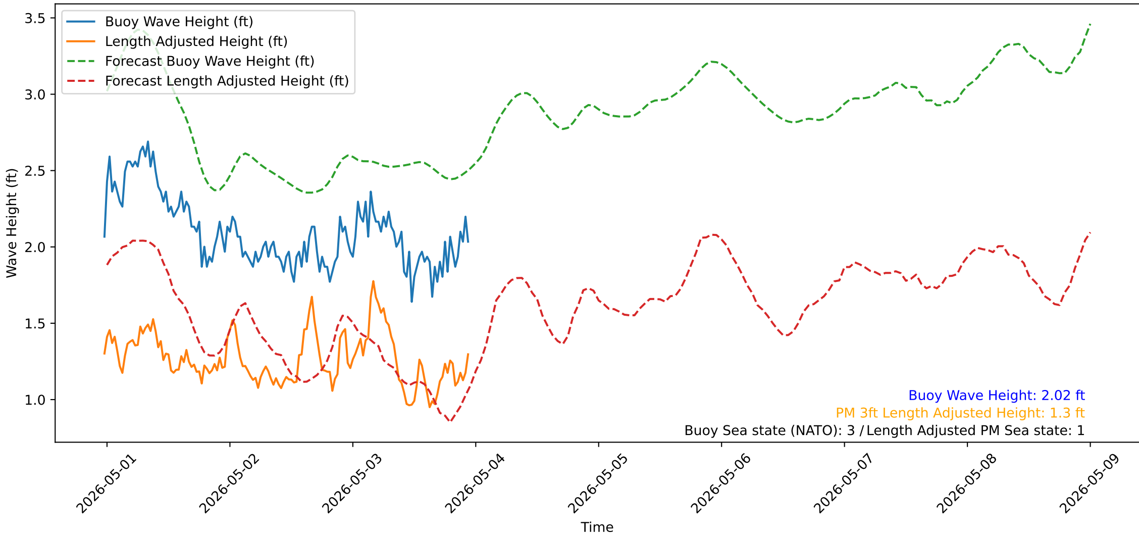
Wave Heights over Time for Oceanside Harbor at 2026-05-03 23:30:32
