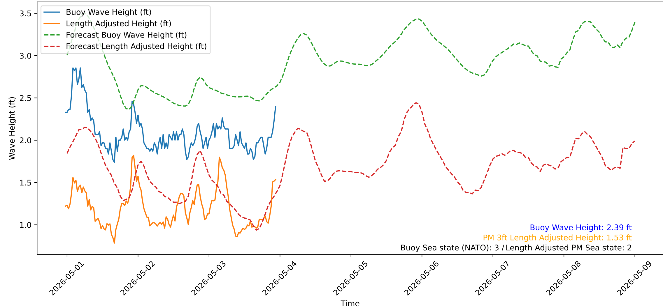
Wave Heights over Time for Green Beach at 2026-05-03 23:31:13
