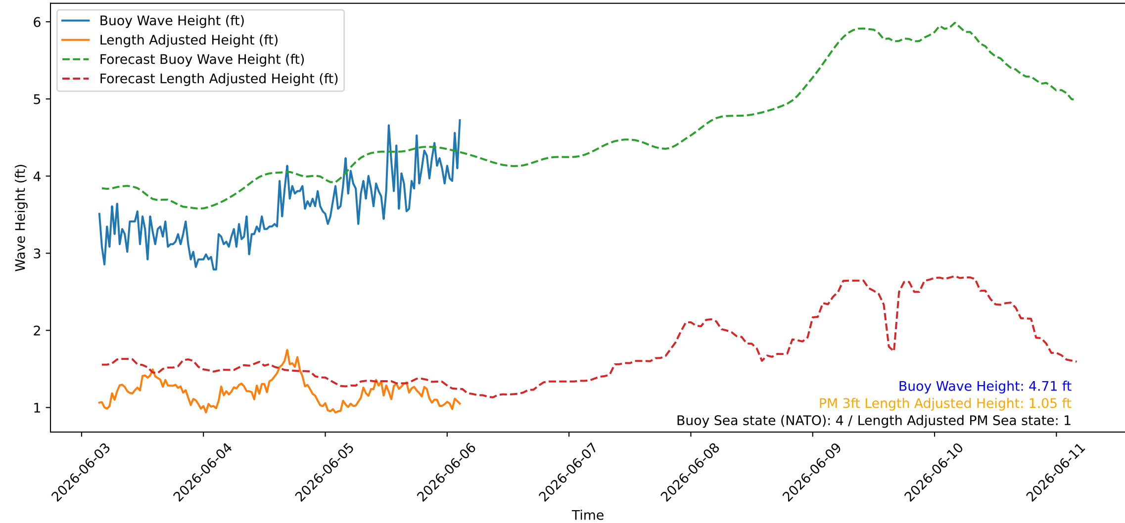
Wave Heights over Time for Green Beach at 2026-06-06 03:31:08
