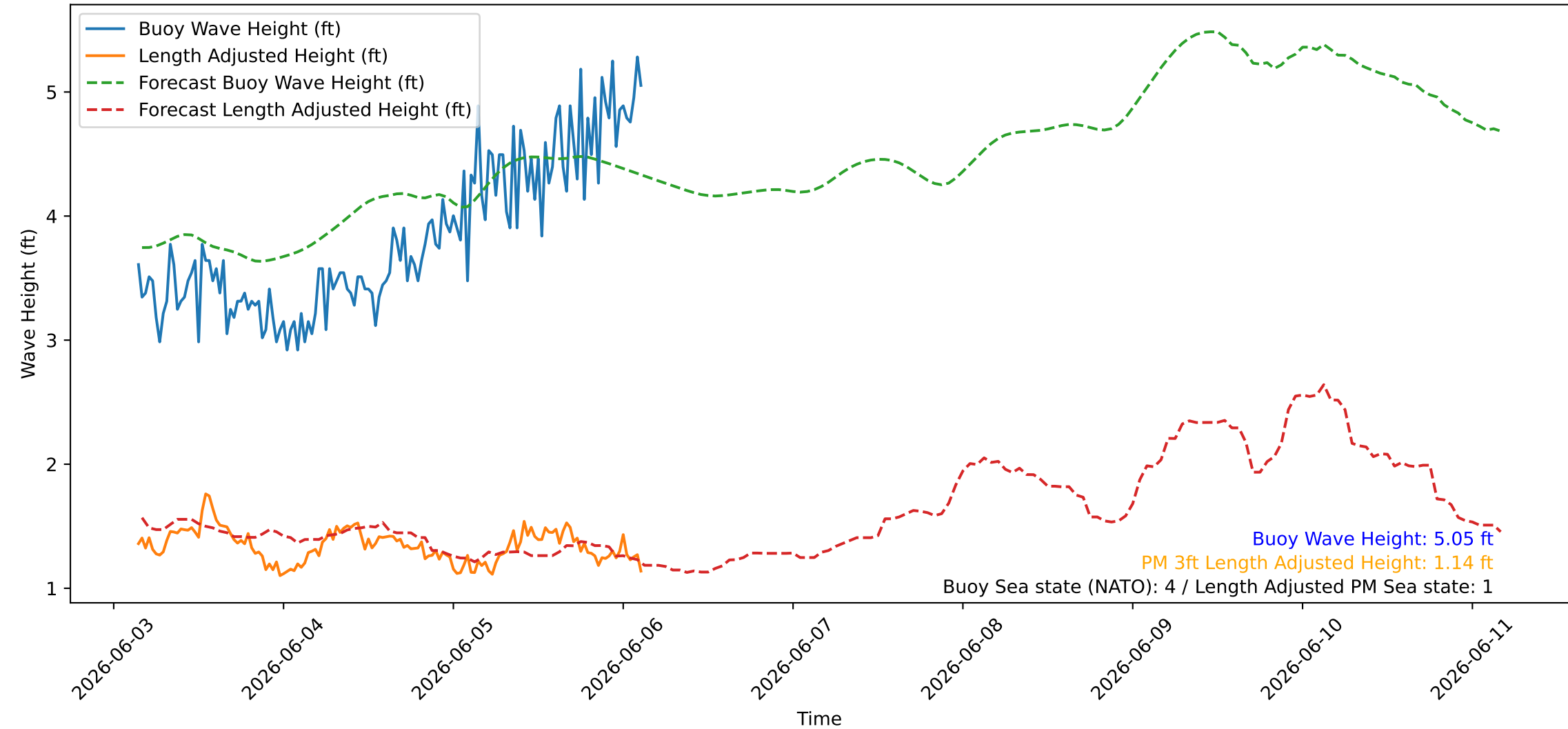
Wave Heights over Time for Oceanside Harbor at 2026-06-06 03:30:26
