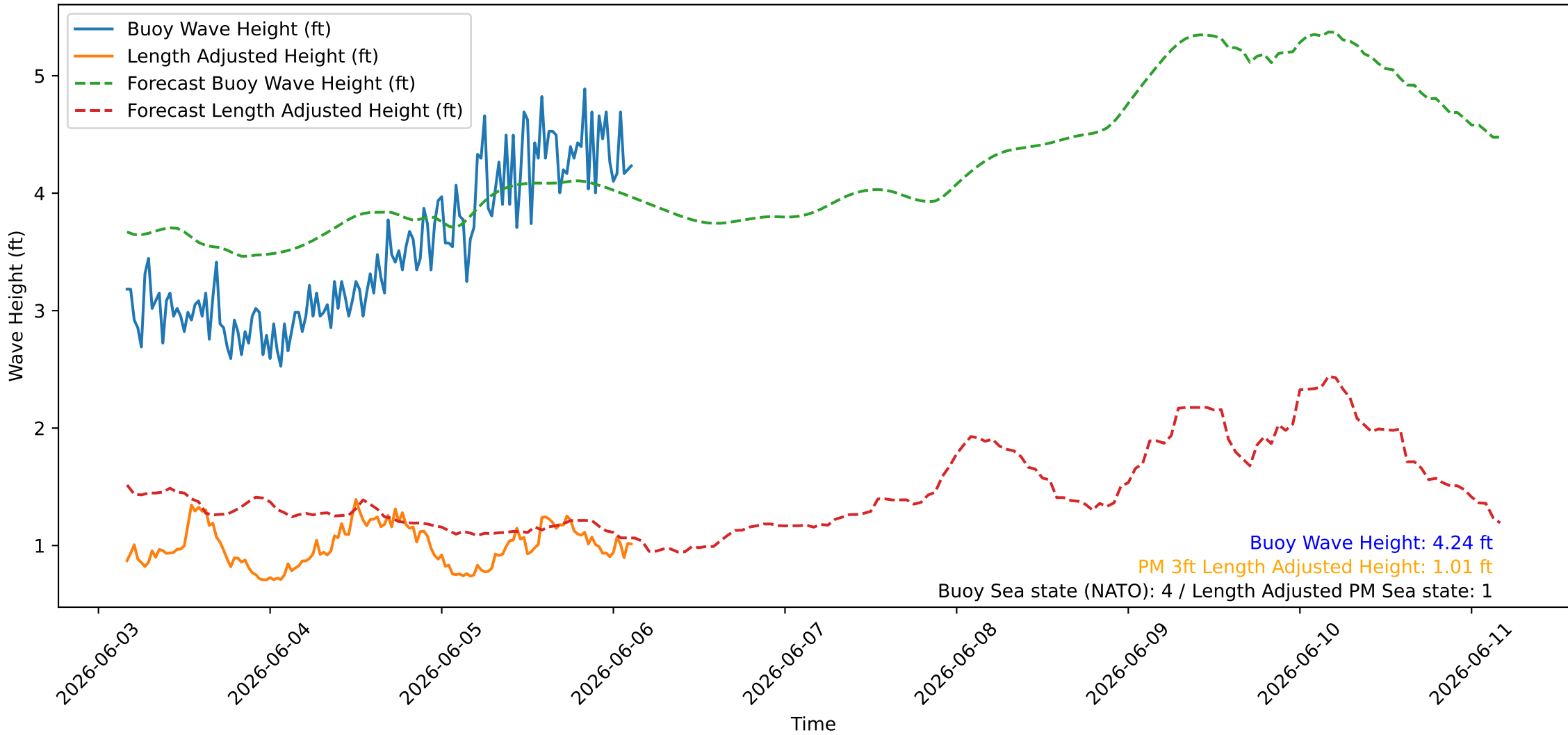
Wave Heights over Time for Red Beach at 2026-06-06 03:30:46
