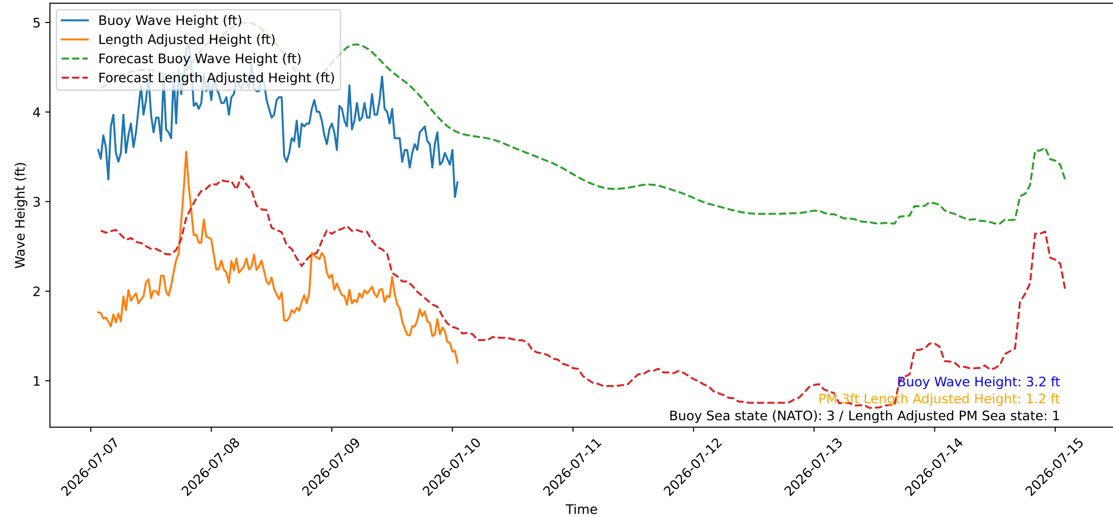
Wave Heights over Time for Green Beach at 2026-07-10 01:41:08
