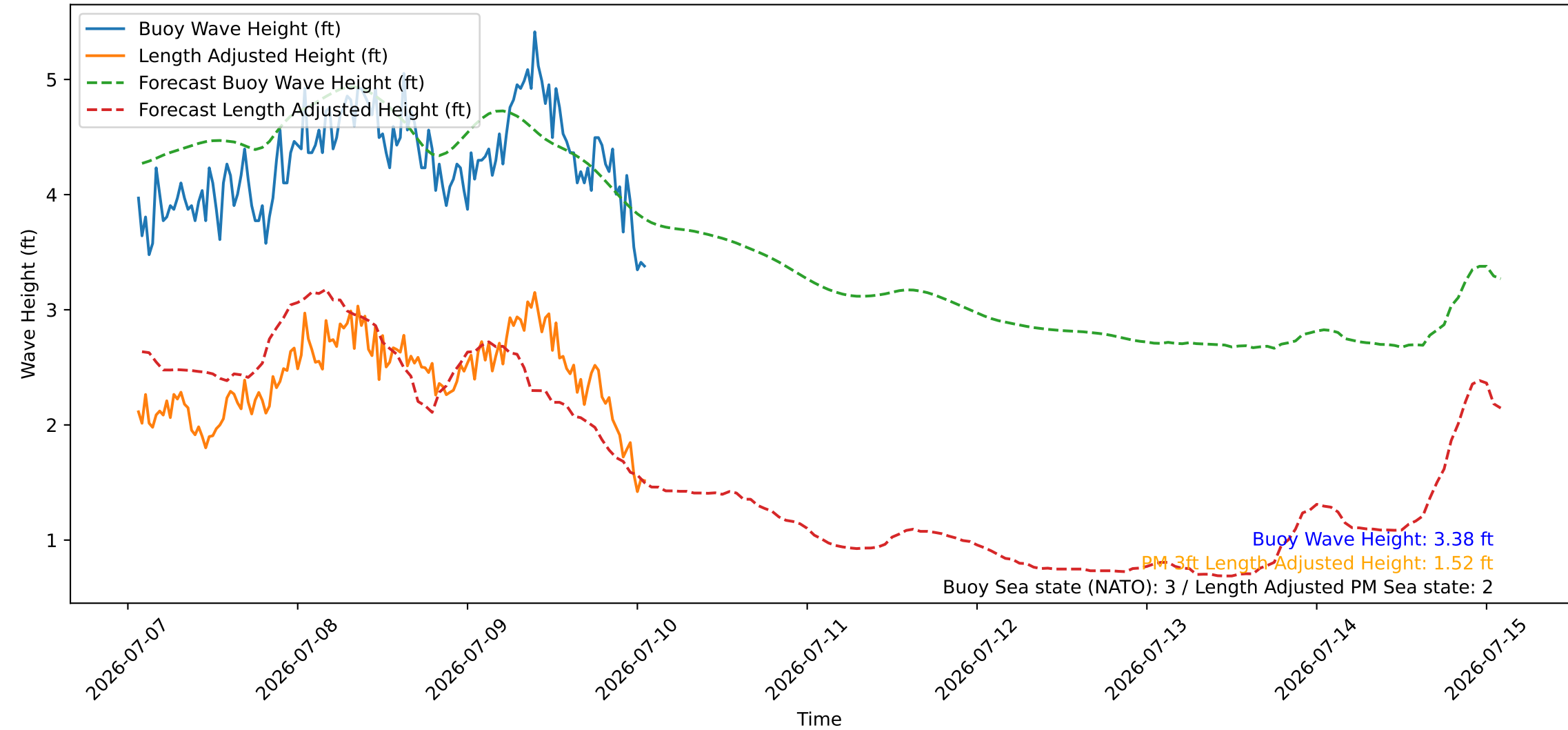
Wave Heights over Time for Oceanside Harbor at 2026-07-10 01:40:26
