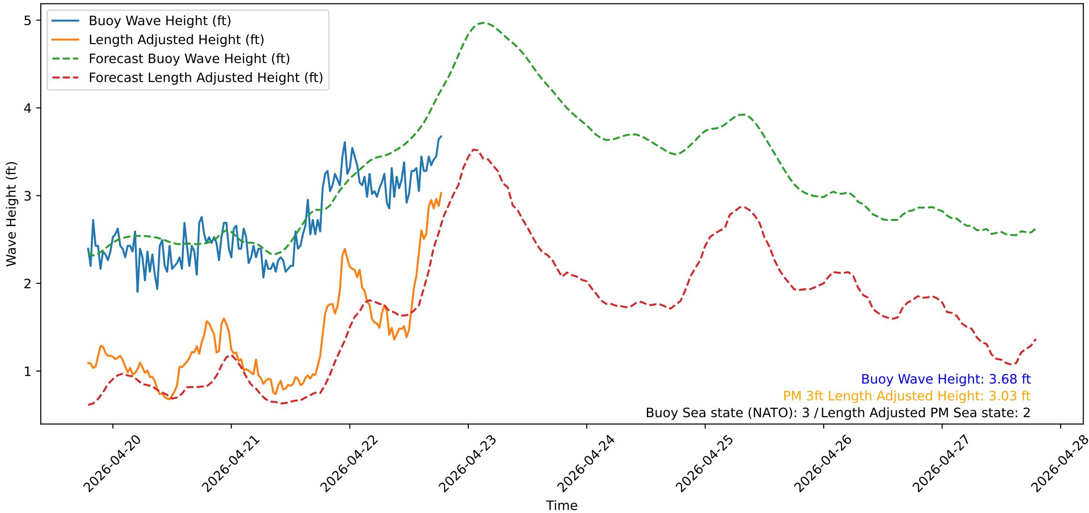
Wave Heights over Time for Oceanside Harbor at 2026-04-22 19:10:31
