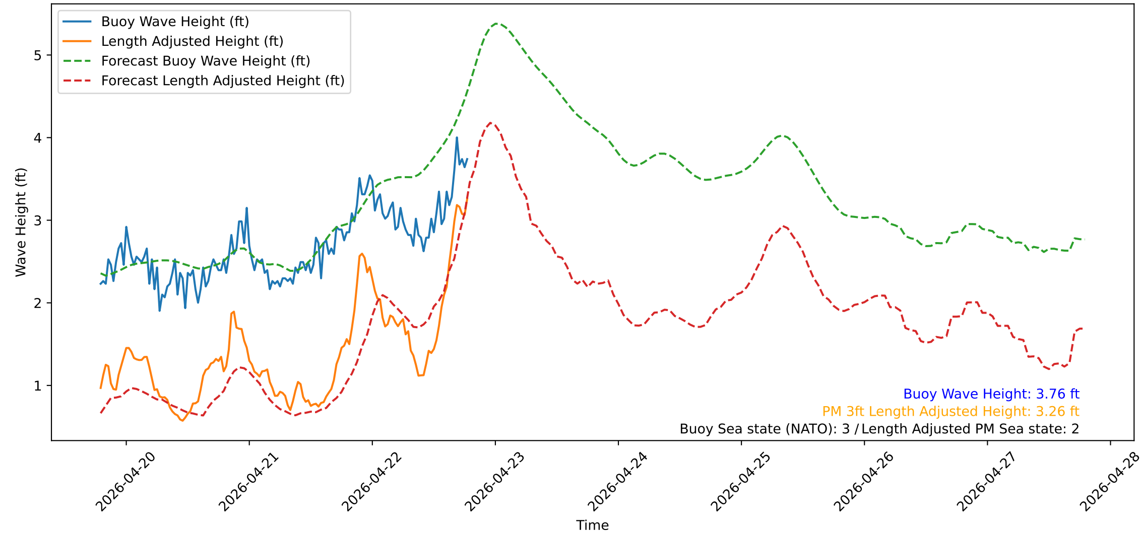
Wave Heights over Time for Green Beach at 2026-04-22 19:11:13
