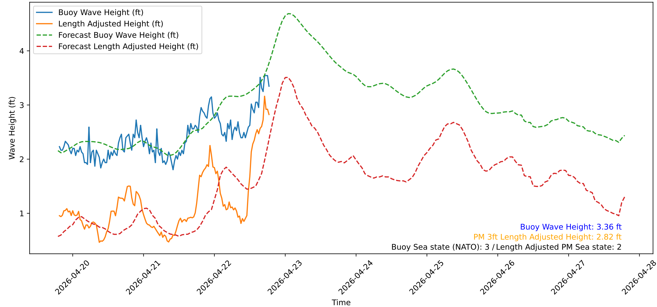
Wave Heights over Time for Red Beach at 2026-04-22 19:10:50
