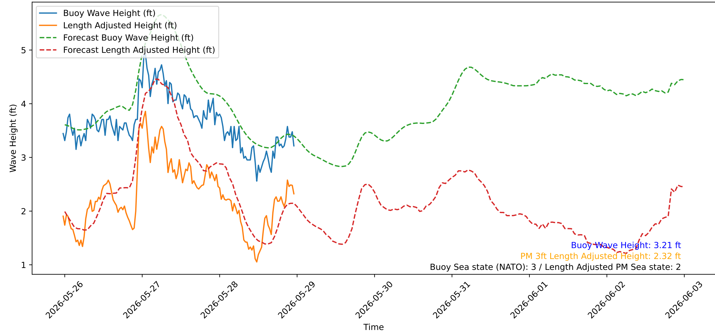
Wave Heights over Time for Green Beach at 2026-05-28 23:41:03
