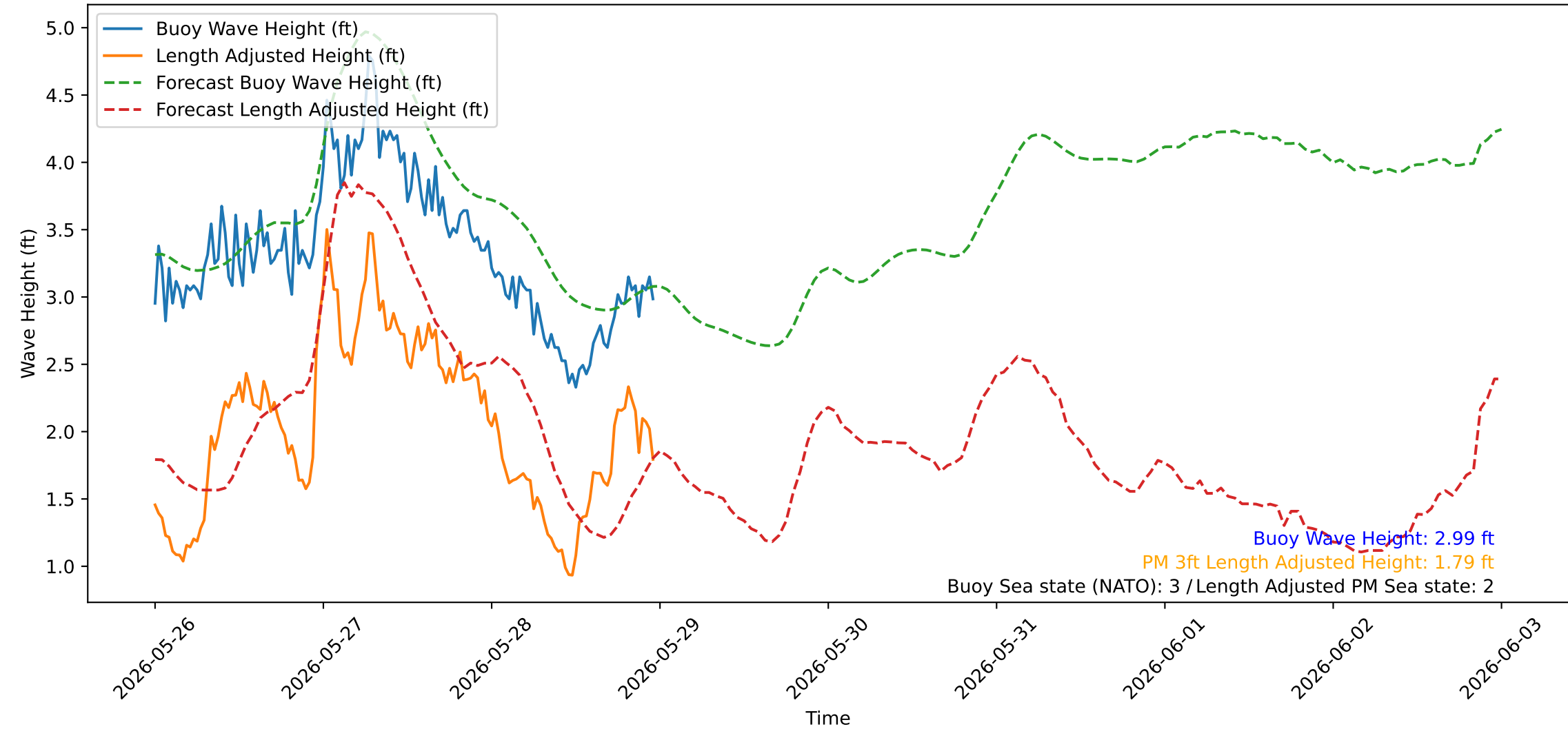
Wave Heights over Time for Red Beach at 2026-05-28 23:40:40
