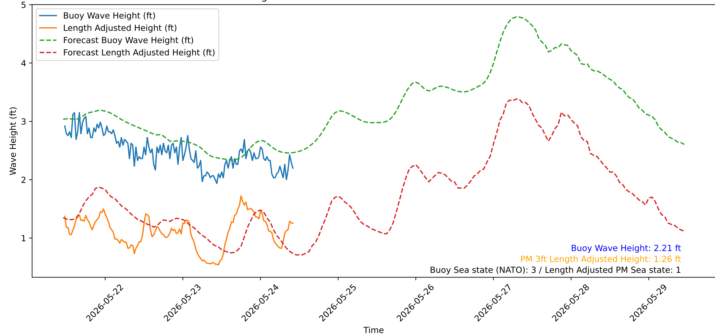
Wave Heights over Time for Red Beach at 2026-05-24 11:00:52
