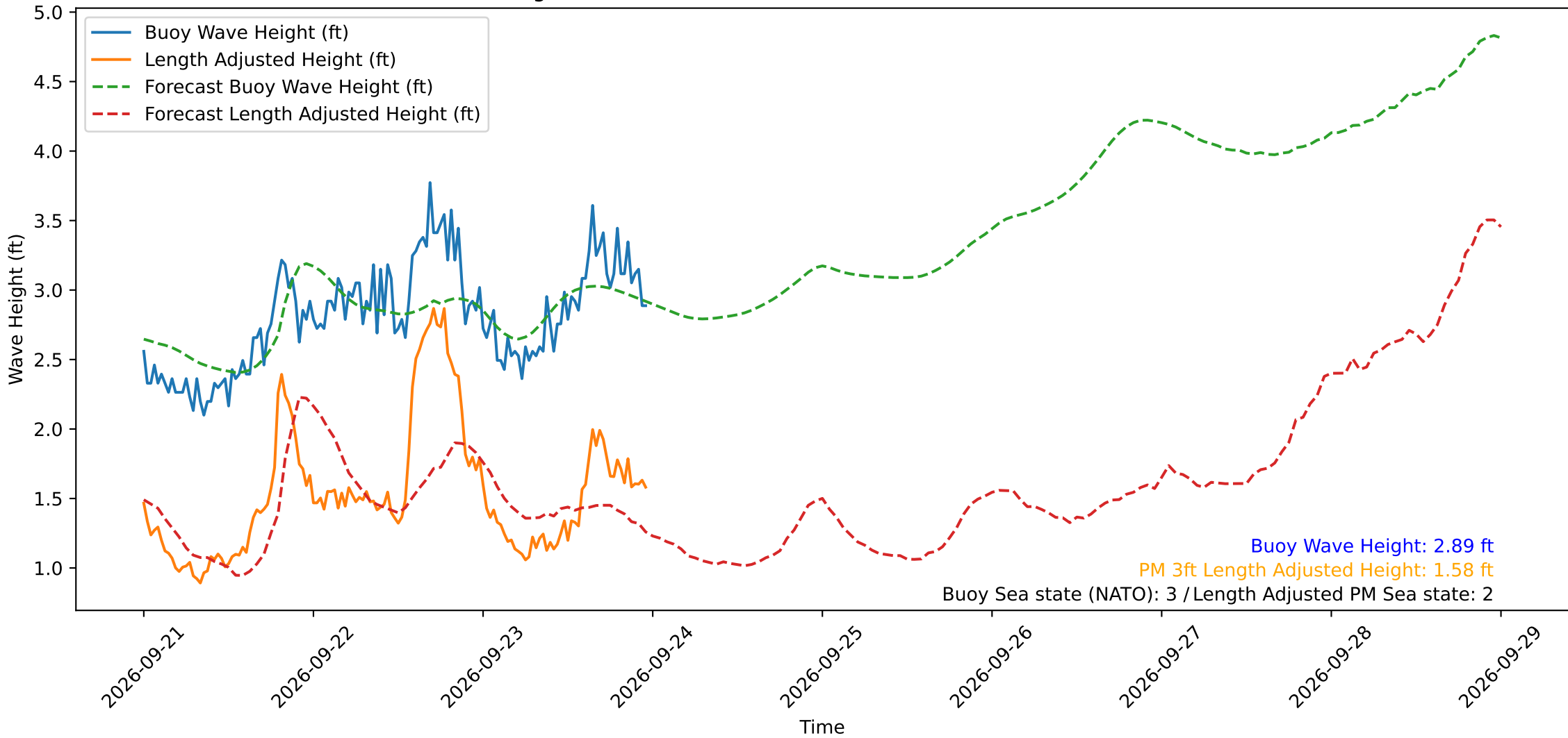
Wave Heights over Time for Oceanside Harbor at 2026-09-24 00:00:29
