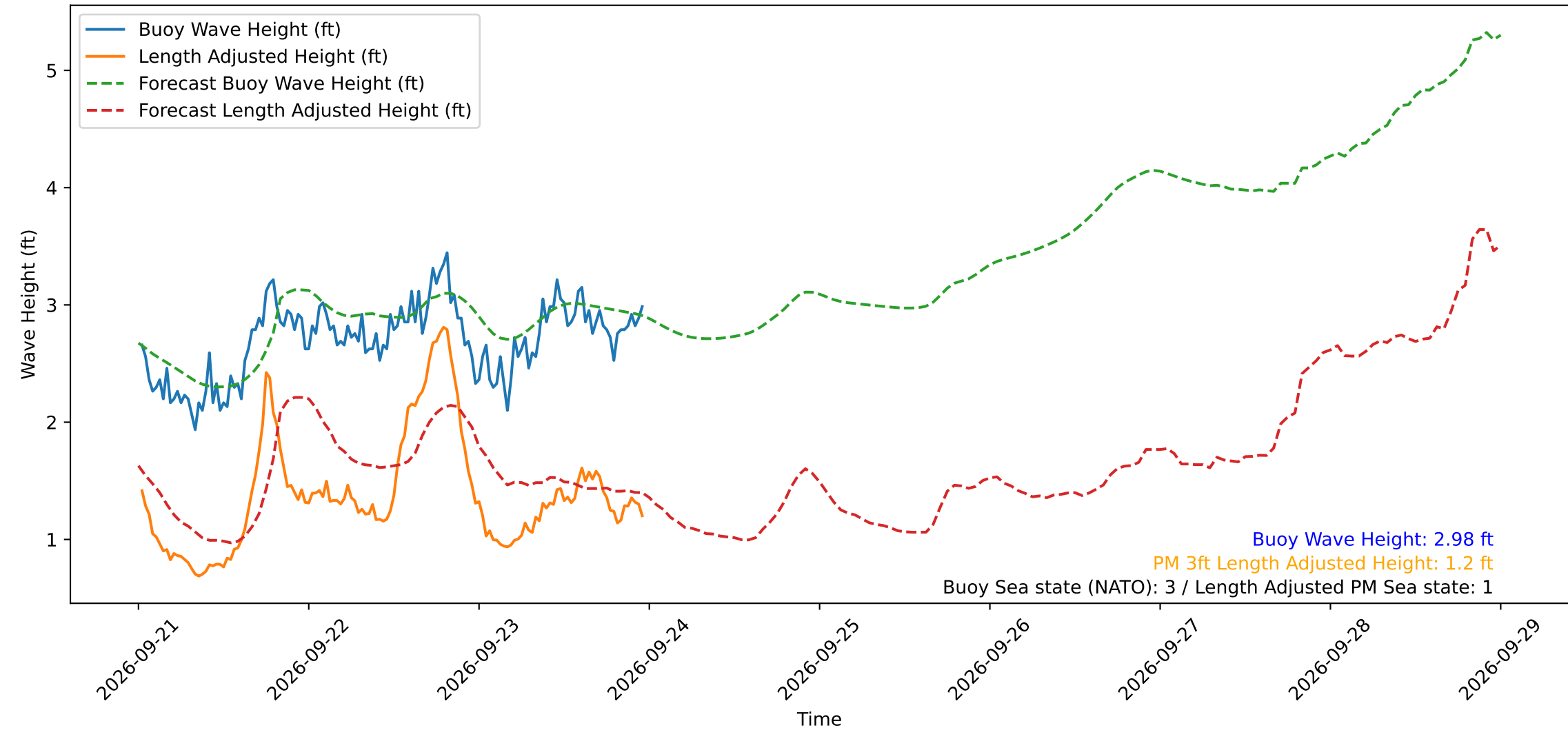
Wave Heights over Time for Green Beach at 2026-09-24 00:01:11
