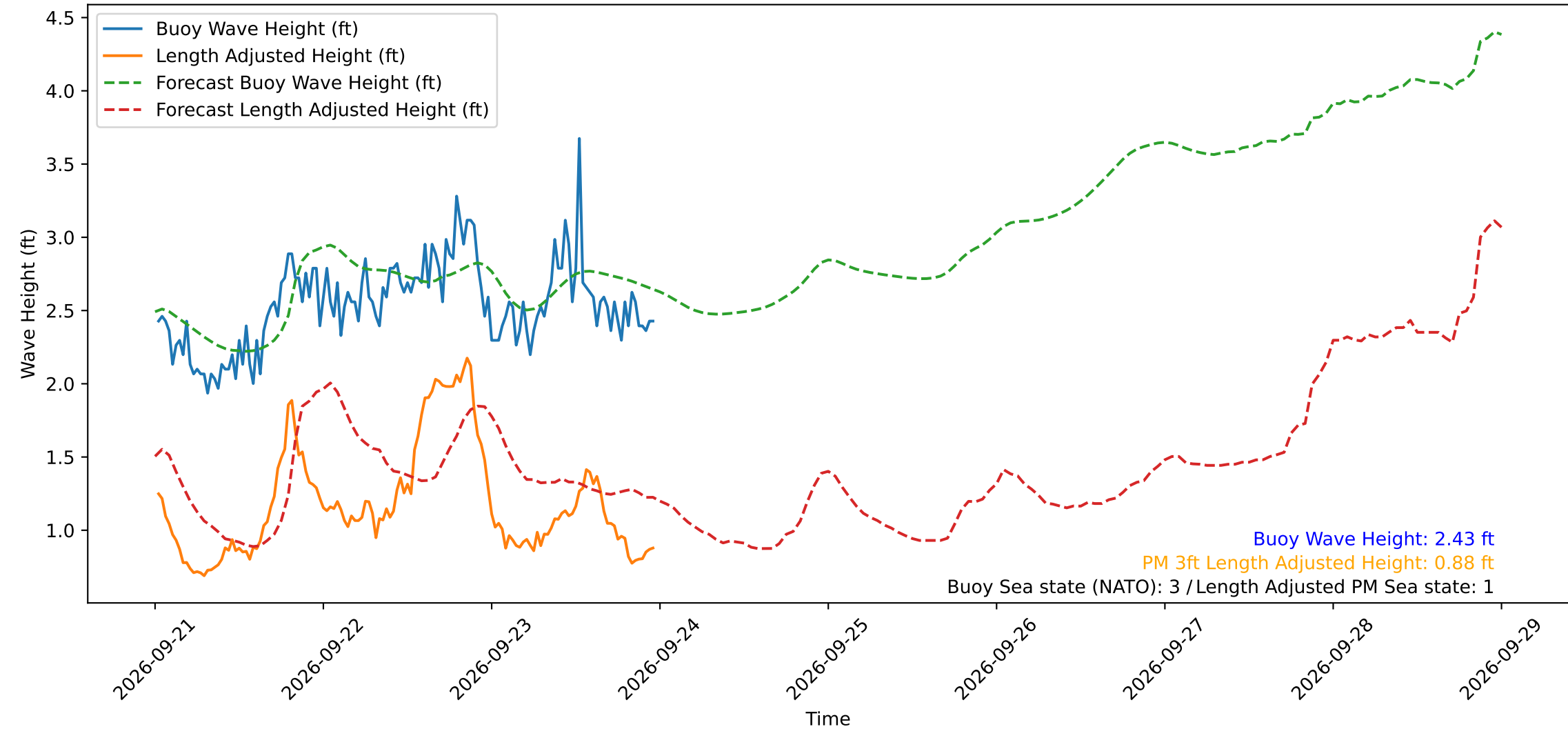
Wave Heights over Time for Red Beach at 2026-09-24 00:00:49
