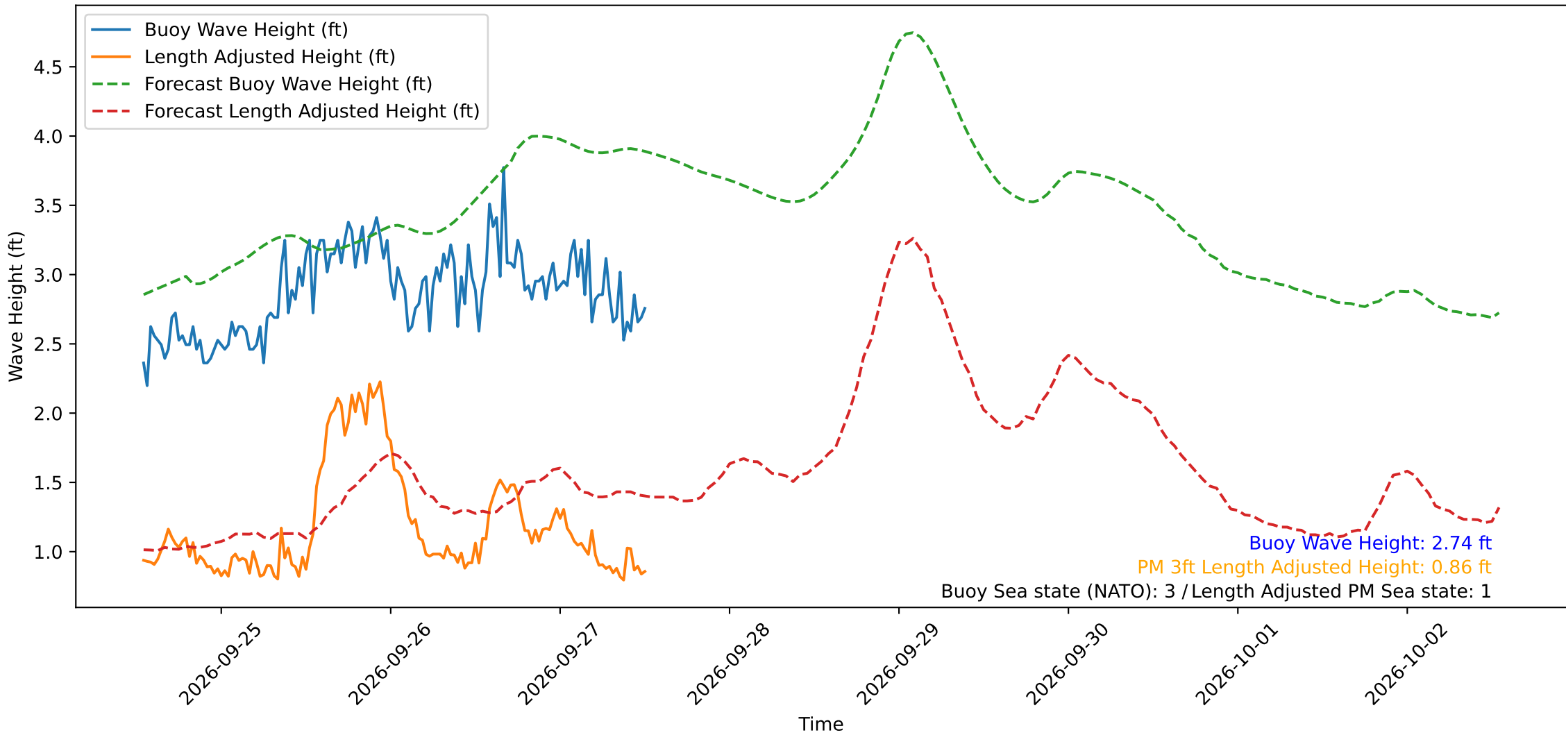
Wave Heights over Time for Oceanside Harbor at 2026-09-27 12:50:30
