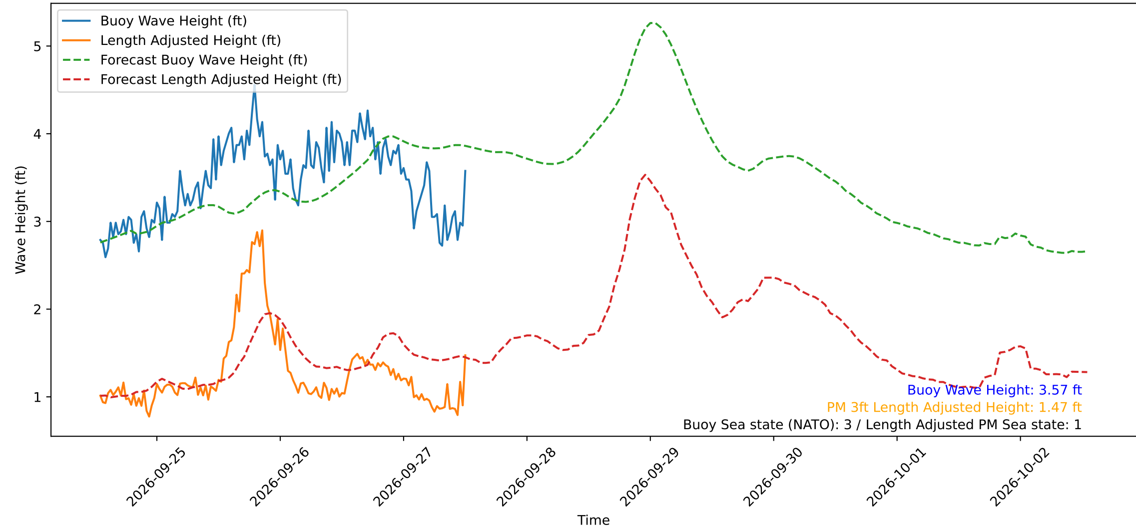
Wave Heights over Time for Green Beach at 2026-09-27 12:51:16
