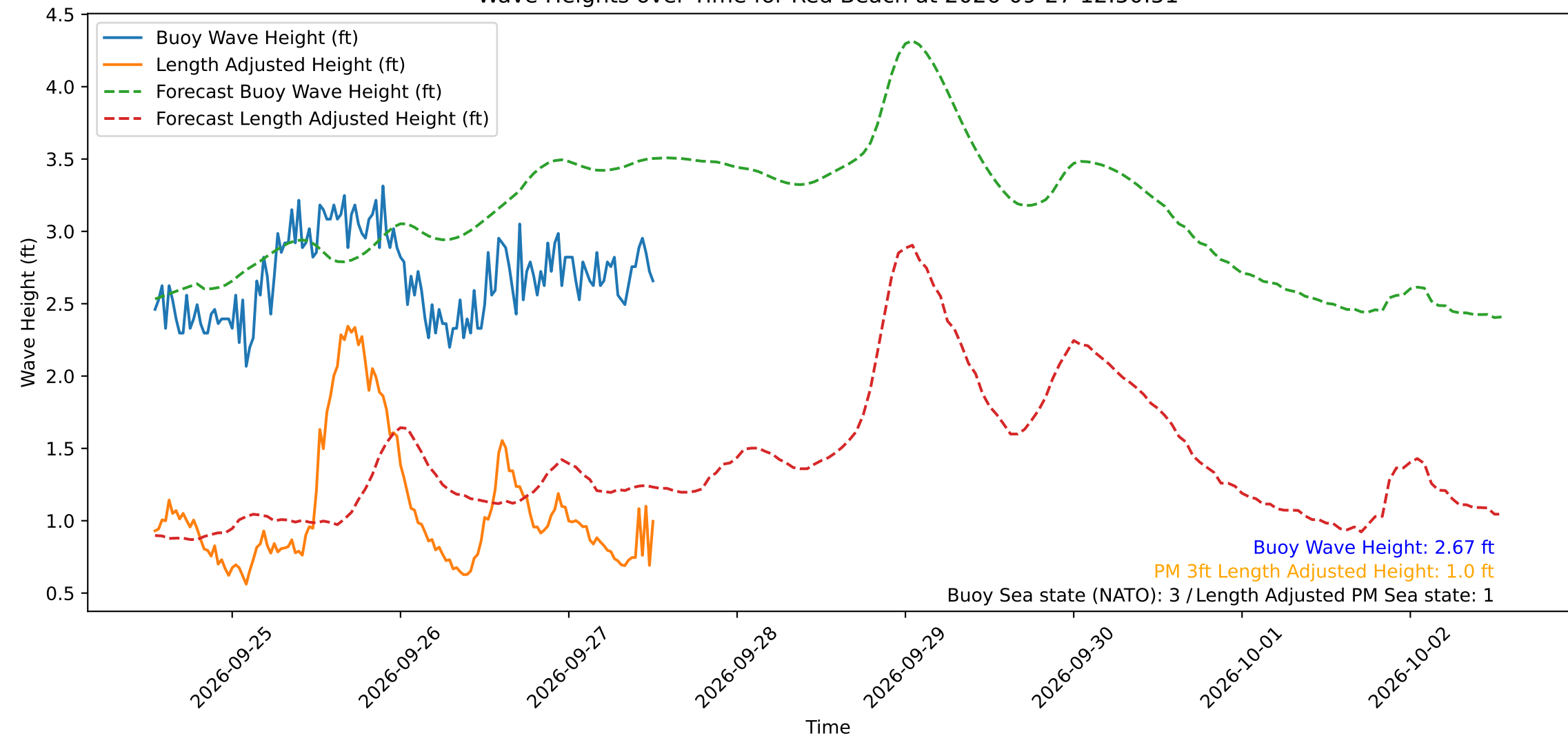
Wave Heights over Time for Red Beach at 2026-09-27 12:50:51
