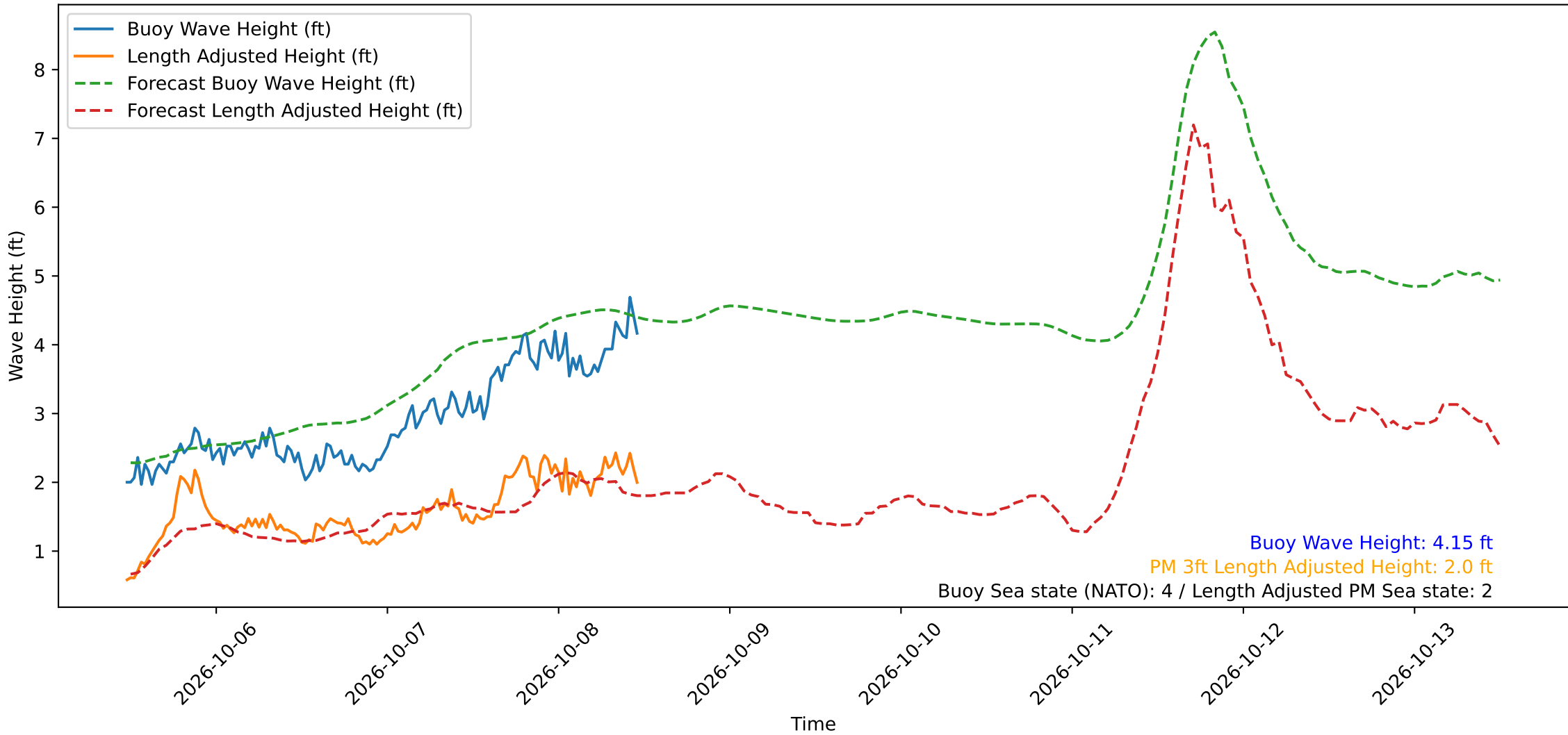
Wave Heights over Time for Oceanside Harbor at 2026-10-08 11:40:30
