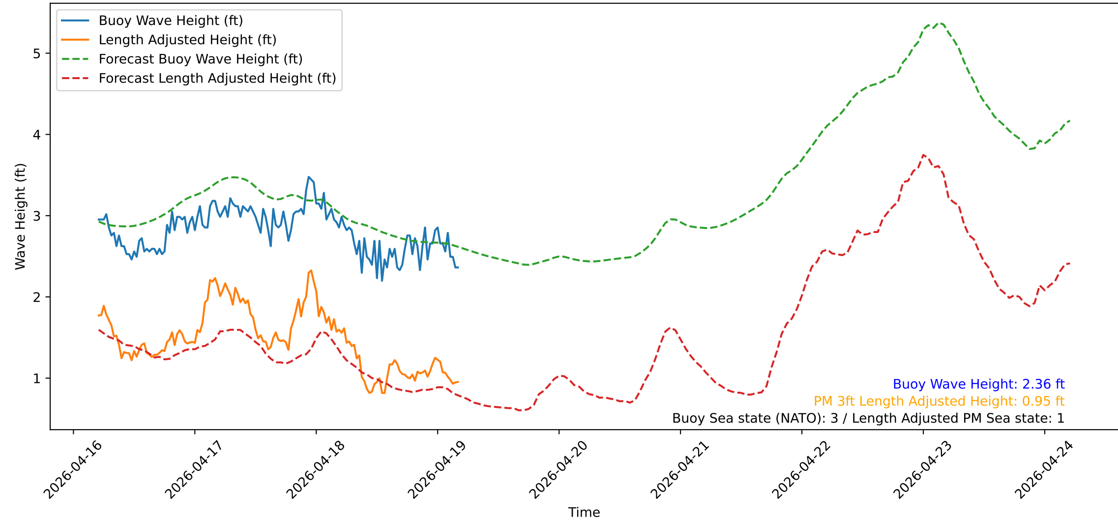
Wave Heights over Time for Green Beach at 2026-04-19 04:51:12
