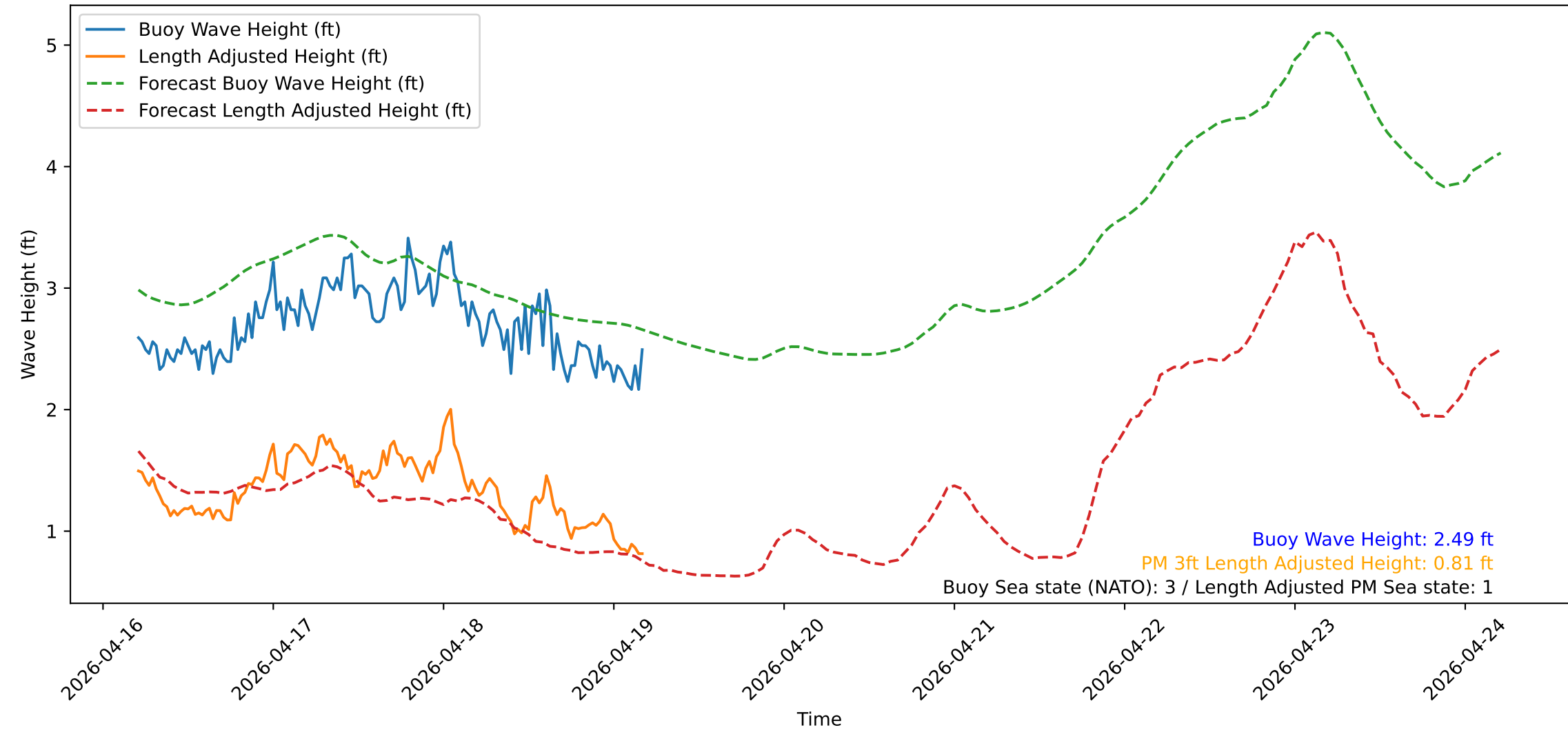
Wave Heights over Time for Oceanside Harbor at 2026-04-19 04:50:30
