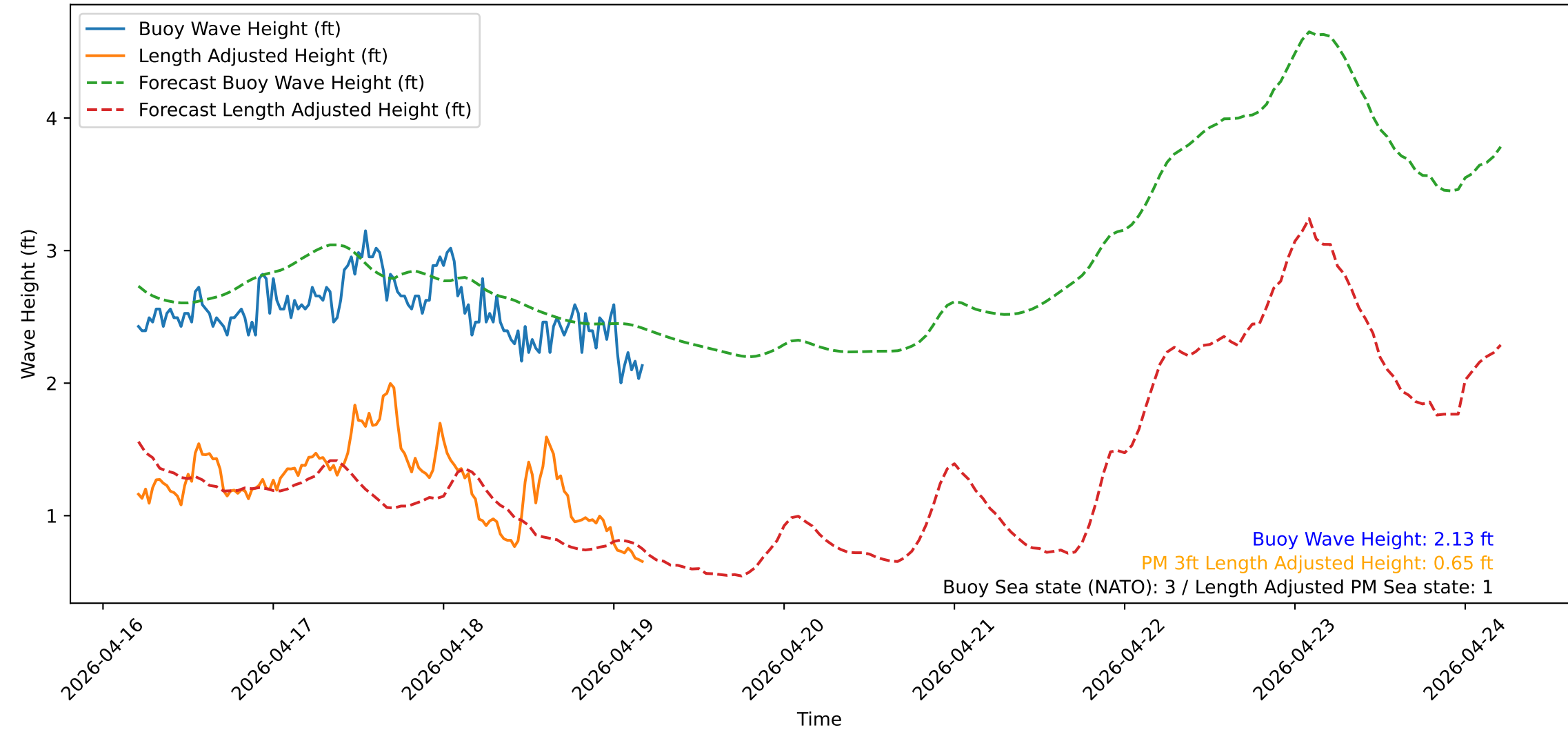
Wave Heights over Time for Red Beach at 2026-04-19 04:50:50
