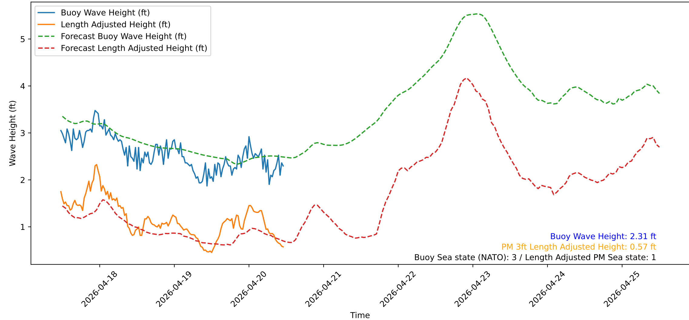
Wave Heights over Time for Green Beach at 2026-04-20 11:41:13
