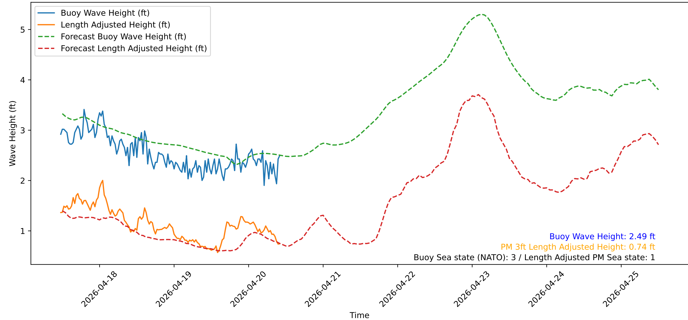
Wave Heights over Time for Oceanside Harbor at 2026-04-20 11:40:31
