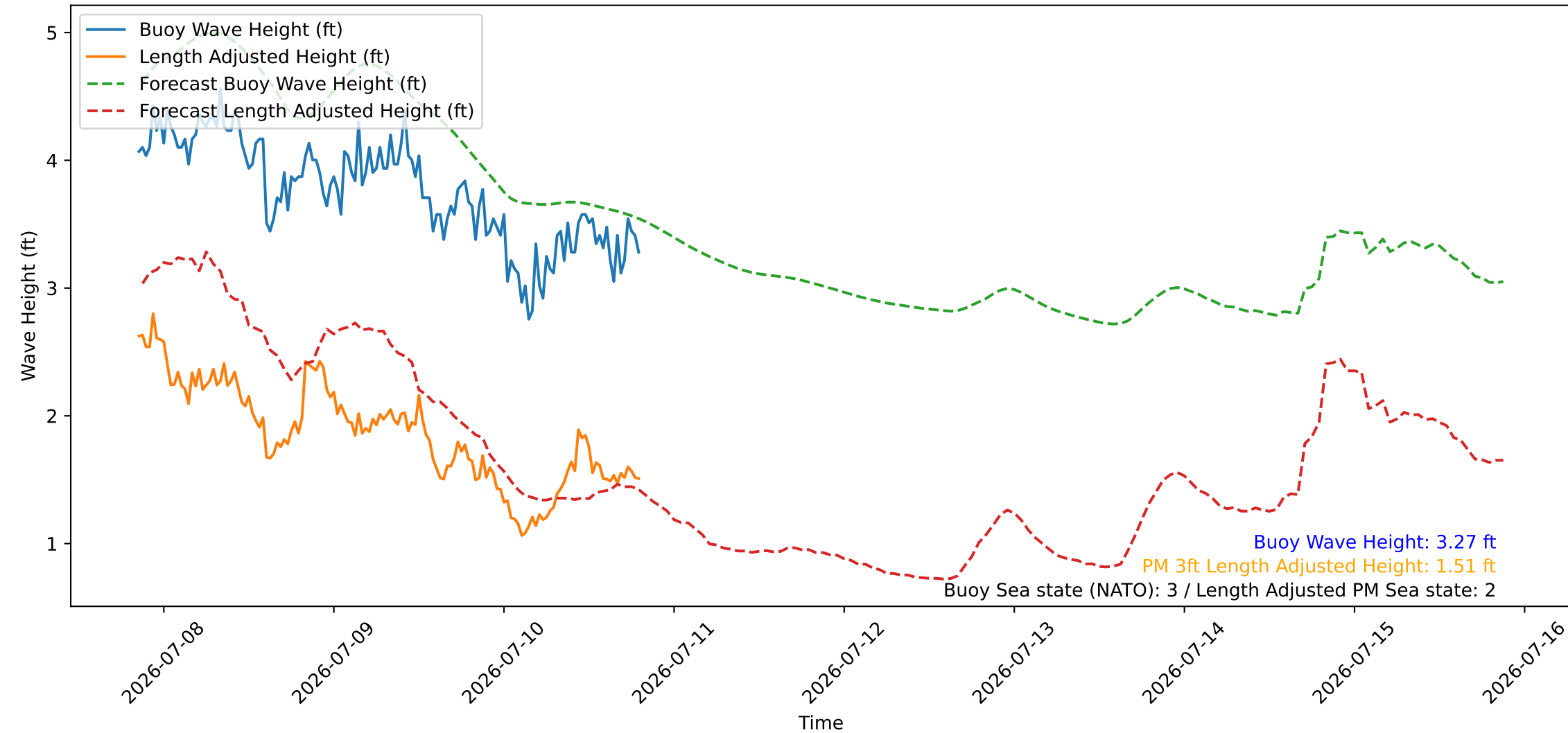
Wave Heights over Time for Green Beach at 2026-07-10 20:31:08
