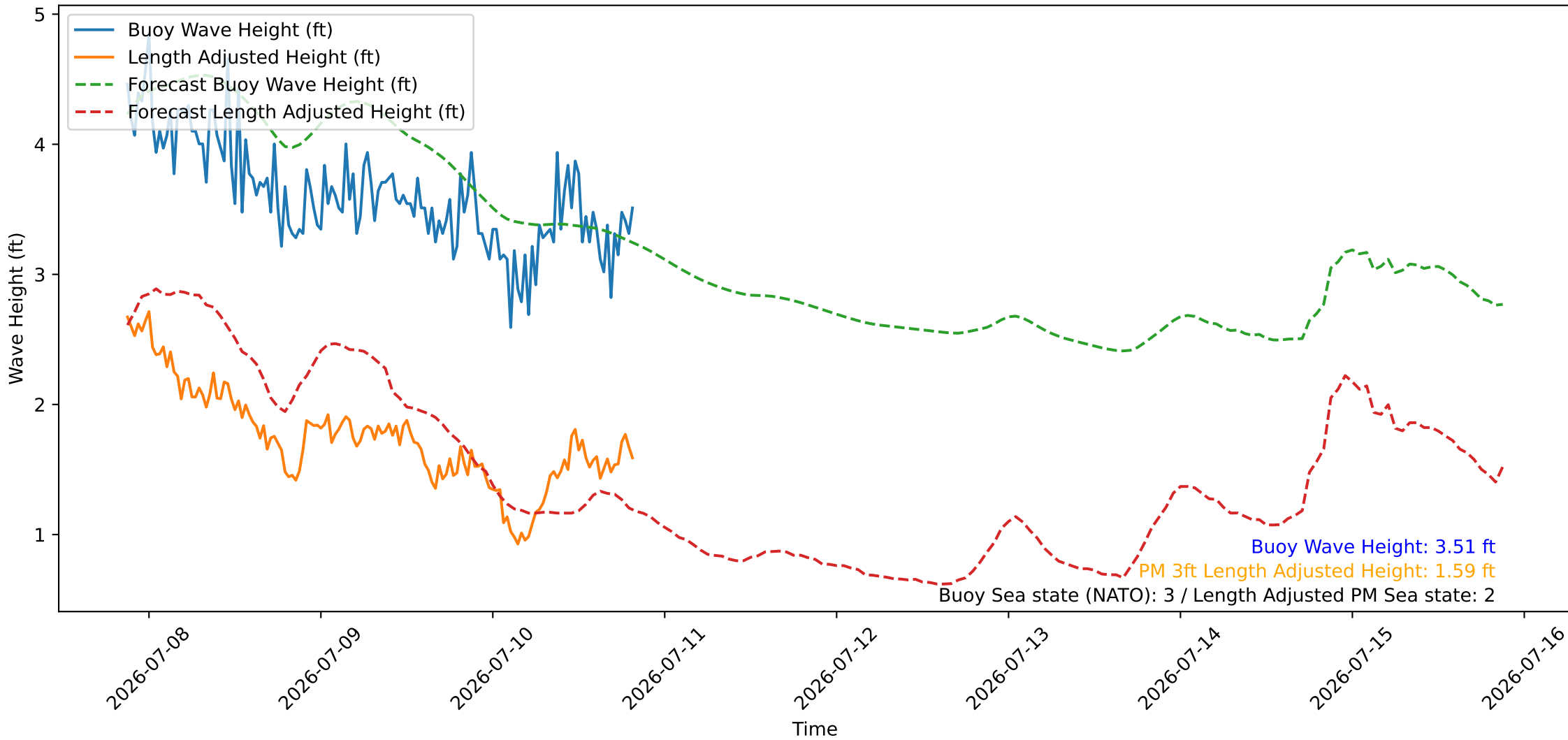
Wave Heights over Time for Red Beach at 2026-07-10 20:30:45
