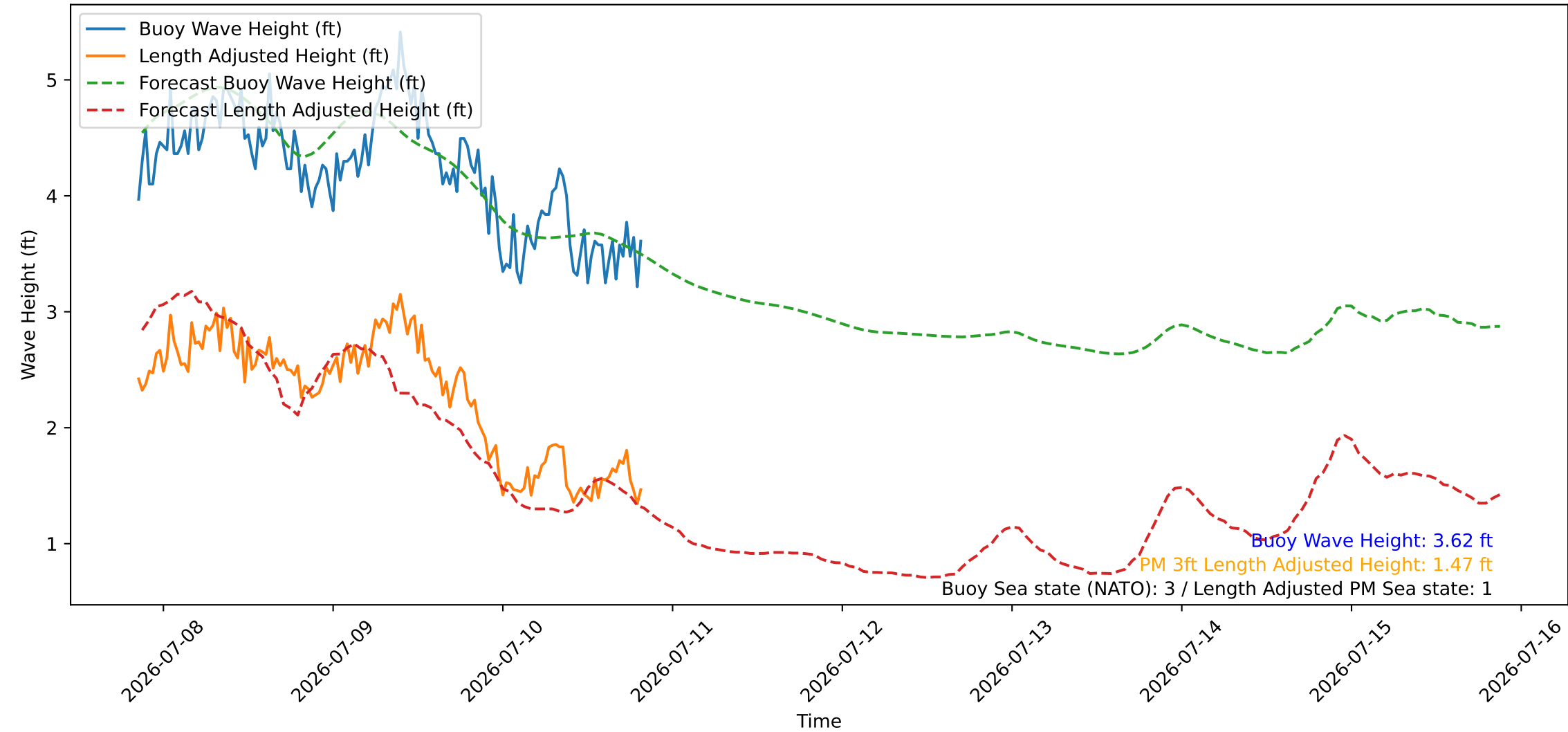
Wave Heights over Time for Oceanside Harbor at 2026-07-10 20:30:26
