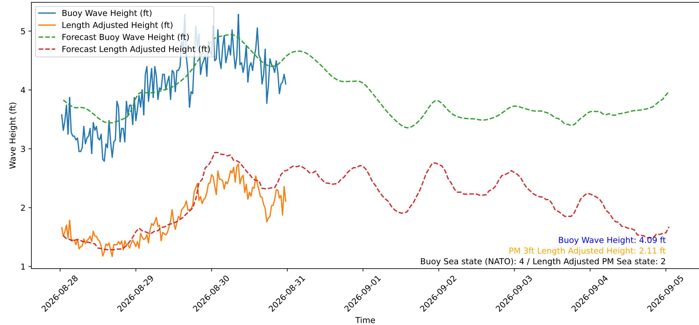
Wave Heights over Time for Oceanside Harbor at 2026-08-31 00:30:30
