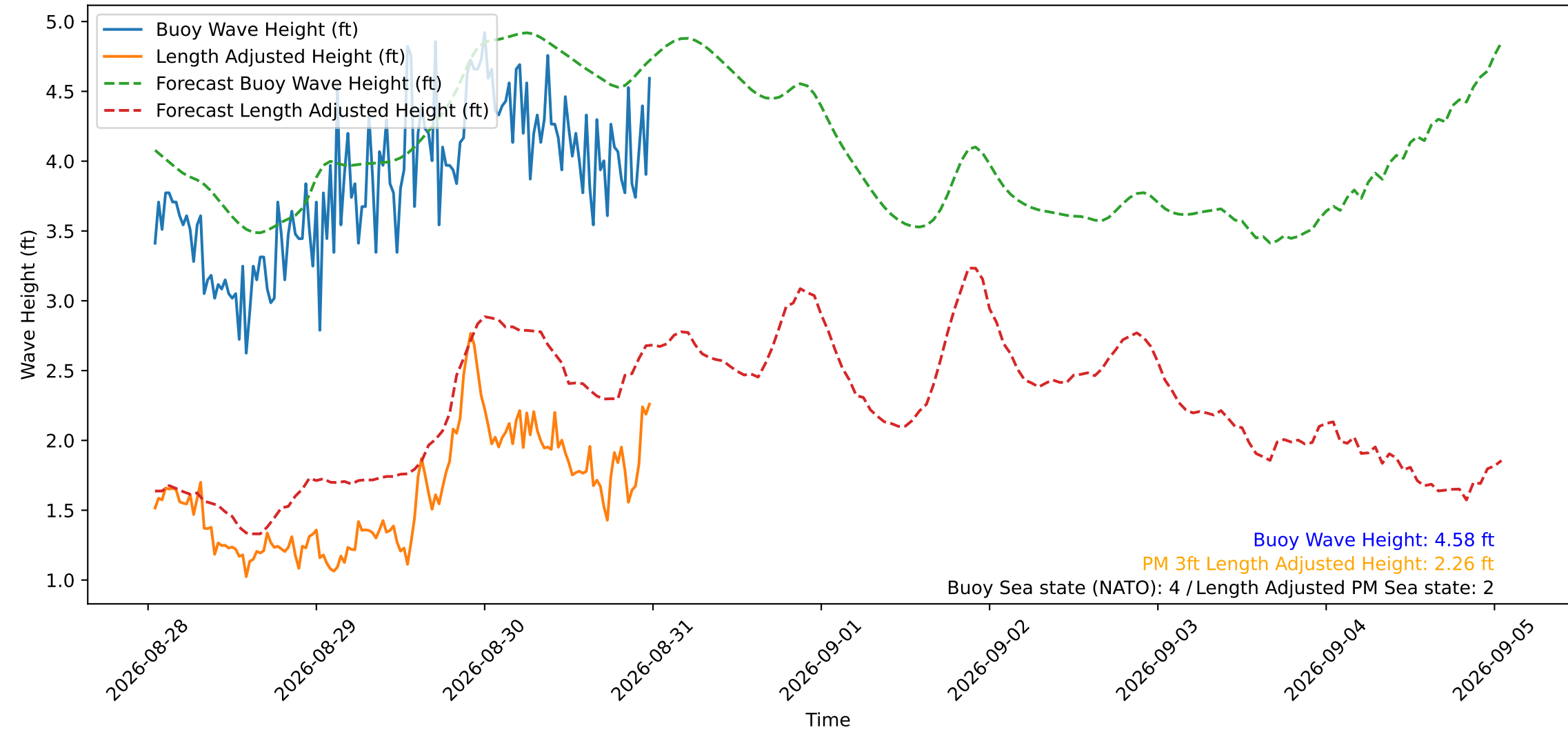
Wave Heights over Time for Green Beach at 2026-08-31 00:31:12
