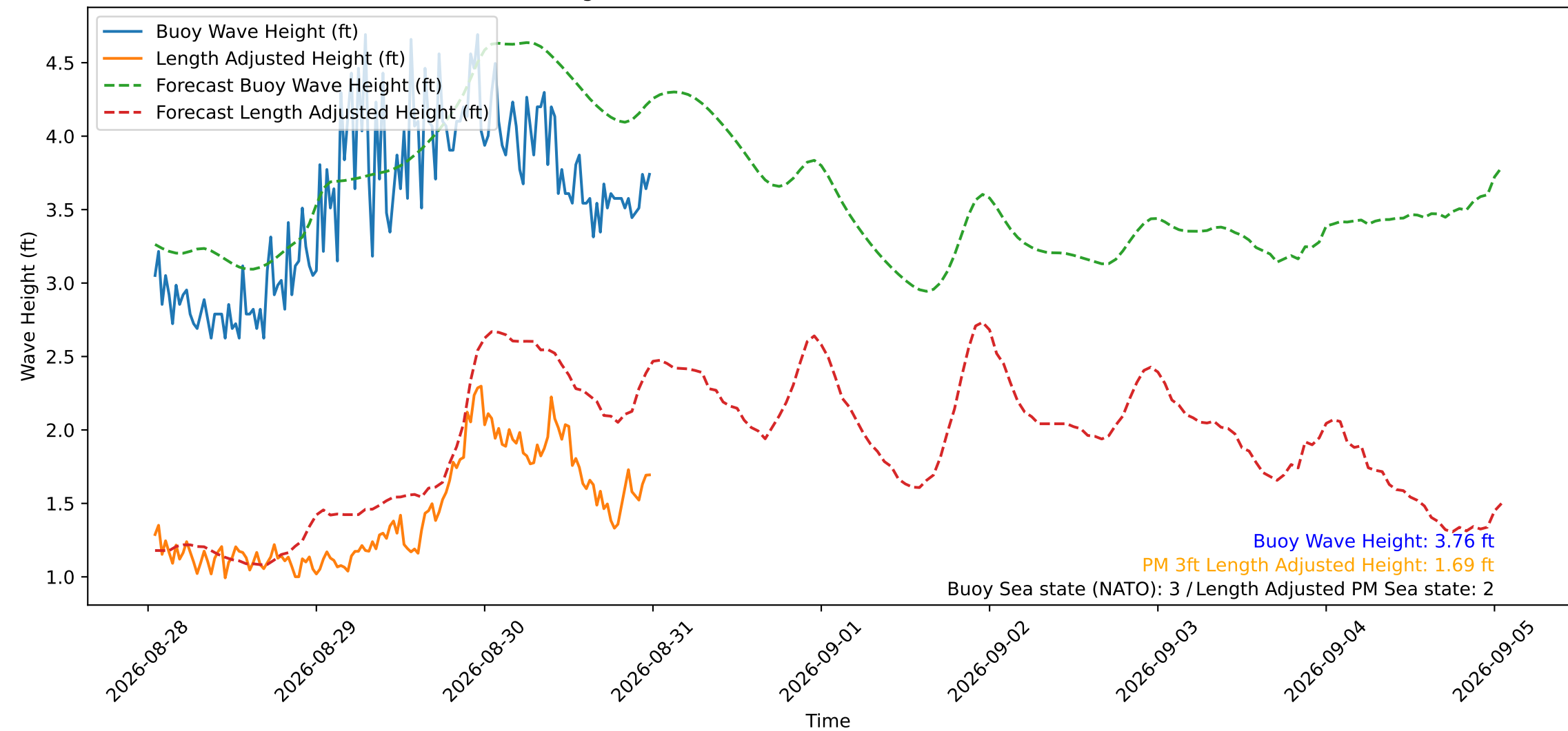
Wave Heights over Time for Red Beach at 2026-08-31 00:30:49
