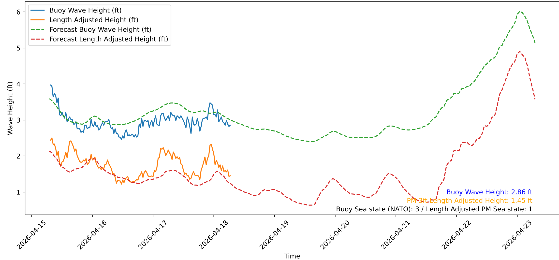
Wave Heights over Time for Green Beach at 2026-04-18 07:21:13
