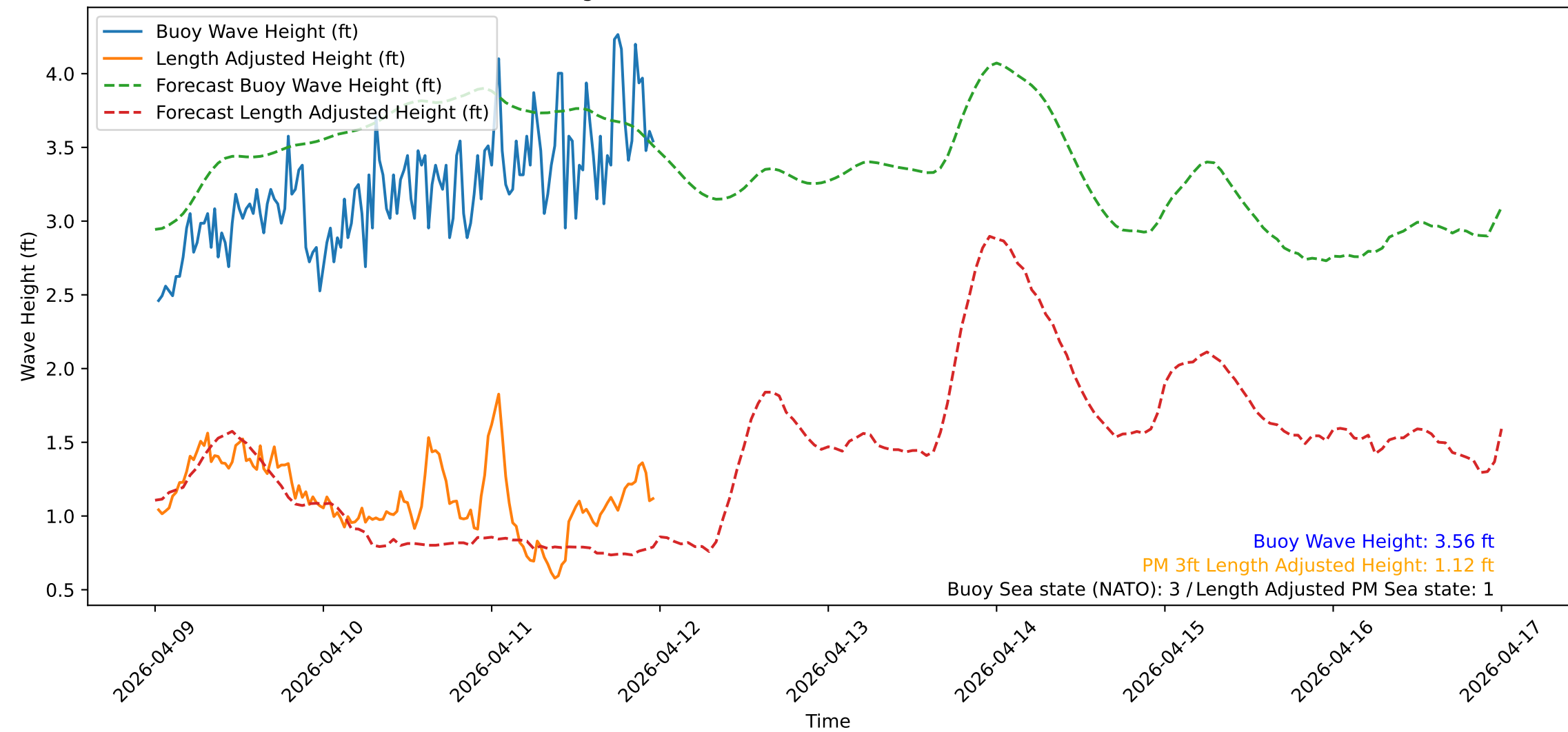
Wave Heights over Time for Red Beach at 2026-04-12 00:00:50
