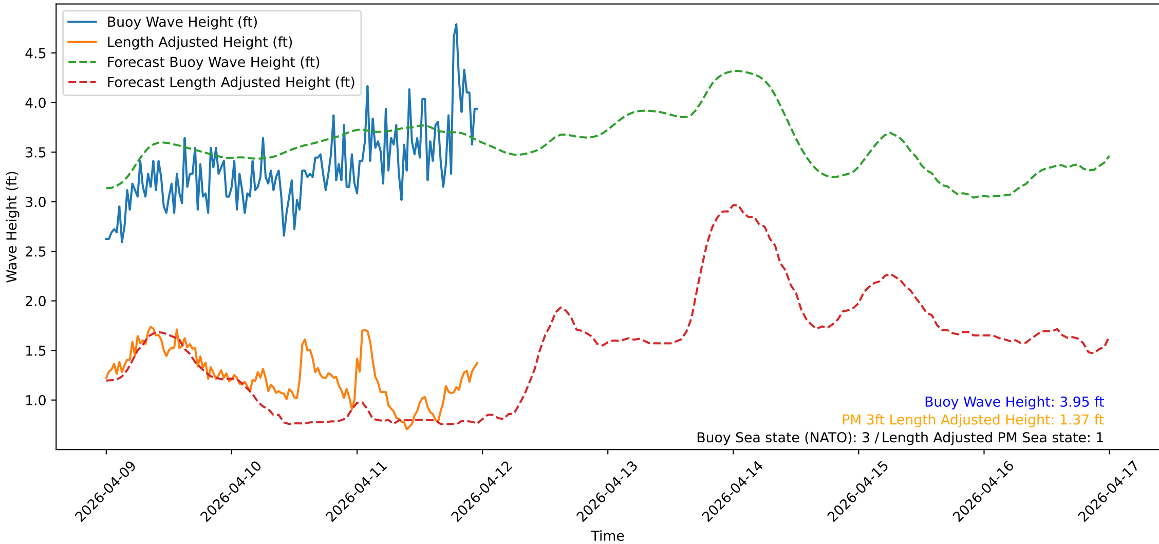
Wave Heights over Time for Oceanside Harbor at 2026-04-12 00:00:31
