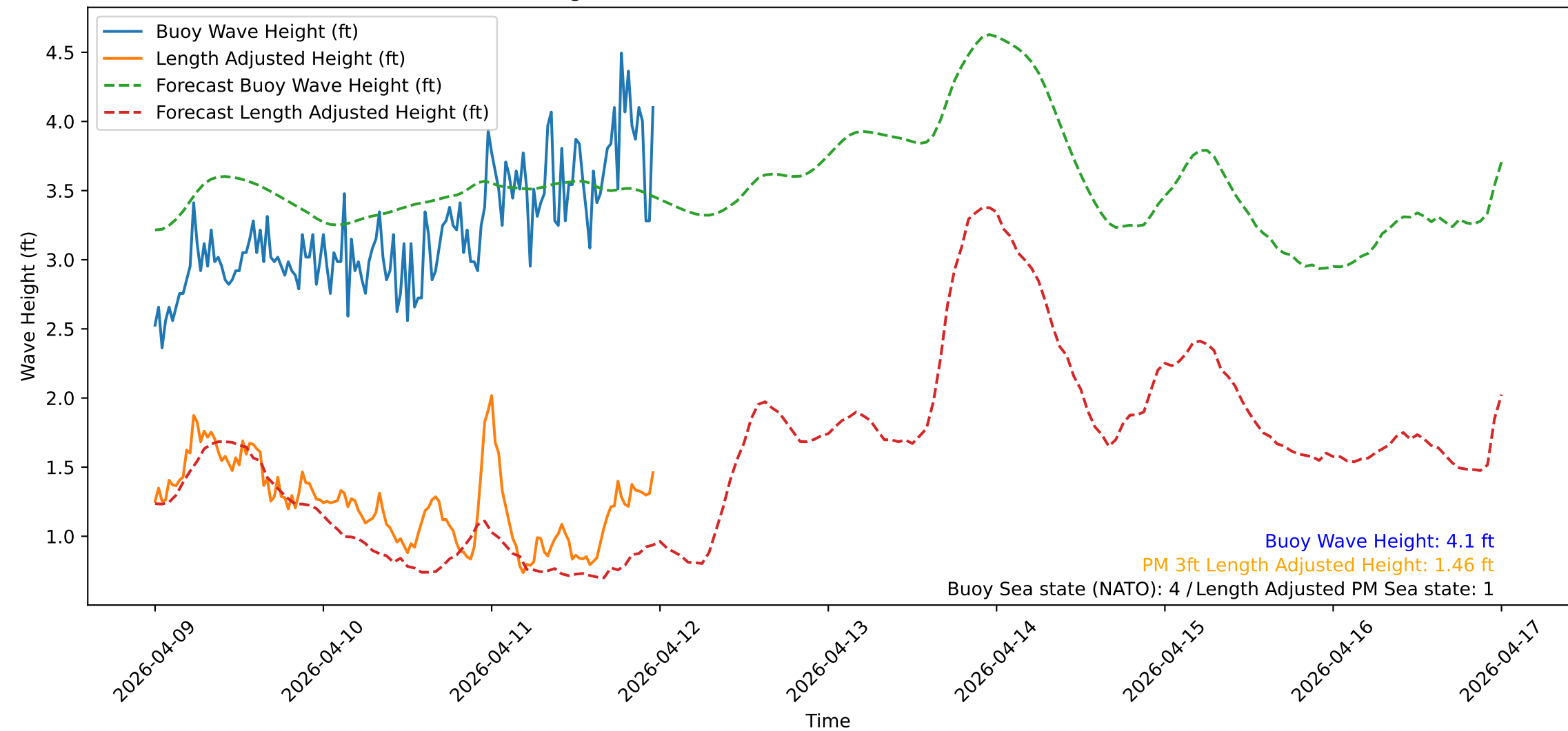
Wave Heights over Time for Green Beach at 2026-04-12 00:01:12
