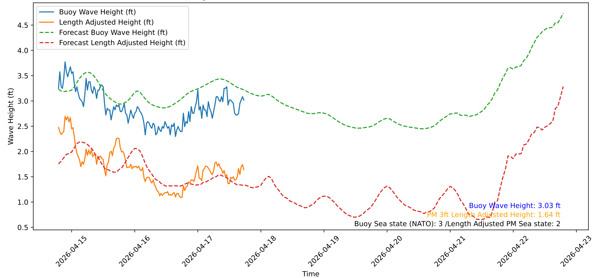
Wave Heights over Time for Oceanside Harbor at 2026-04-17 18:50:31
