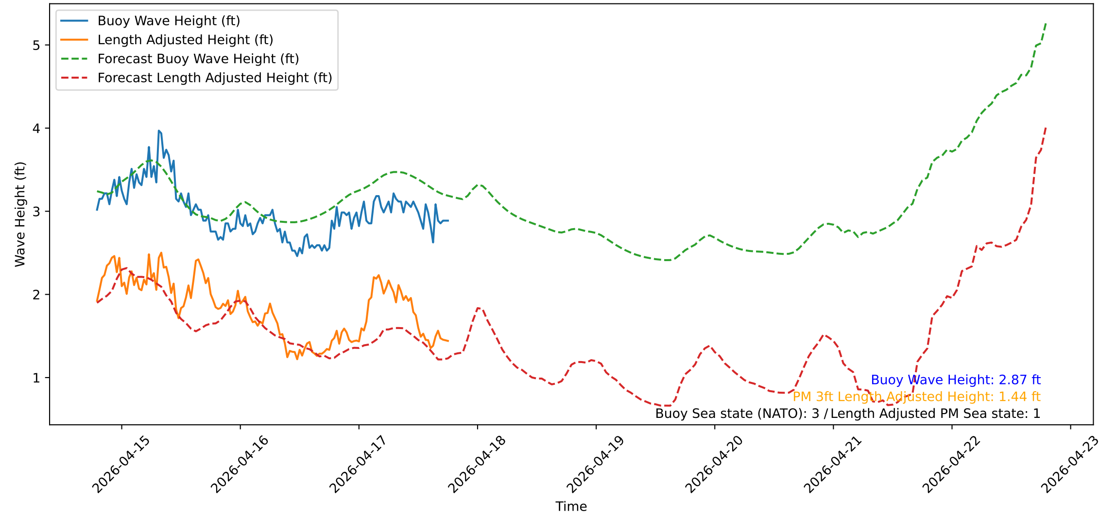
Wave Heights over Time for Green Beach at 2026-04-17 18:51:14
