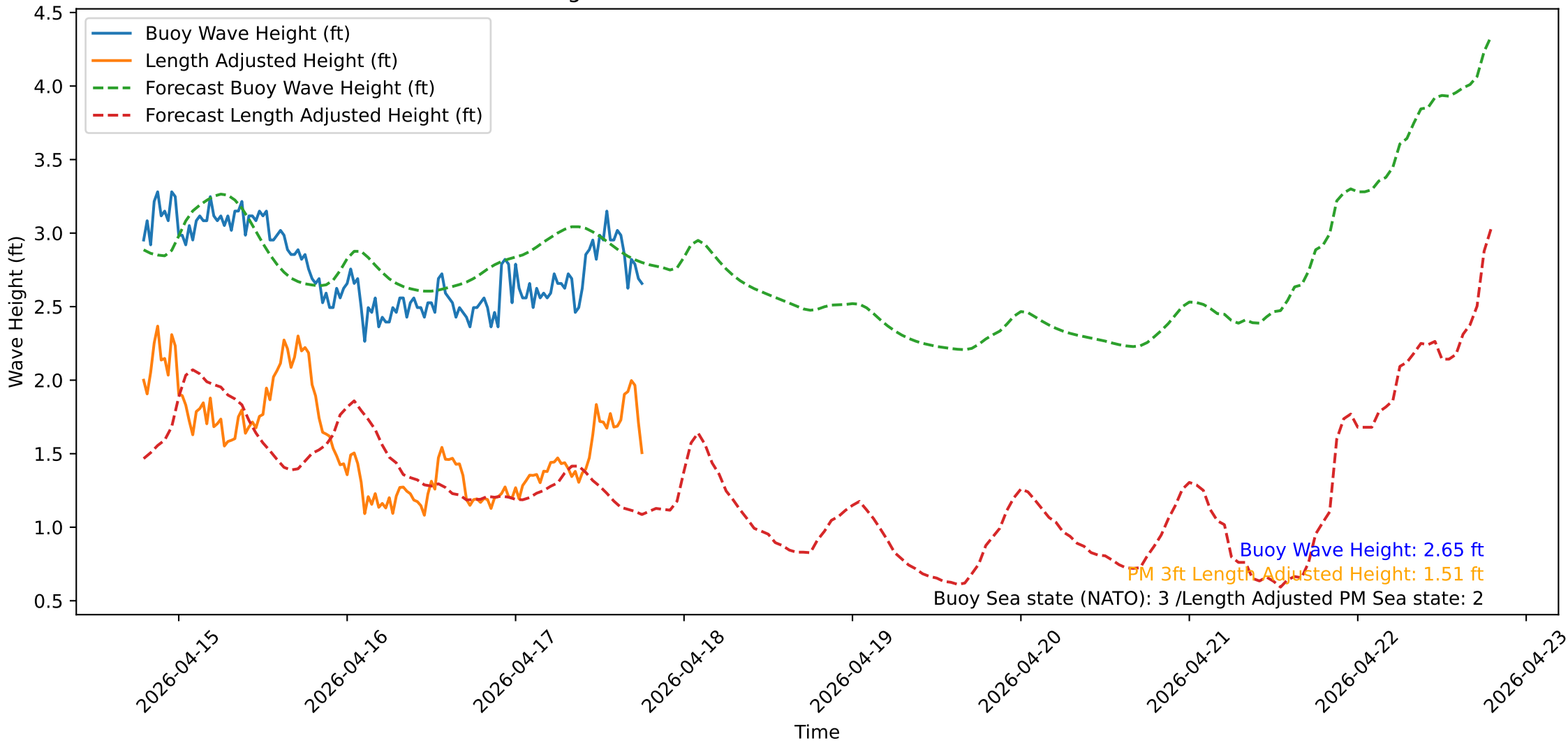
Wave Heights over Time for Red Beach at 2026-04-17 18:50:52
