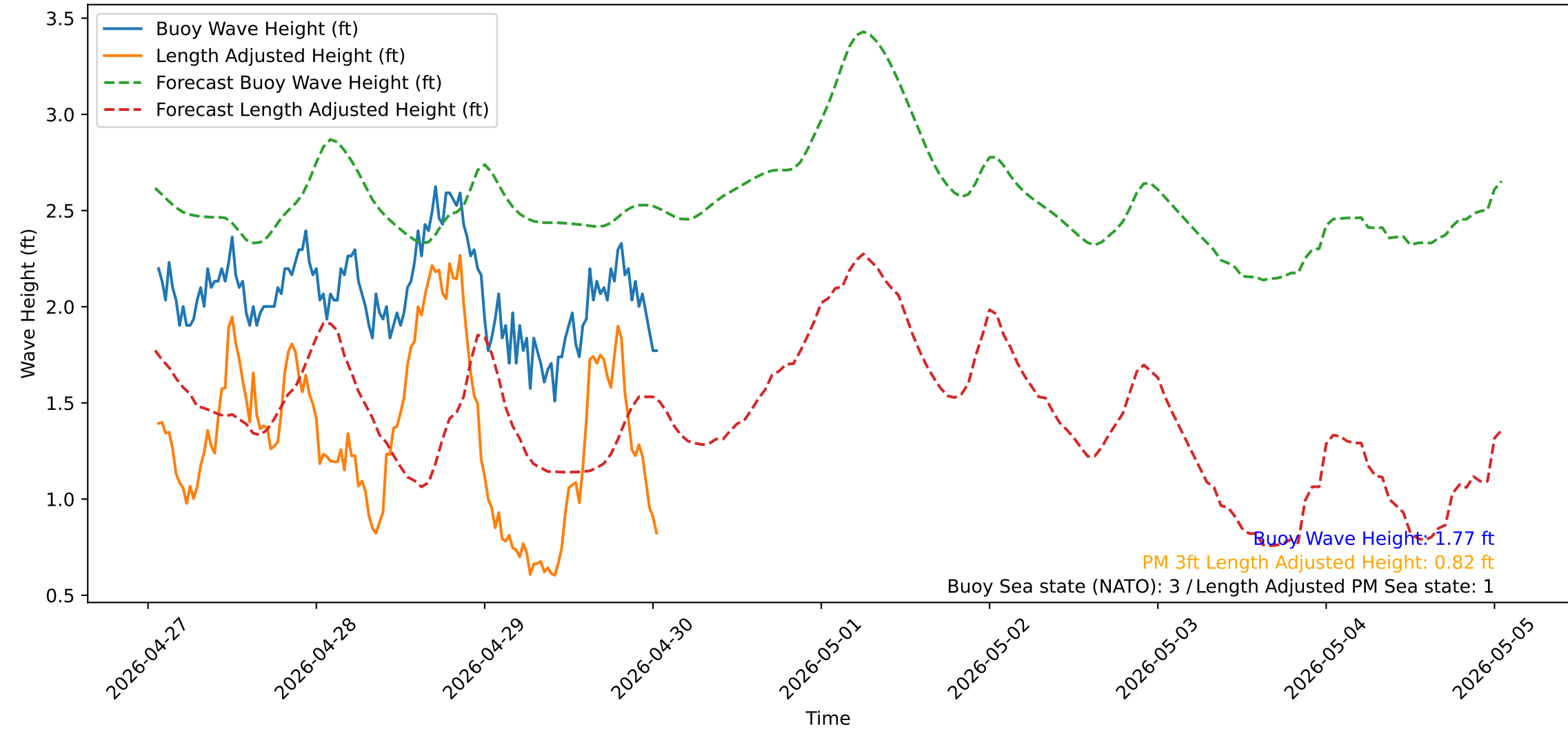
Wave Heights over Time for Red Beach at 2026-04-30 01:10:49
