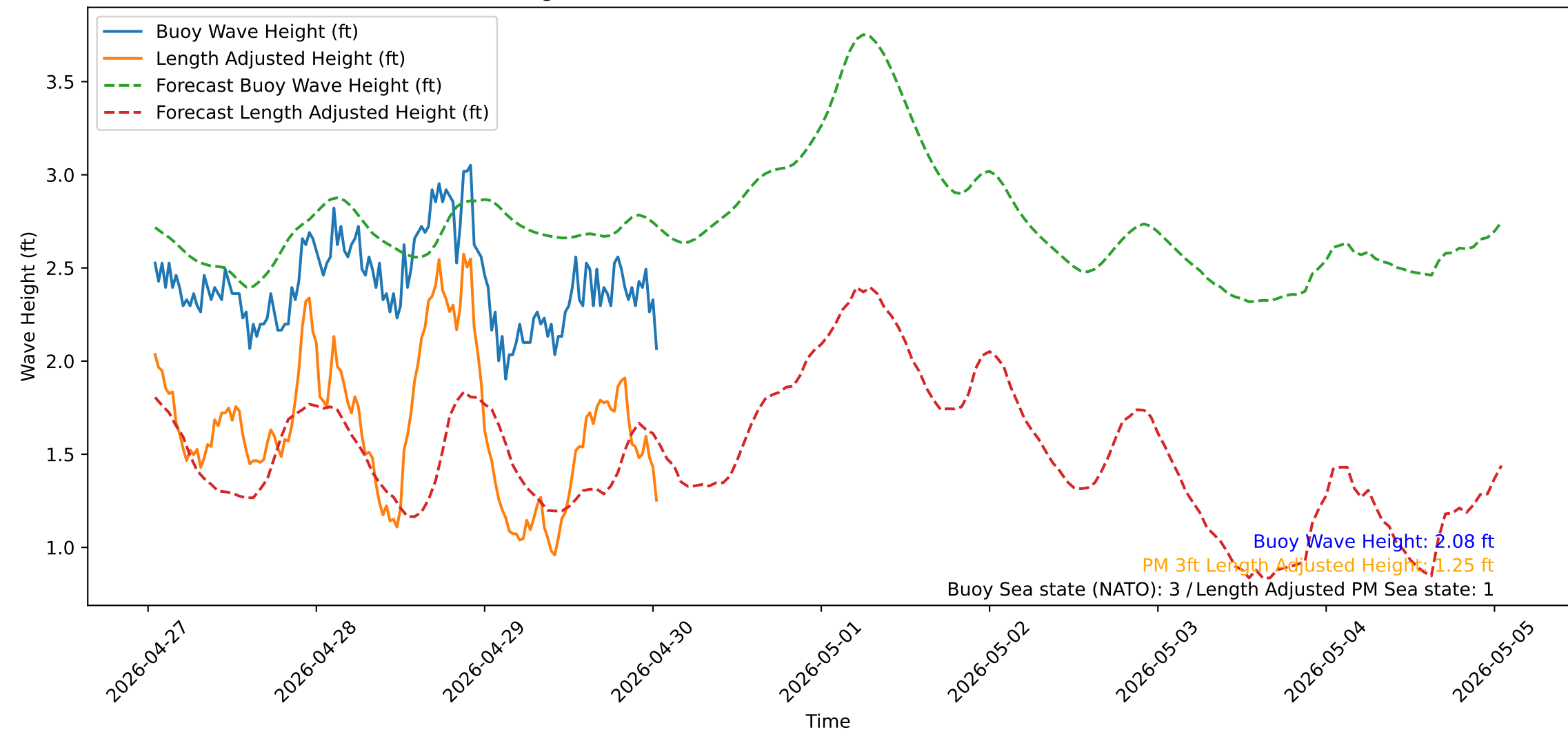
Wave Heights over Time for Oceanside Harbor at 2026-04-30 01:10:30
