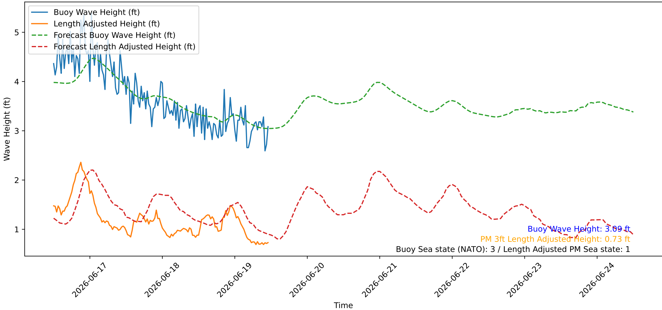
Wave Heights over Time for Red Beach at 2026-06-19 11:50:47
