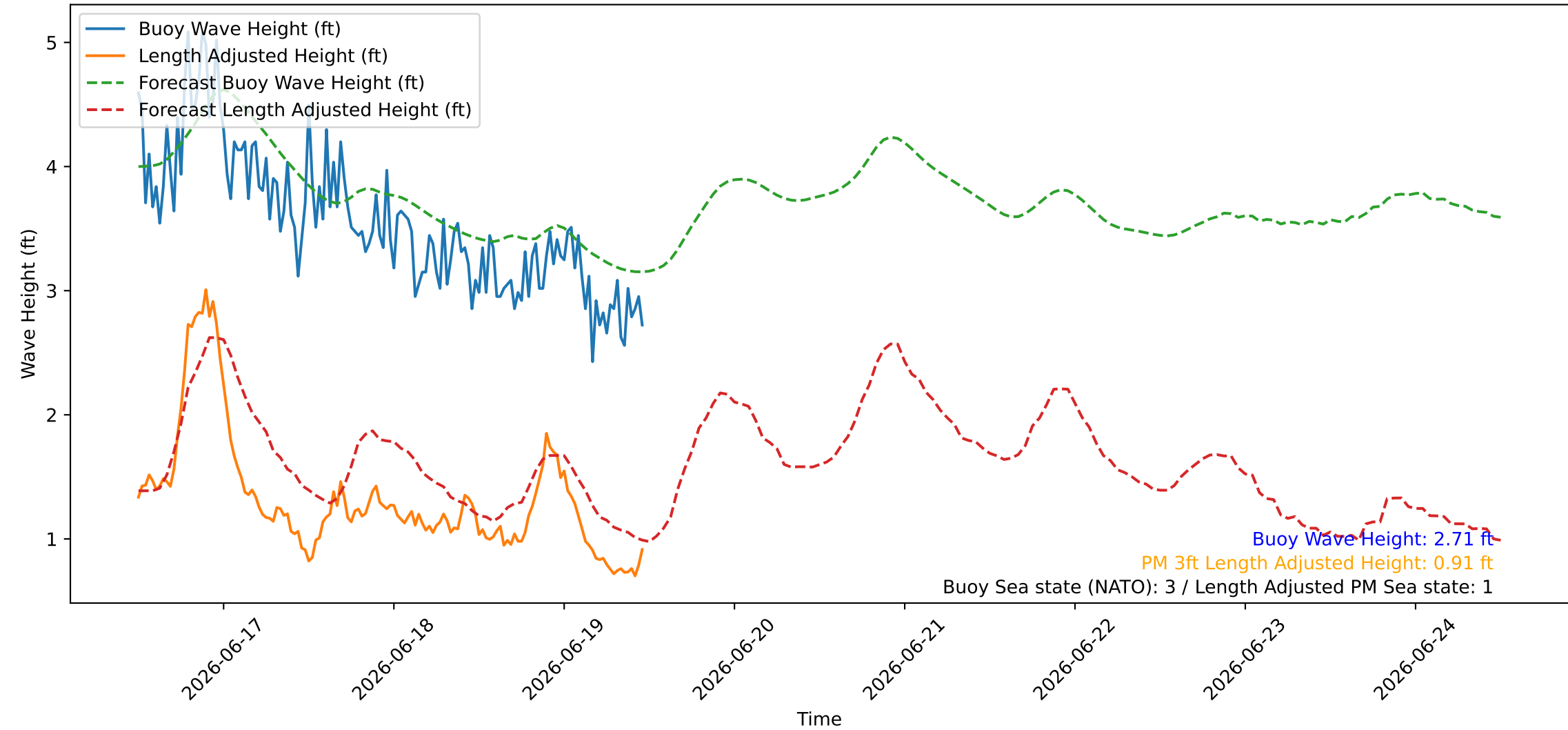
Wave Heights over Time for Green Beach at 2026-06-19 11:51:10
