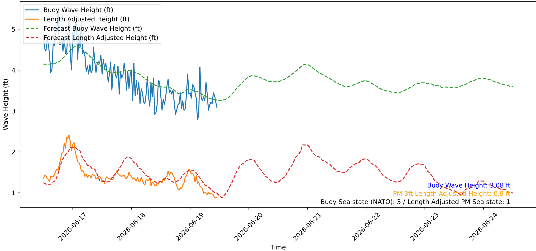
Wave Heights over Time for Oceanside Harbor at 2026-06-19 11:50:26
