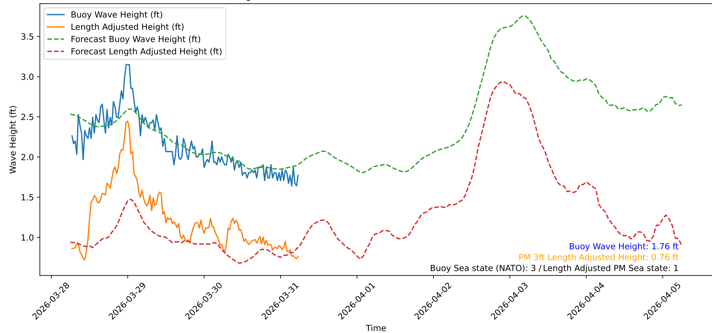
Wave Heights over Time for Oceanside Harbor at 2026-03-31 06:20:31
