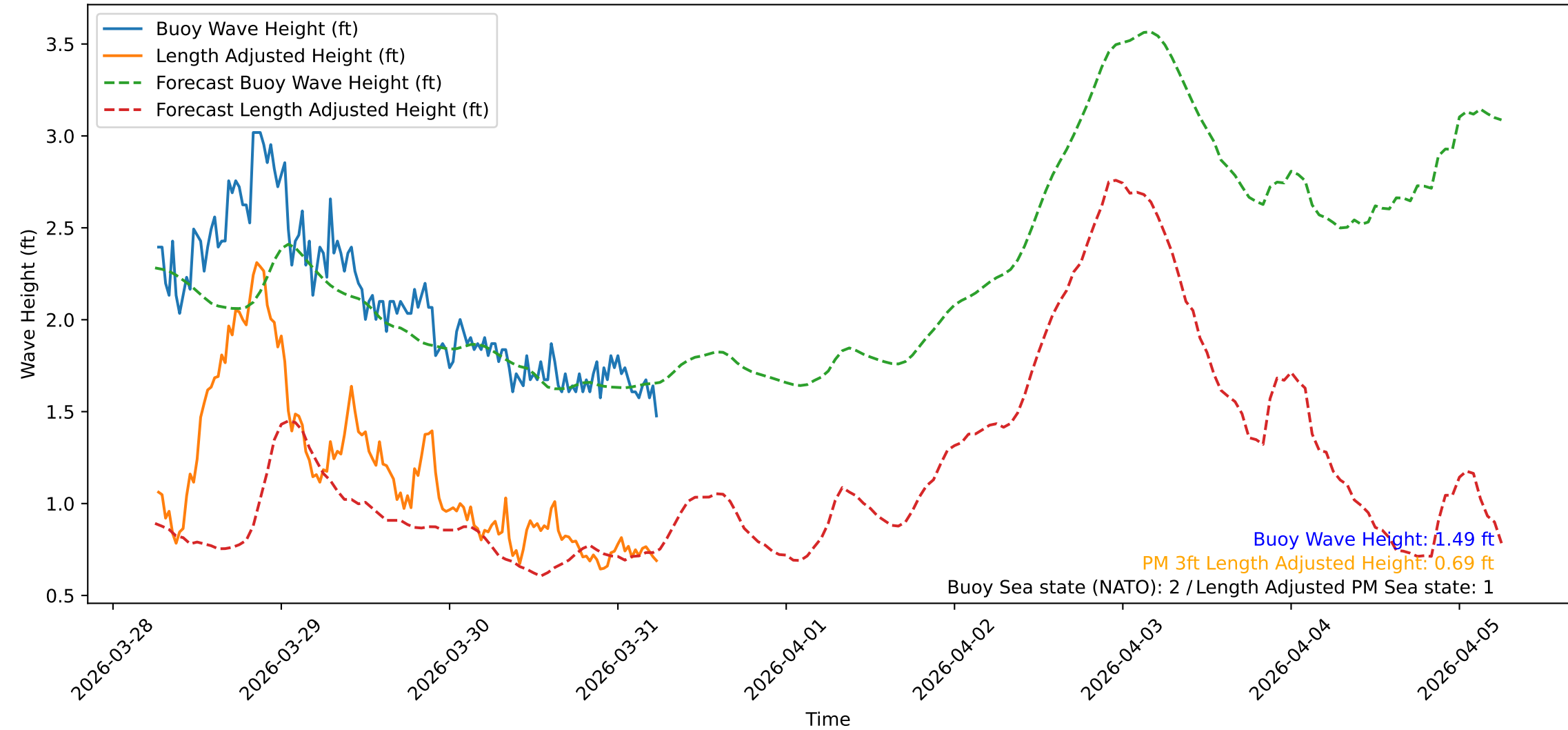
Wave Heights over Time for Red Beach at 2026-03-31 06:20:47
