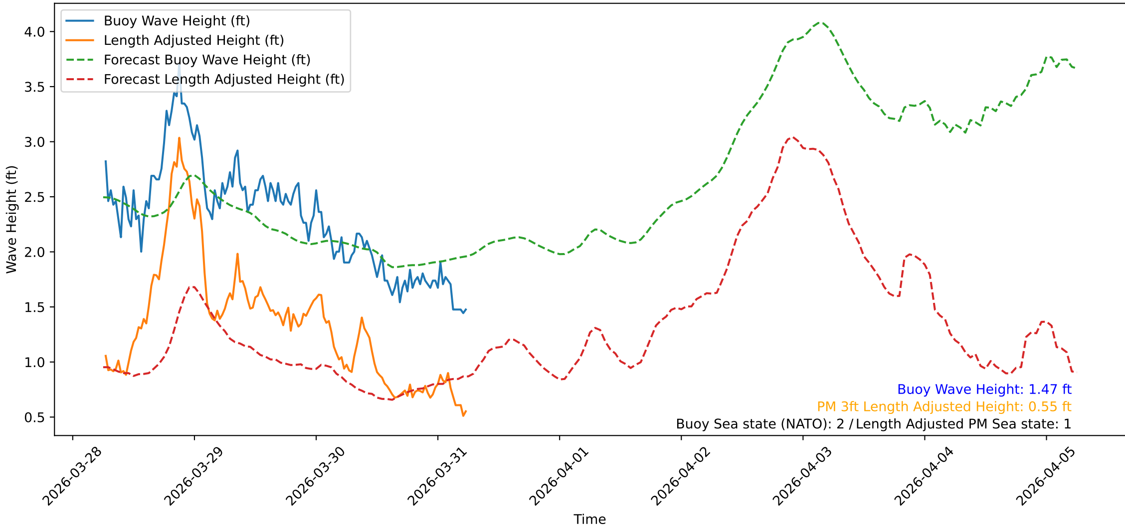
Wave Heights over Time for Green Beach at 2026-03-31 06:21:09
