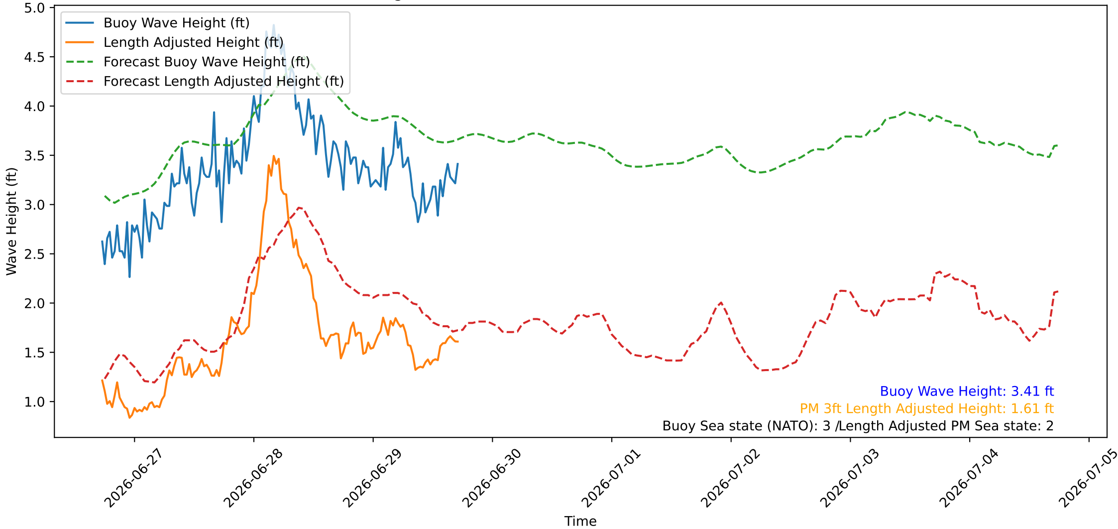
Wave Heights over Time for Green Beach at 2026-06-29 17:41:09
