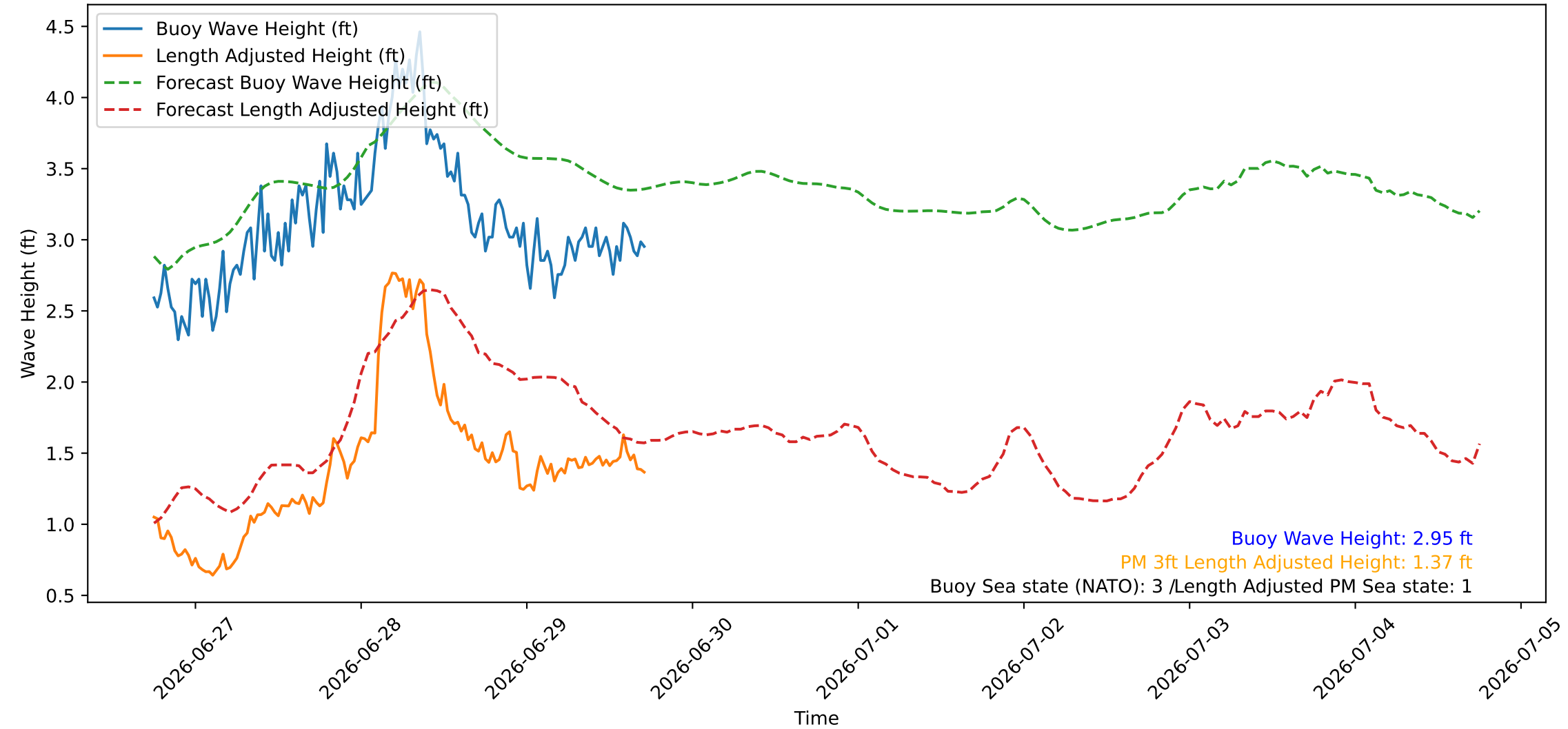
Wave Heights over Time for Red Beach at 2026-06-29 17:40:46
