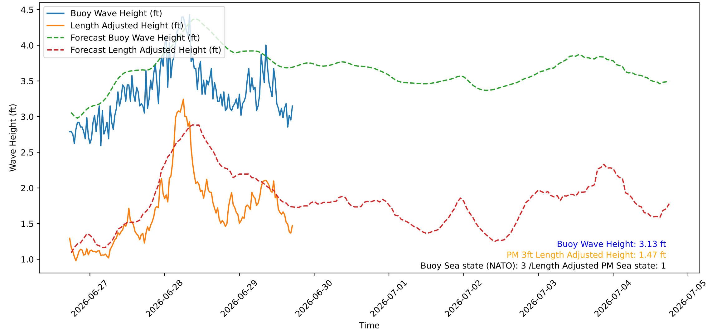
Wave Heights over Time for Oceanside Harbor at 2026-06-29 17:40:26
