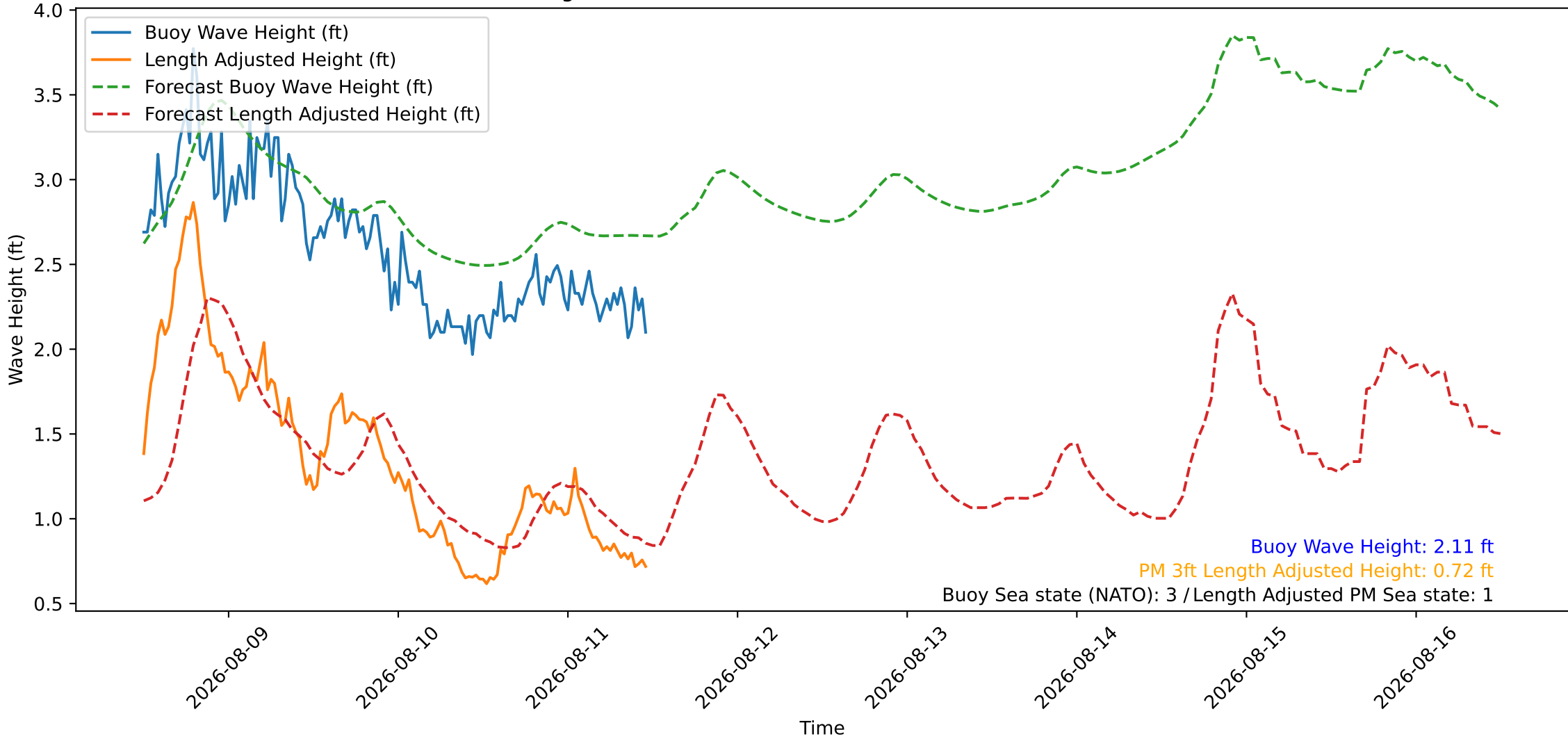
Wave Heights over Time for Green Beach at 2026-08-11 11:51:08
