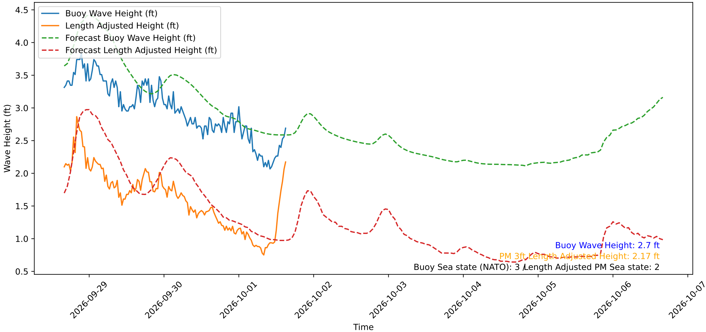
Wave Heights over Time for Red Beach at 2026-10-01 15:50:51
