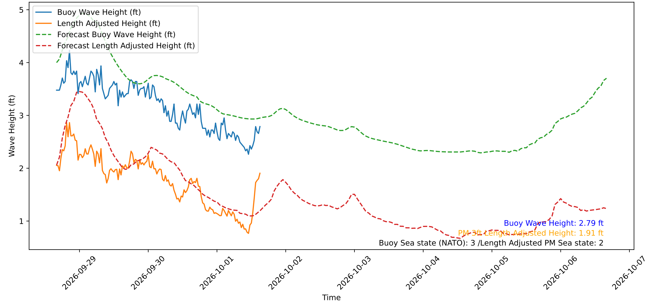
Wave Heights over Time for Oceanside Harbor at 2026-10-01 15:50:30
