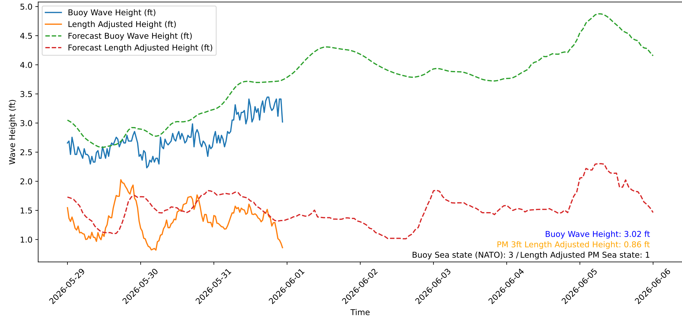
Wave Heights over Time for Red Beach at 2026-05-31 23:30:44
