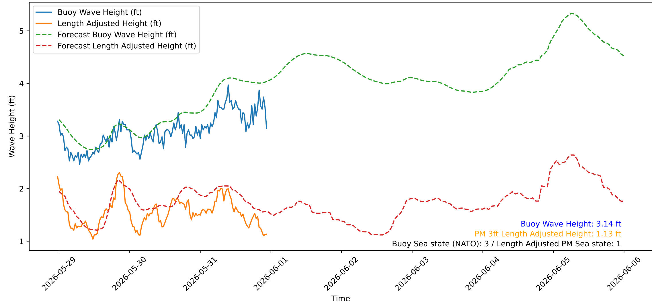
Wave Heights over Time for Green Beach at 2026-05-31 23:31:07
