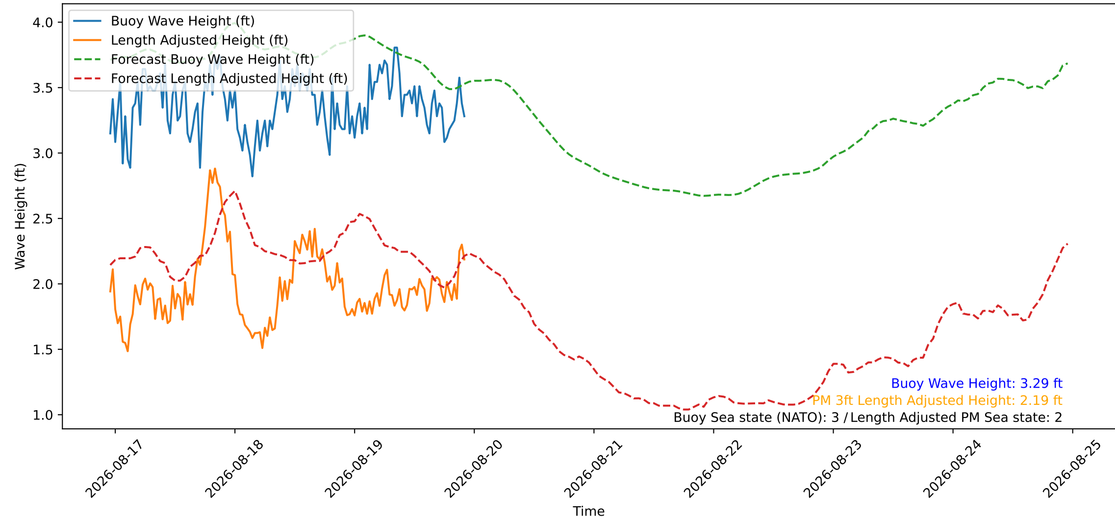
Wave Heights over Time for Oceanside Harbor at 2026-08-19 22:50:26
