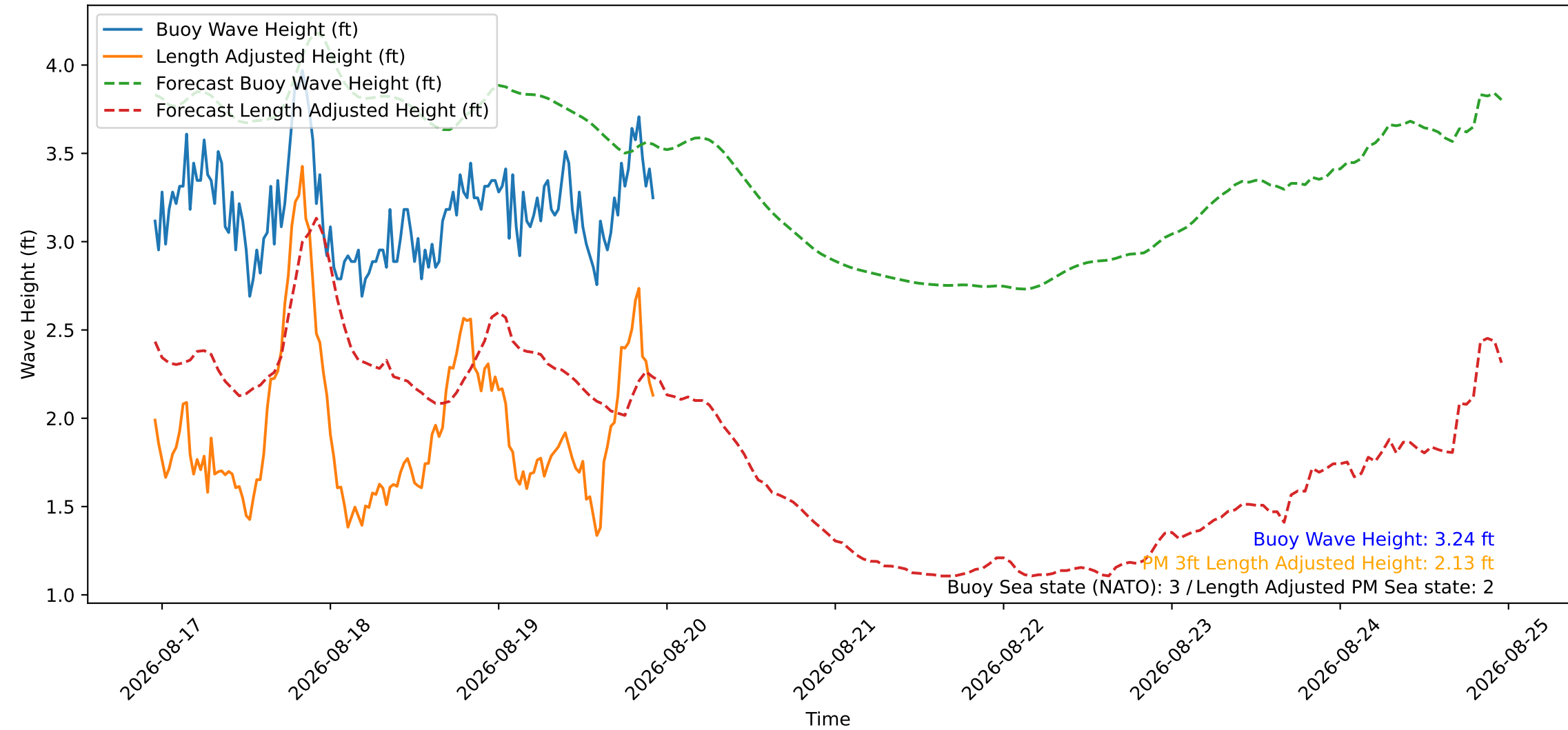
Wave Heights over Time for Green Beach at 2026-08-19 22:51:10
