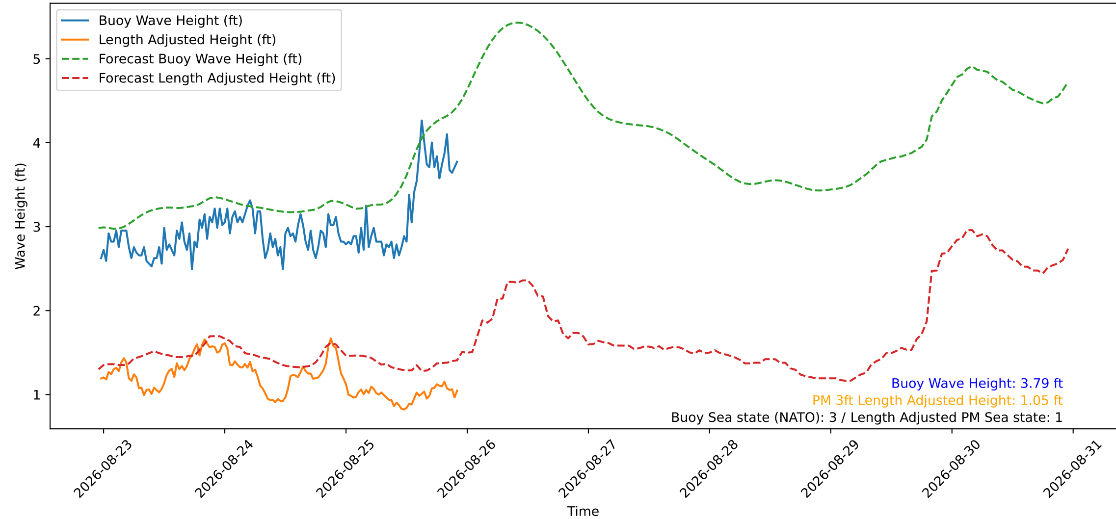
Wave Heights over Time for Green Beach at 2026-08-25 23:01:11
