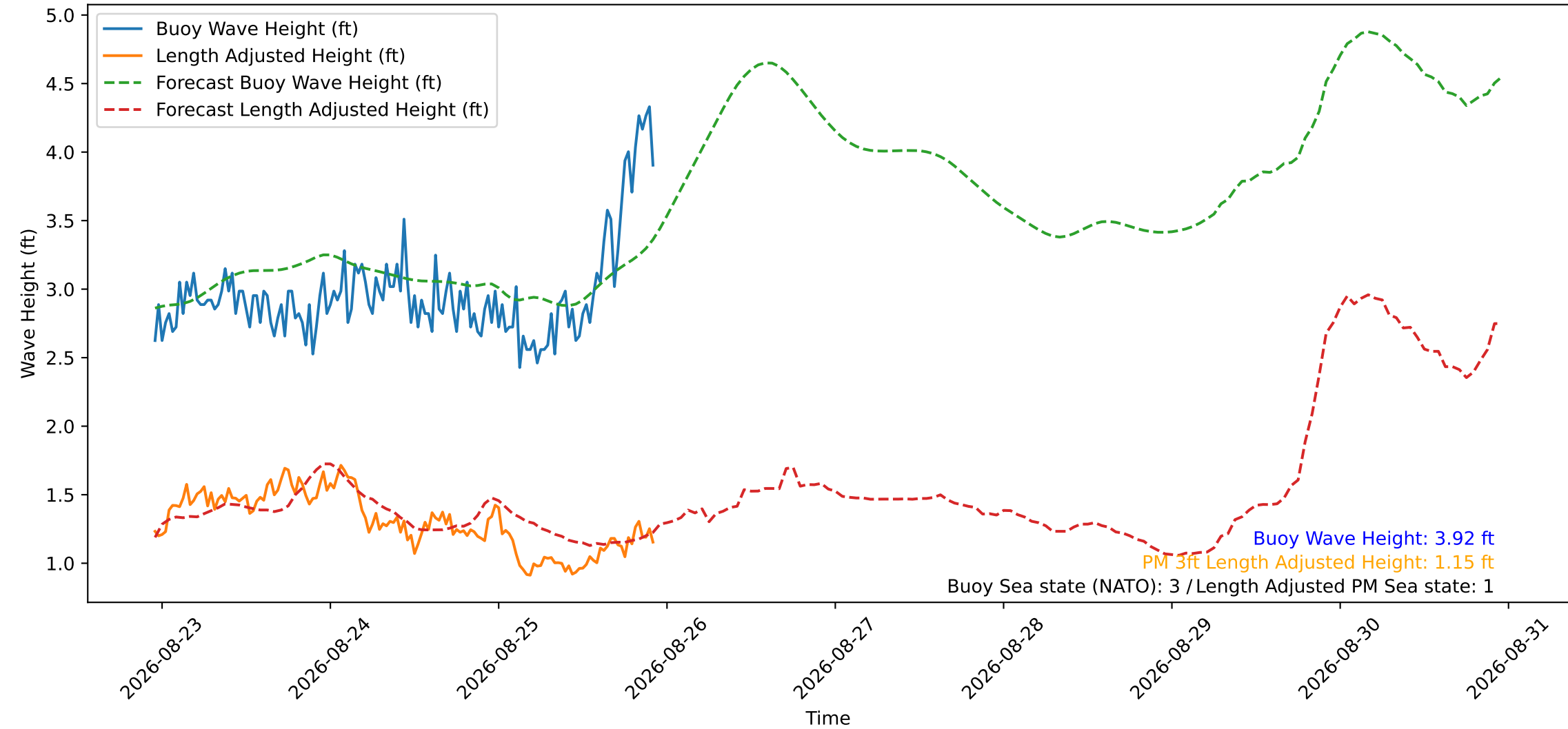
Wave Heights over Time for Oceanside Harbor at 2026-08-25 23:00:29
