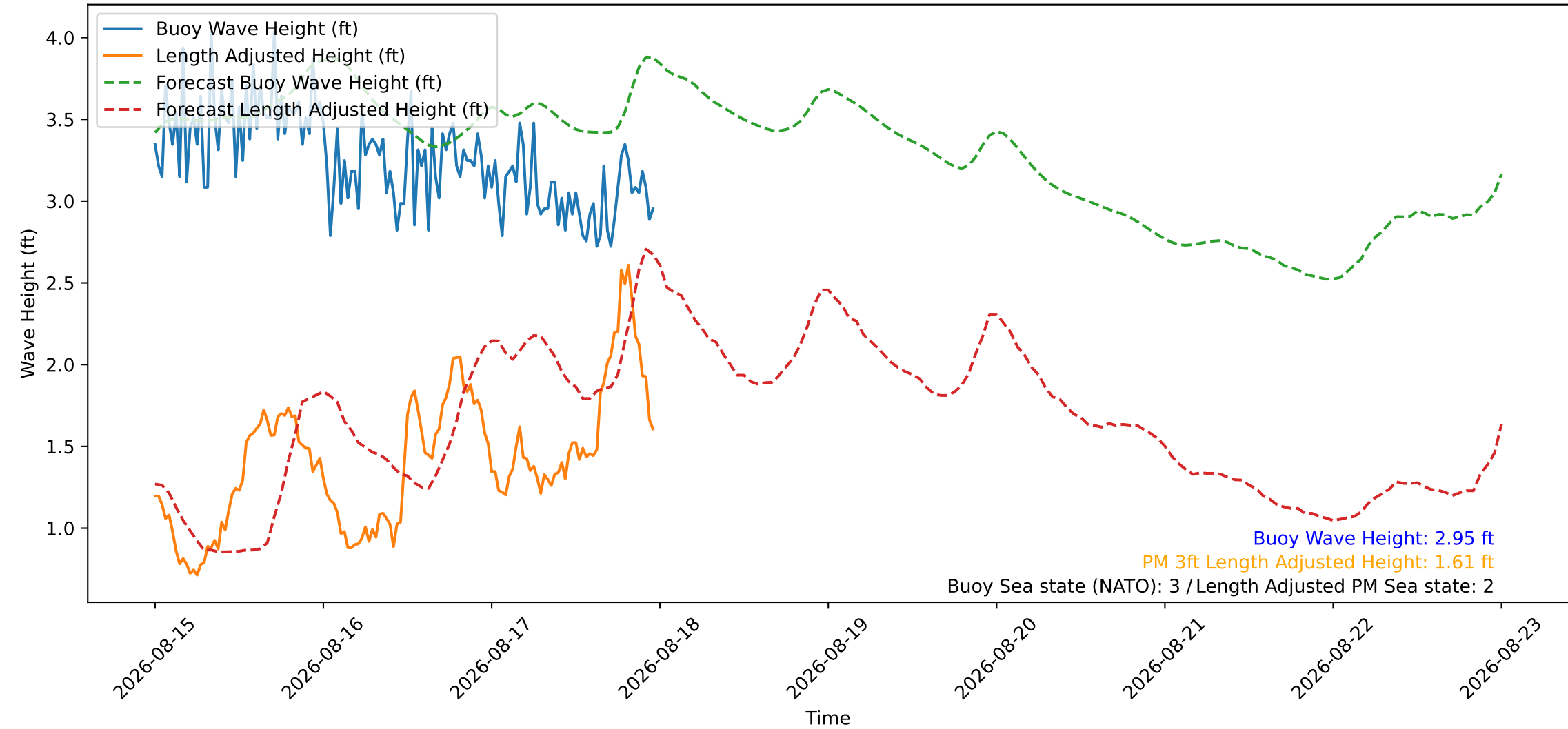
Wave Heights over Time for Red Beach at 2026-08-17 23:50:47
