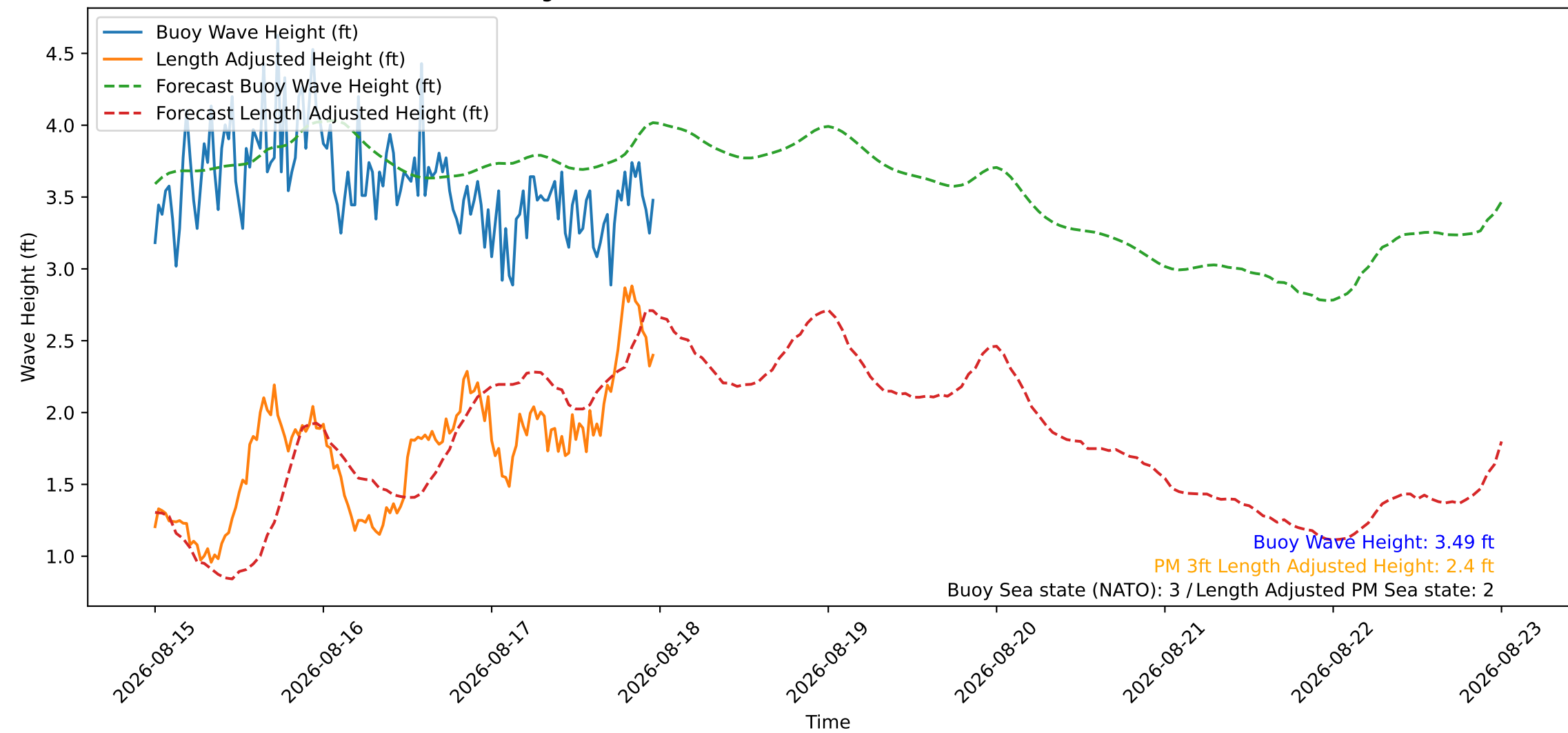
Wave Heights over Time for Oceanside Harbor at 2026-08-17 23:50:27
