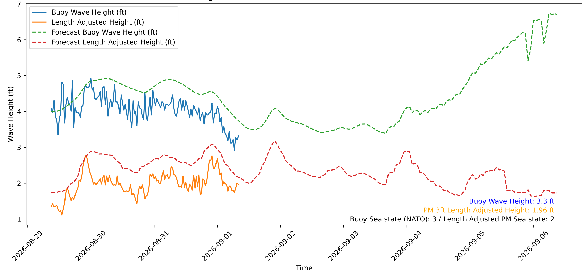
Wave Heights over Time for Green Beach at 2026-09-01 08:41:12
