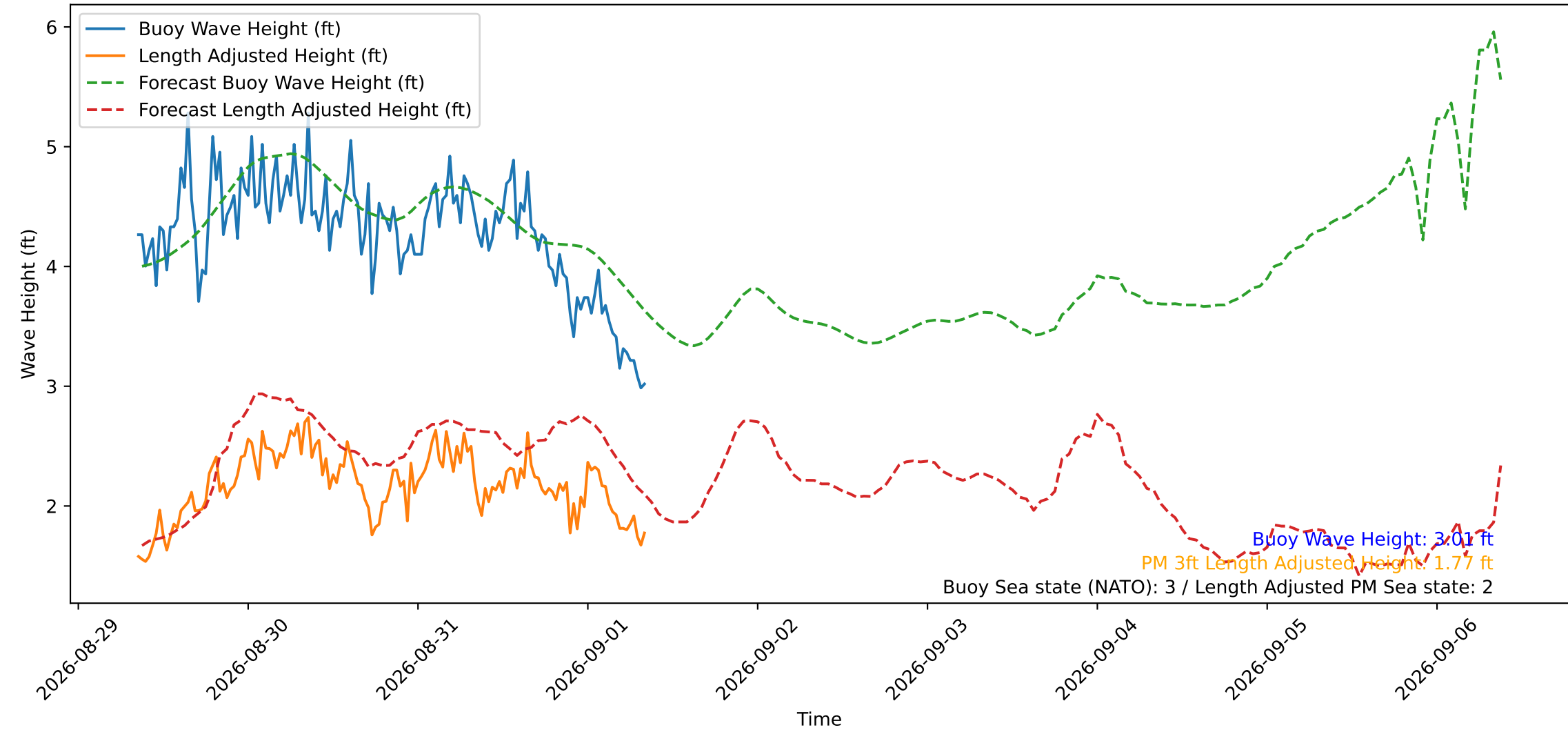
Wave Heights over Time for Oceanside Harbor at 2026-09-01 08:40:29
