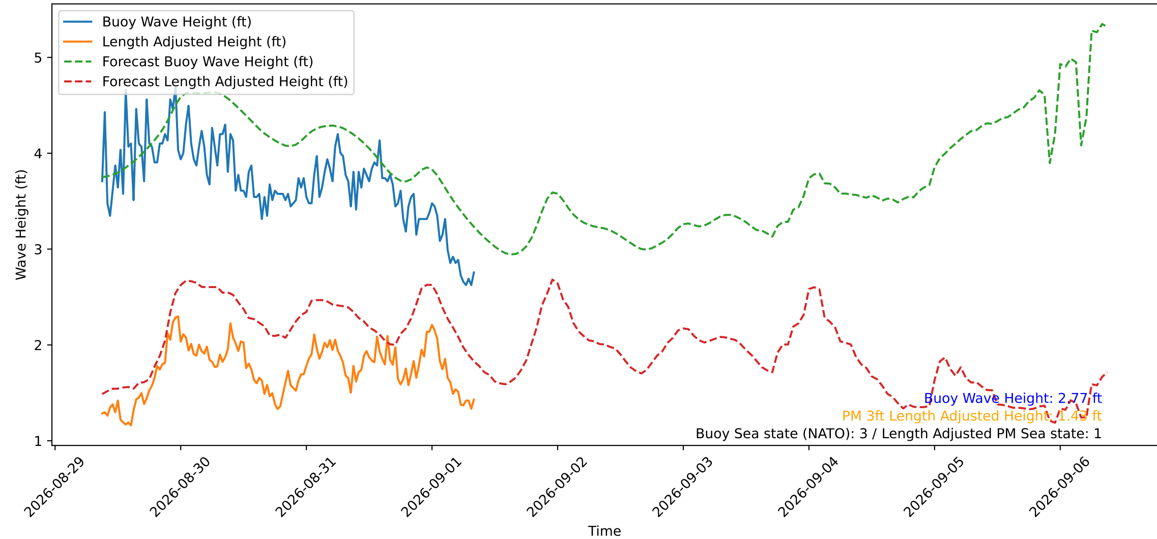
Wave Heights over Time for Red Beach at 2026-09-01 08:40:49
