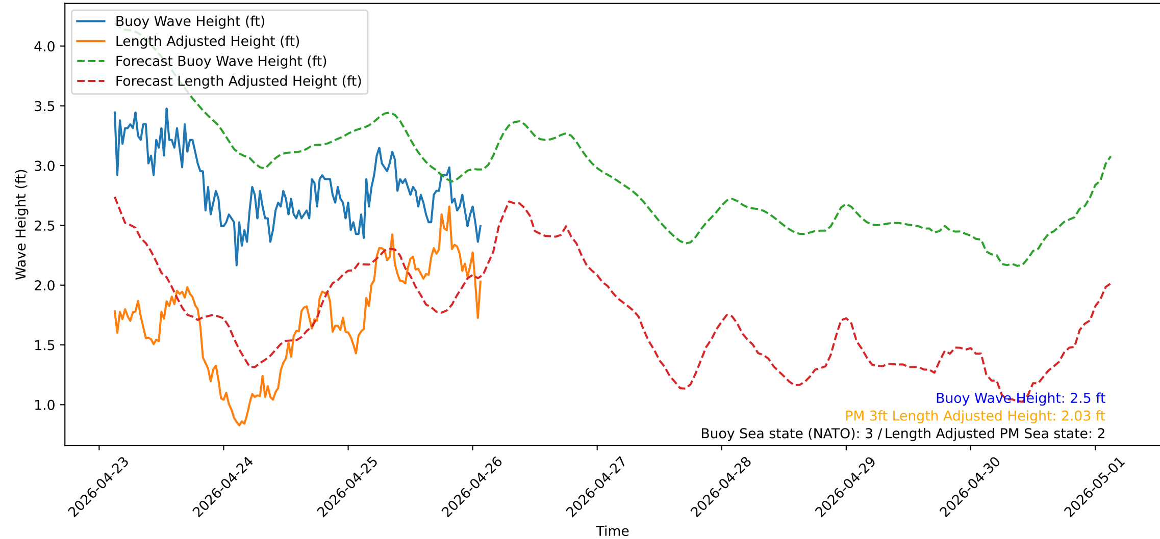
Wave Heights over Time for Red Beach at 2026-04-26 02:50:51
