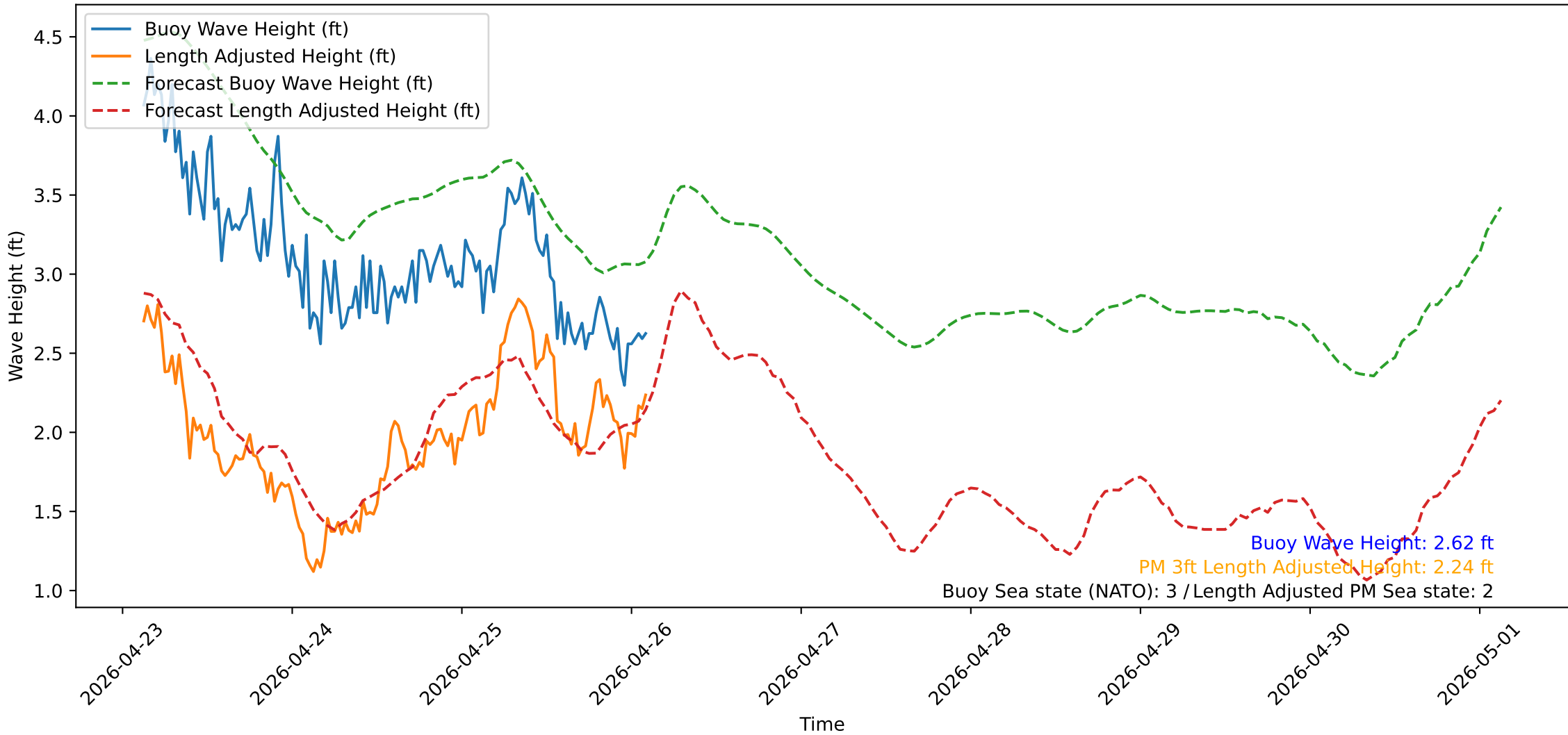
Wave Heights over Time for Oceanside Harbor at 2026-04-26 02:50:30
