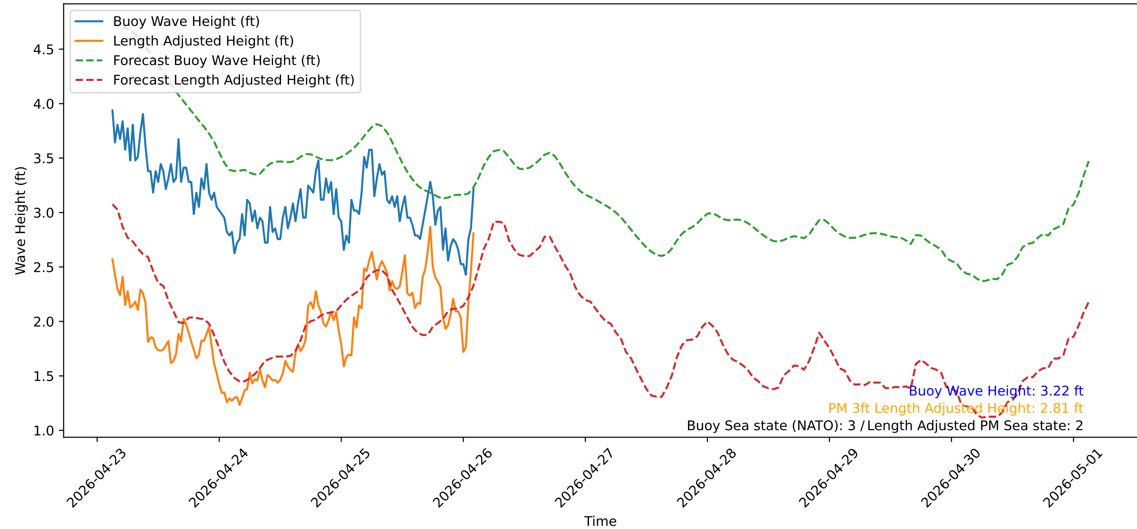
Wave Heights over Time for Green Beach at 2026-04-26 02:51:13
