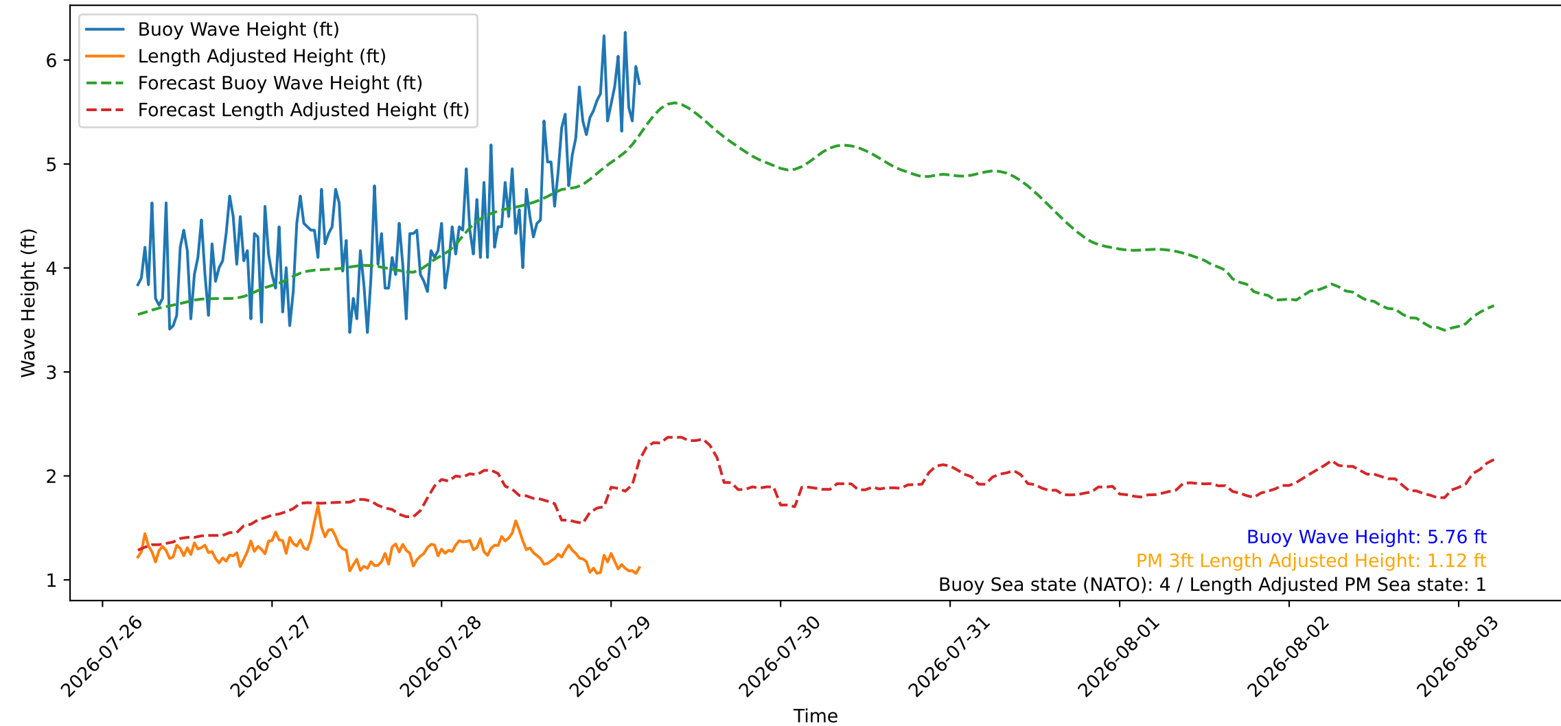
Wave Heights over Time for Green Beach at 2026-07-29 04:51:10
