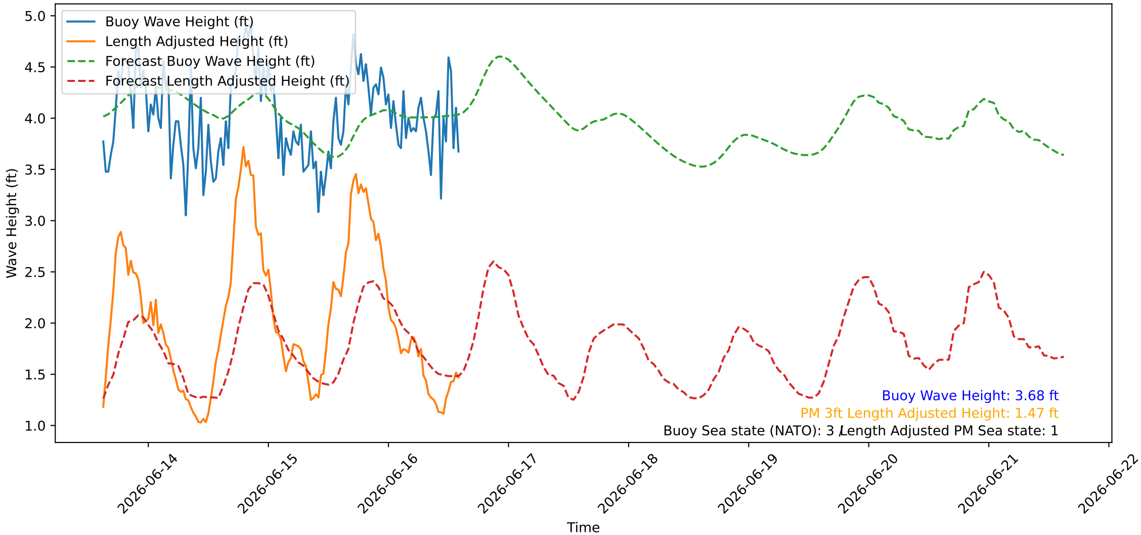
Wave Heights over Time for Green Beach at 2026-06-16 14:51:10
