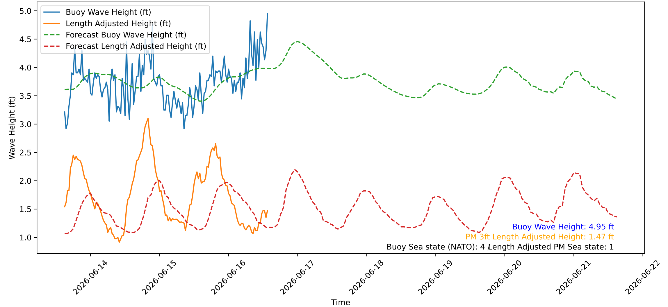
Wave Heights over Time for Red Beach at 2026-06-16 14:50:47
