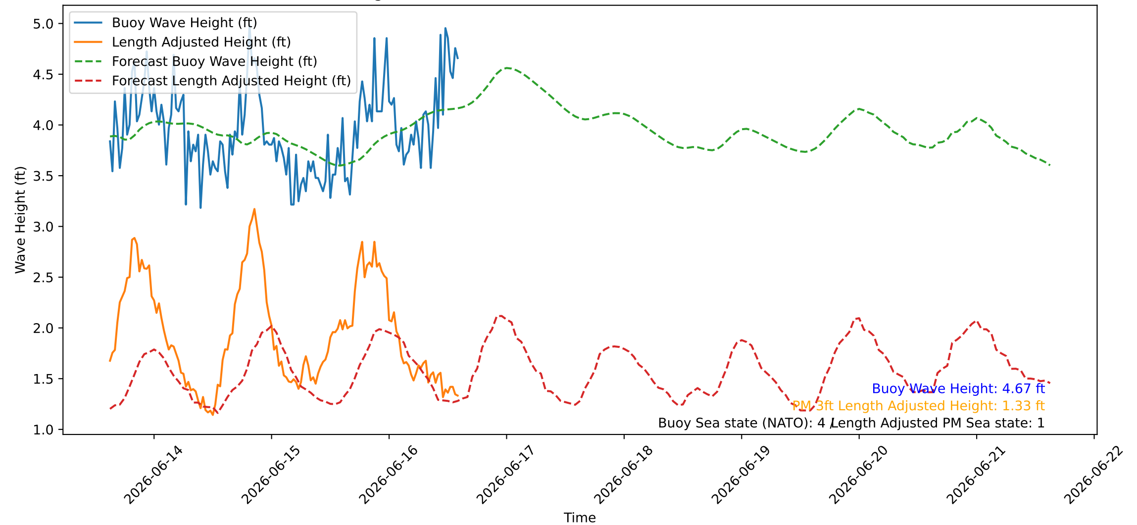
Wave Heights over Time for Oceanside Harbor at 2026-06-16 14:50:26
