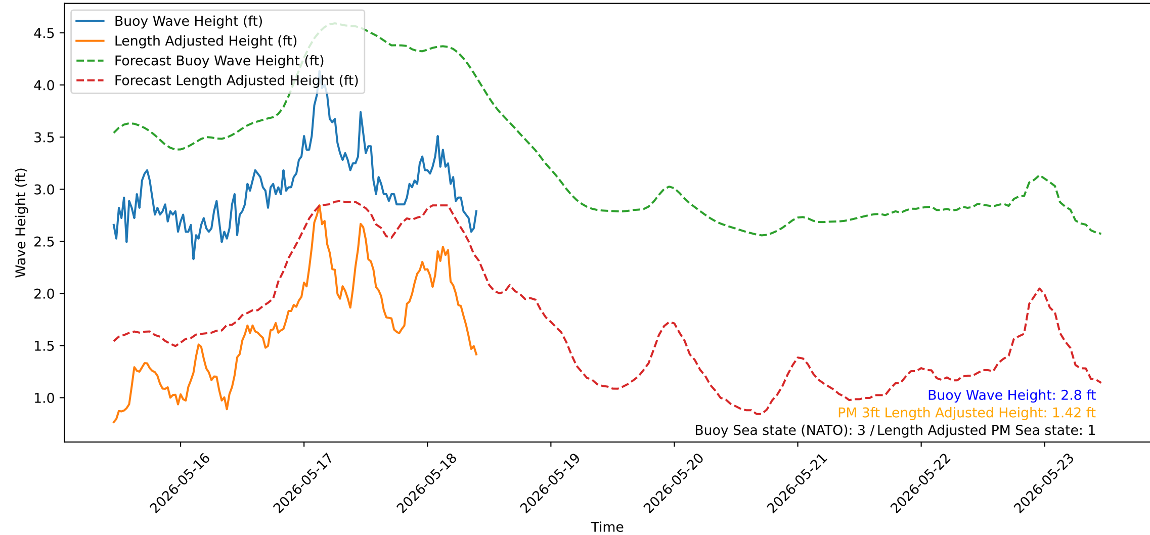
Wave Heights over Time for Red Beach at 2026-05-18 10:30:51
