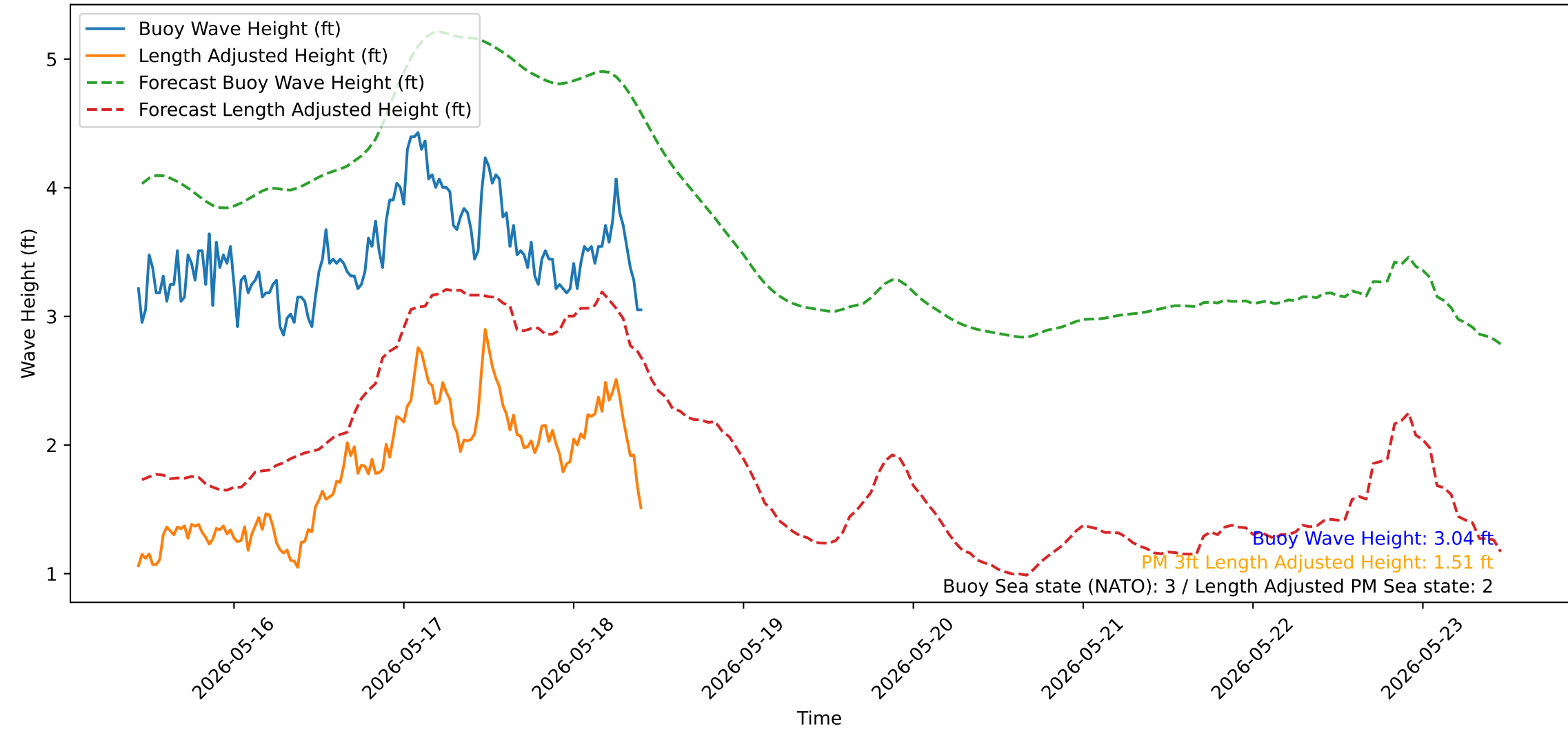
Wave Heights over Time for Green Beach at 2026-05-18 10:31:14
