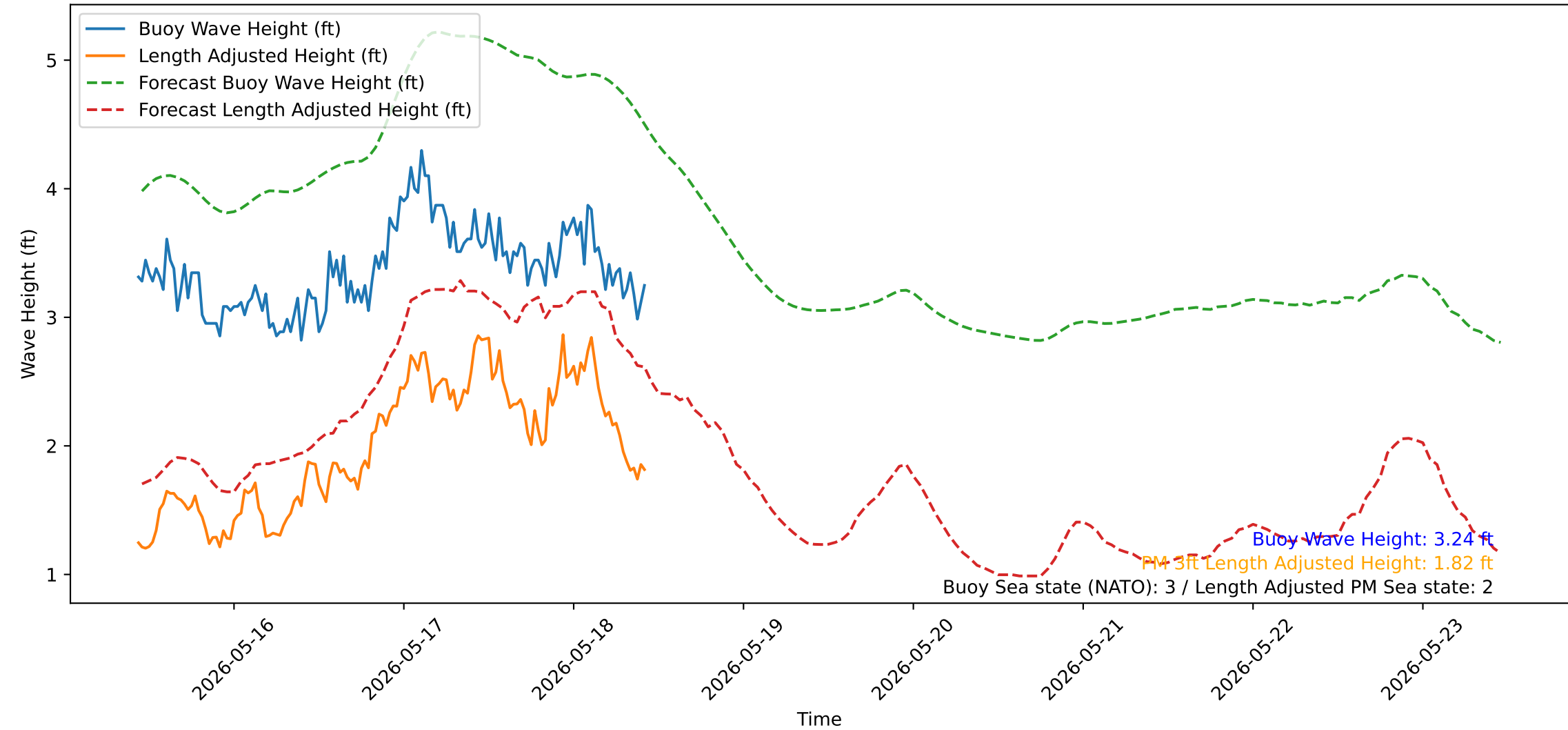
Wave Heights over Time for Oceanside Harbor at 2026-05-18 10:30:32
