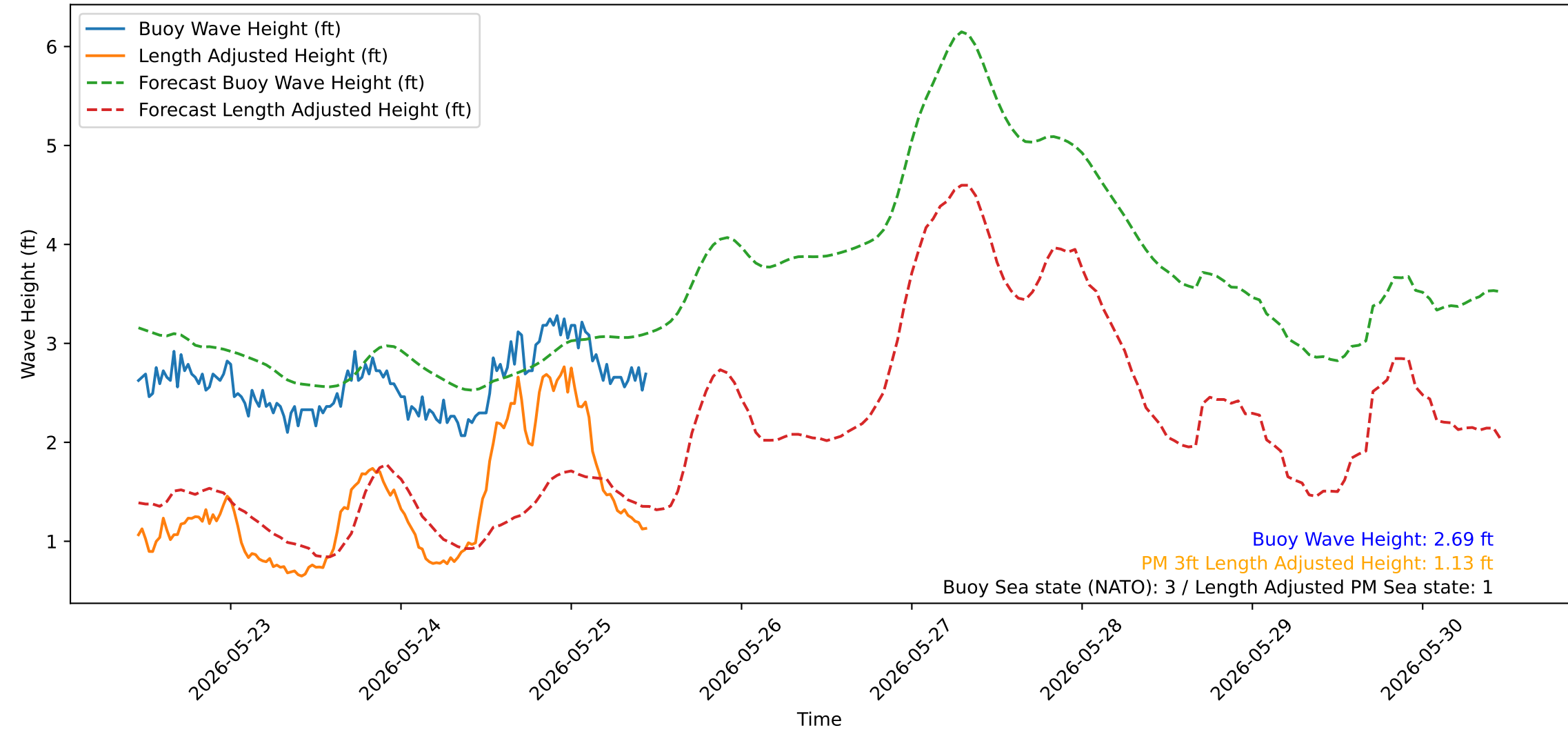
Wave Heights over Time for Green Beach at 2026-05-25 11:11:13
