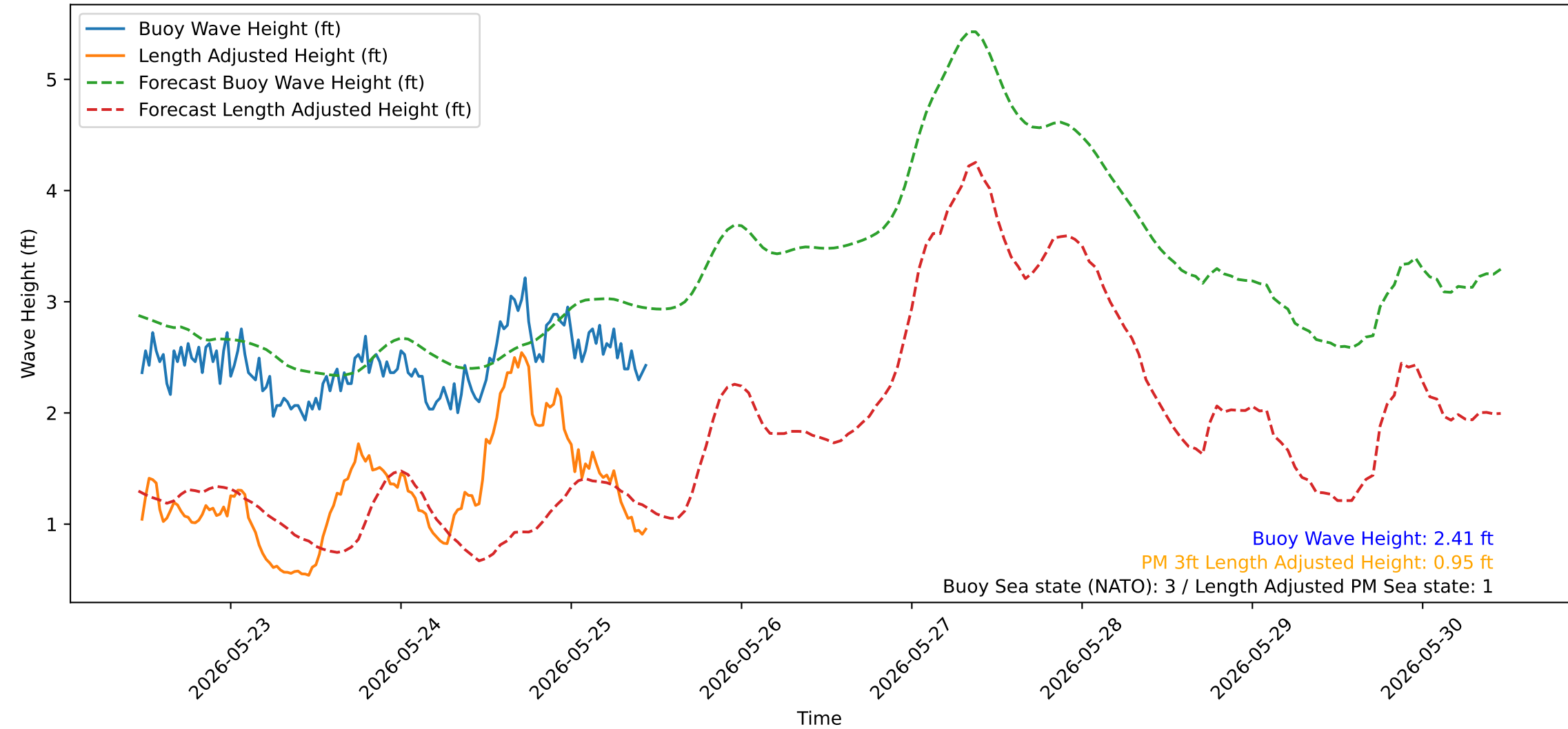
Wave Heights over Time for Red Beach at 2026-05-25 11:10:51
