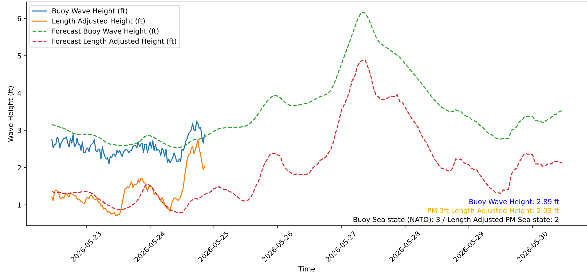
Wave Heights over Time for Oceanside Harbor at 2026-05-25 11:10:31
