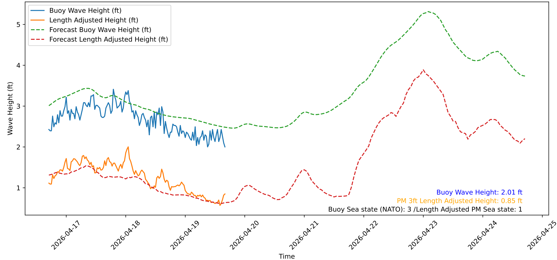
Wave Heights over Time for Oceanside Harbor at 2026-04-19 16:50:31
