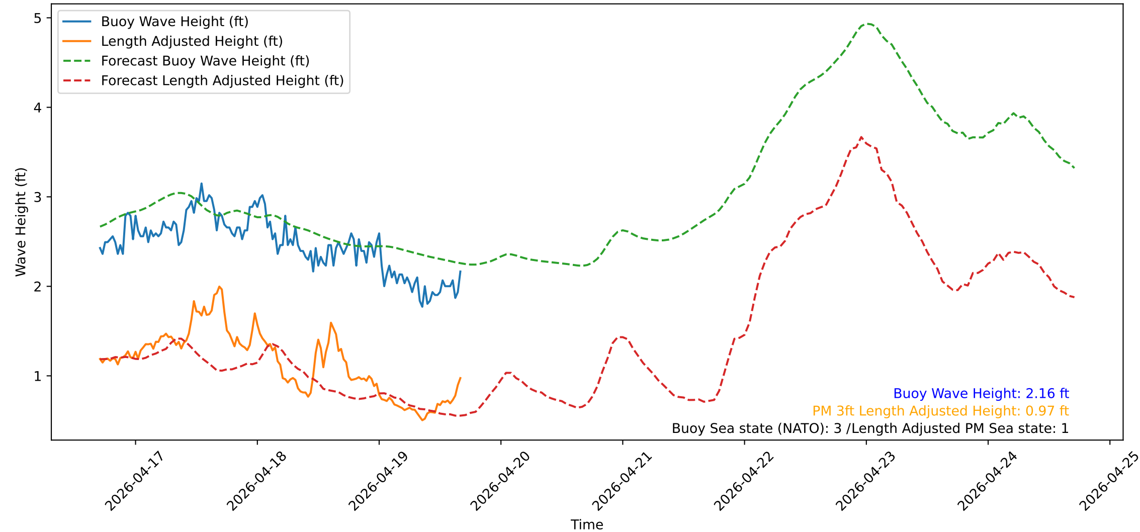
Wave Heights over Time for Red Beach at 2026-04-19 16:50:51
