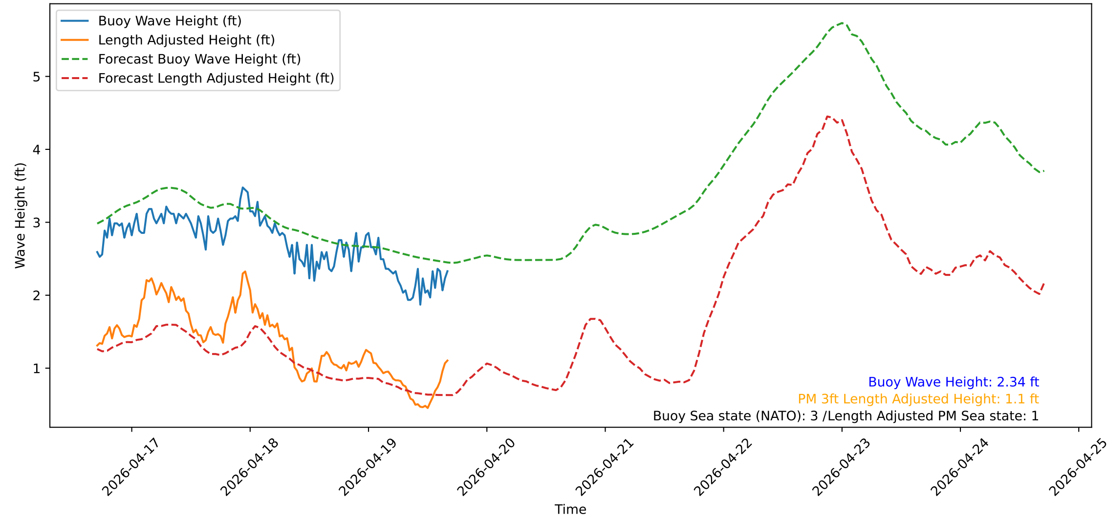
Wave Heights over Time for Green Beach at 2026-04-19 16:51:14
