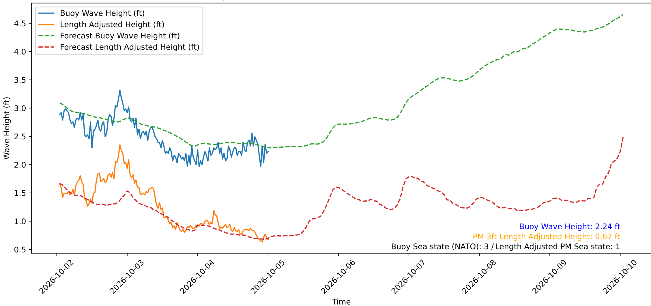
Wave Heights over Time for Oceanside Harbor at 2026-10-05 01:10:29
