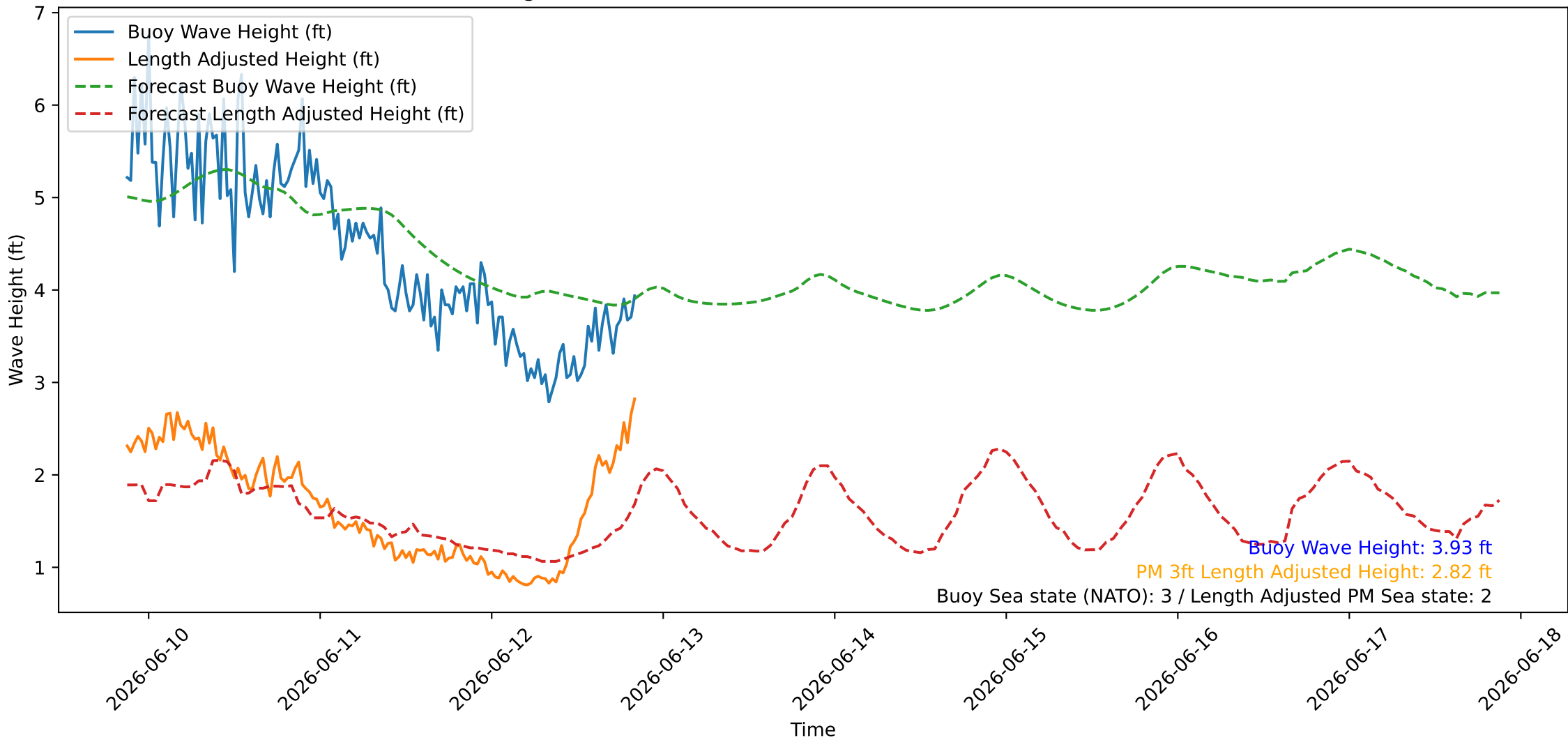
Wave Heights over Time for Oceanside Harbor at 2026-06-12 20:50:26
