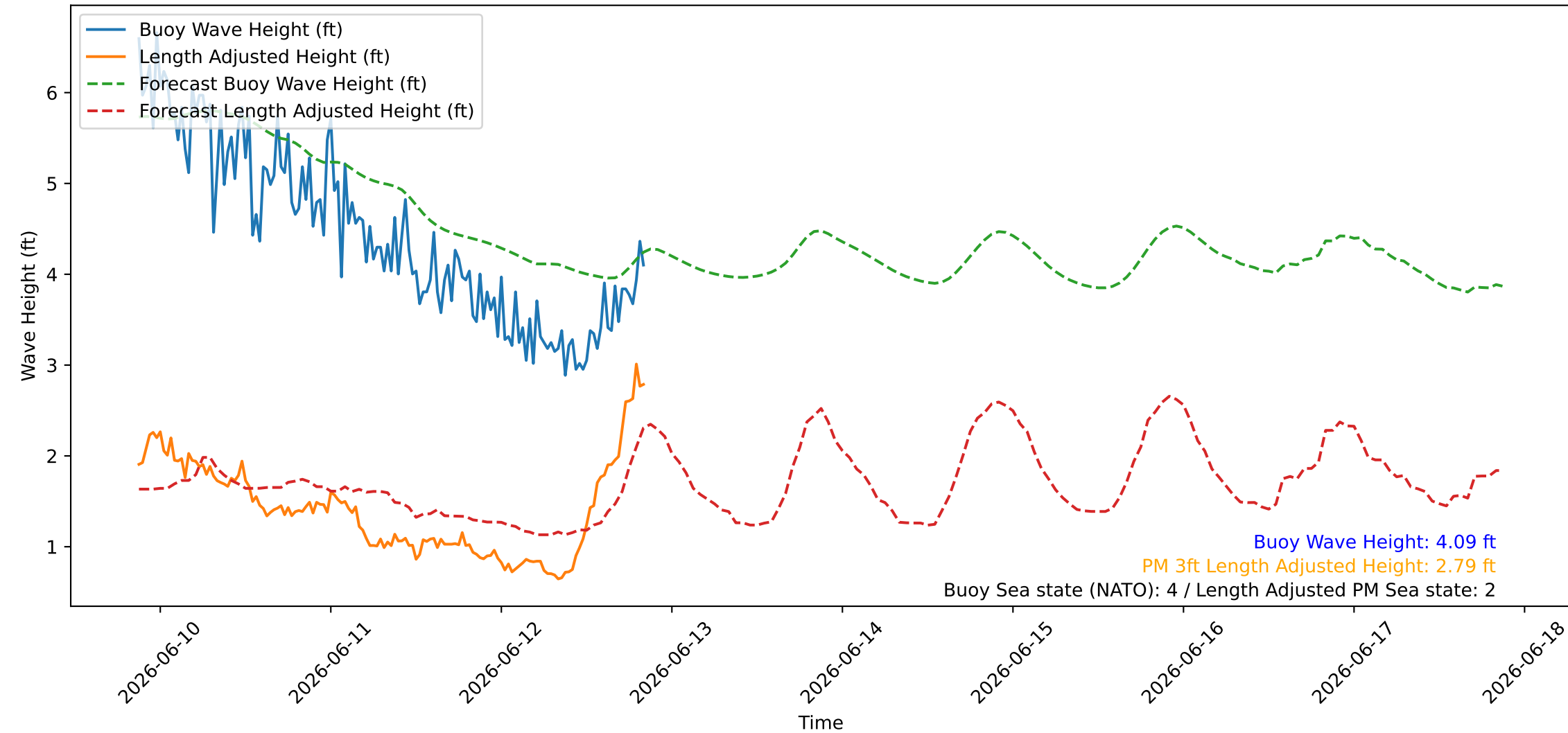
Wave Heights over Time for Green Beach at 2026-06-12 20:51:10
